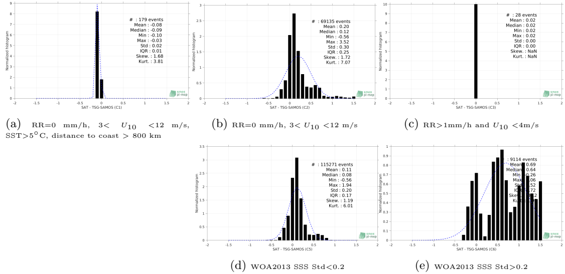
Figure 13: Normalized histogram of \Delta\text{SSS} (Aquarius-L4-IPRC-V5-MONTHLY - TSG-SAMOS) for 5 different subdatasets corresponding to: RR=0 mm/h, 3 < U_{10} < 12 m/s, SST > 5^{\circ}\text{C} , distance to coast > 800 km (a), RR=0 mm/h, 3 < U_{10} < 12 m/s (b), RR > 1\text{mm/h} and U_{10} < 4\text{m/s} (c), WOA2013 SSS Std < 0.2 (d), WOA2013 SSS Std > 0.2 (e).
