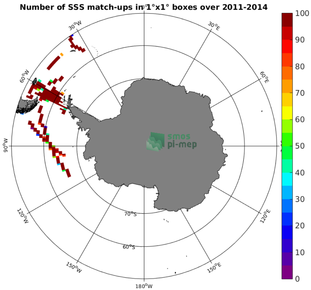
Figure 4: Number of SSS match-ups between TSG-SAMOS SSS and the Aquarius-L4-IPRC-V5-MONTHLY SSS product for the Southern Ocean Pi-MEP region over 1^\circ \times 1^\circ boxes and for the full satellite product period.
