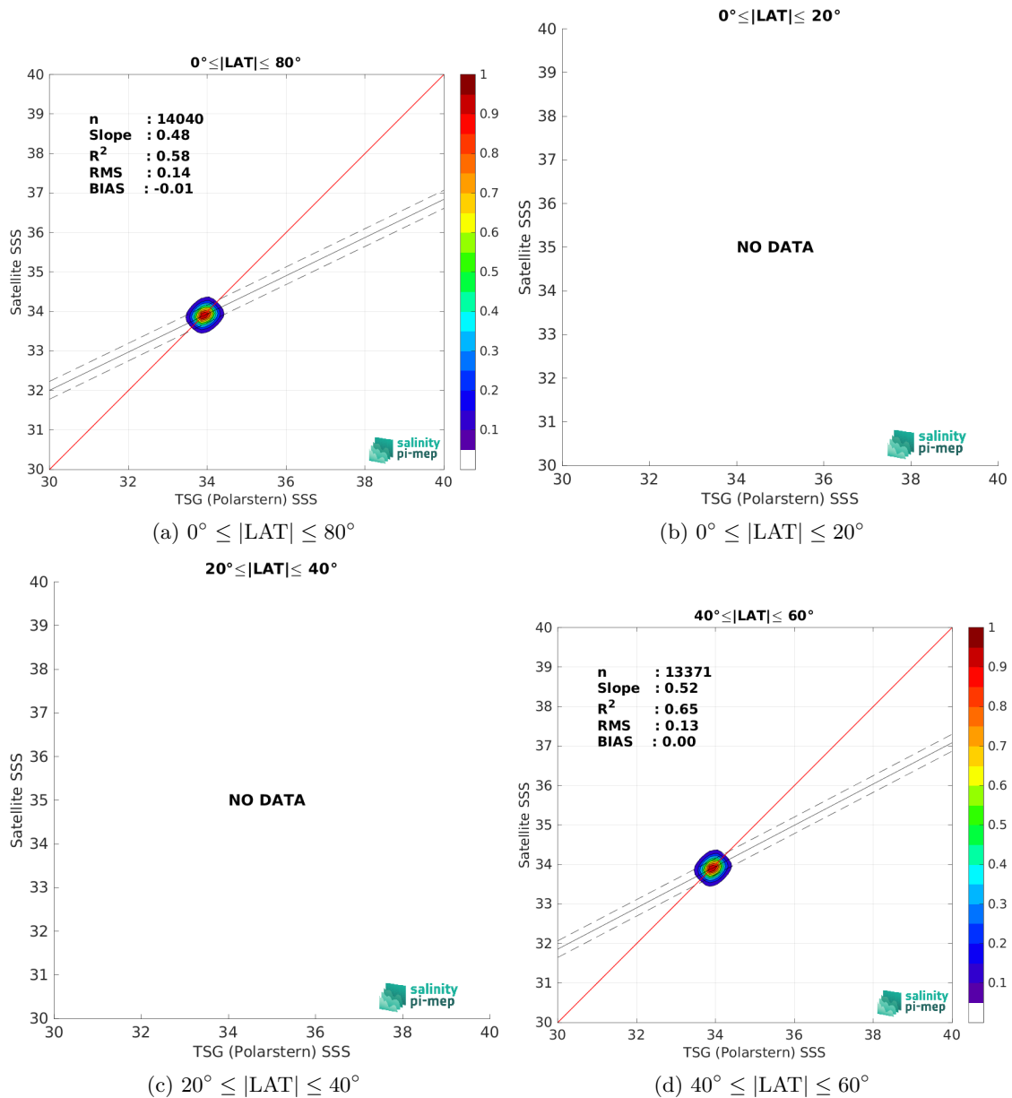
Figure 10: Contour maps of the concentration of Aquarius SSS L4 OI v5 - Monthly (IPRC) SSS (y-axis) versus TSG (Polarstern) SSS (x-axis) at match-up pairs for different latitude bands. For each plot, the red line shows x=y . The black thin and dashed lines indicate a linear fit through the data cloud and the \pm 95\% confidence levels, respectively. The number match-up pairs n , the slope and R^2 coefficient of the linear fit, the root mean square (RMS) and the mean bias between satellite and in situ data are indicated for each latitude band in each plots.
