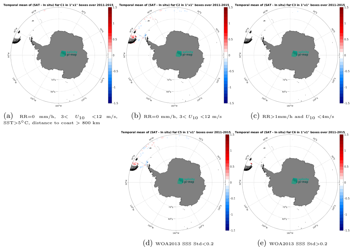
Figure 14: Temporal mean gridded over spatial boxes of size 1^\circ \times 1^\circ of \Delta SSS (Aquarius SSS L4 OI v5 - Monthly (IPRC) - TSG (Polarstern)) for 5 different subdatasets corresponding to:RR=0 mm/h, 3 < U_{10} < 12 m/s, SST >5^\circ\text{C} , distance to coast > 800 km (a), RR=0 mm/h, 3 < U_{10} < 12 m/s (b), RR >1 mm/h and U_{10} < 4 m/s (c), WOA2013 SSS Std <0.2 (d), WOA2013 SSS Std >0.2 (e).
