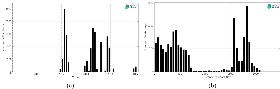
Figure 2: Number of match-ups between TSG (Polarstern) and Aquarius SSS L4 OI v5 - Monthly (IPRC) SSS as a function of time (a) and as function of the distance to coast (b) over the Southern Ocean Pi-MEP region and for the full satellite product period.
