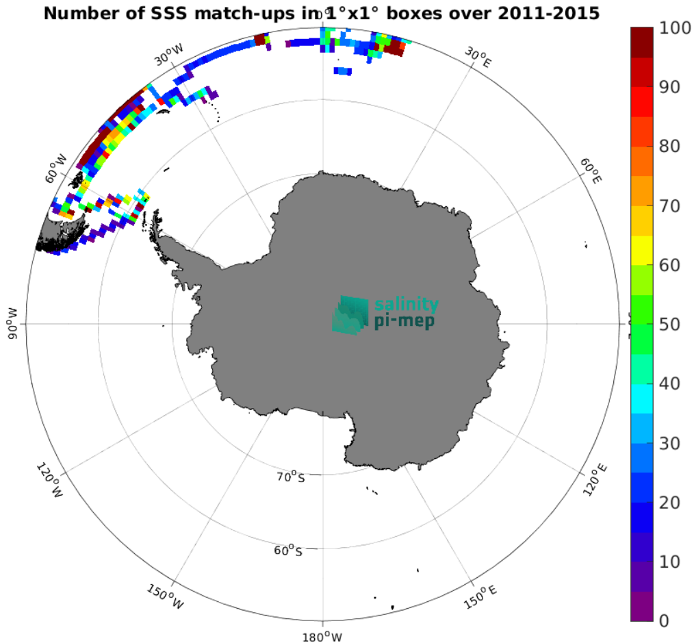
Figure 5: Number of SSS match-ups between TSG (Polarstern) SSS and the Aquarius SSS L4 OI v5 - Monthly (IPRC) SSS product for the Southern Ocean Pi-MEP region over 1^\circ \times 1^\circ boxes and for the full satellite product period.
