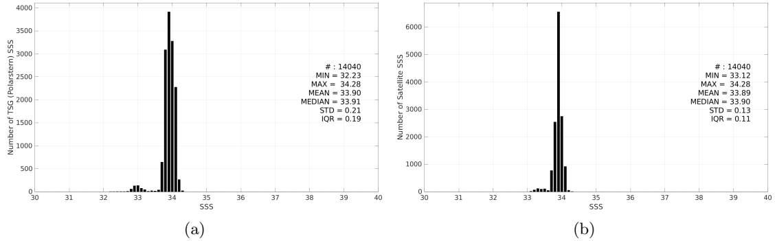
Figure 3: Histograms of SSS from TSG (Polarstern) (a) and Aquarius SSS L4 OI v5 - Monthly (IPRC) (b) considering all match-up pairs per bins of 0.1 over the Southern Ocean Pi-MEP region and for the full satellite product period.
