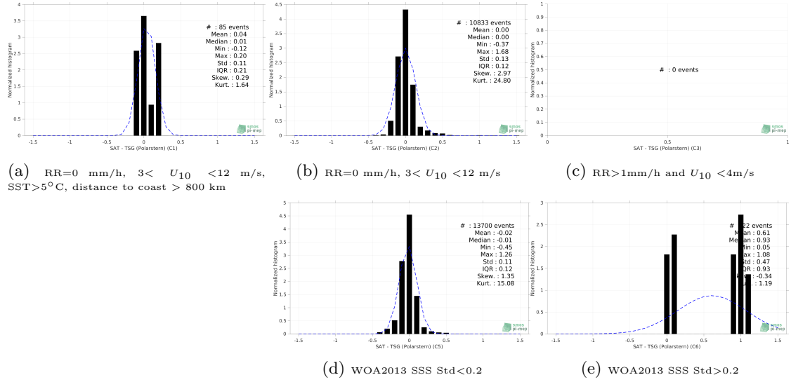
Figure 13: Normalized histogram of \Delta SSS (Aquarius SSS L4 OI v5 - Monthly (IPRC) - TSG (Polarstern)) for 5 different subdatasets corresponding to: RR=0 mm/h, 3 < U_{10} < 12 m/s, SST > 5°C, distance to coast > 800 km (a), RR=0 mm/h, 3 < U_{10} < 12 m/s (b), RR > 1mm/h and U_{10} < 4 m/s (c), WOA2013 SSS Std < 0.2 (d), WOA2013 SSS Std > 0.2 (e).
