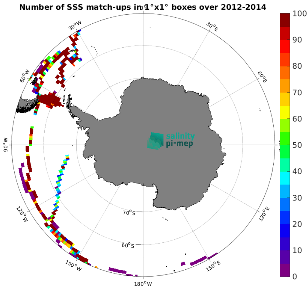
Figure 5: Number of SSS match-ups between TSG (GOSUD-Sailing-ship) SSS and the Aquarius SSS L4 OI v5 - Monthly (IPRC) SSS product for the Southern Ocean Pi-MEP region over 1^\circ \times 1^\circ boxes and for the full satellite product period.
