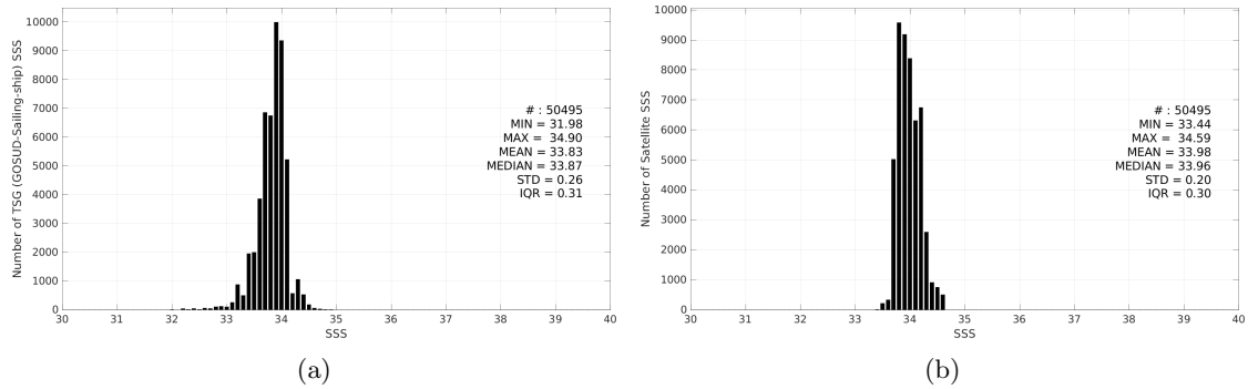
Figure 3: Histograms of SSS from TSG (GOSUD-Sailing-ship) (a) and Aquarius SSS L4 OI v5 - Monthly (IPRC) (b) considering all match-up pairs per bins of 0.1 over the Southern Ocean Pi-MEP region and for the full satellite product period.
