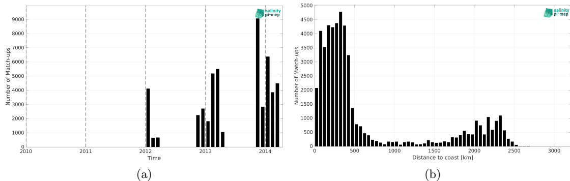
Figure 2: Number of match-ups between TSG (GOSUD-Sailing-ship) and Aquarius SSS L4 OI v5 - Monthly (IPRC) SSS as a function of time (a) and as function of the distance to coast (b) over the Southern Ocean Pi-MEP region and for the full satellite product period.
