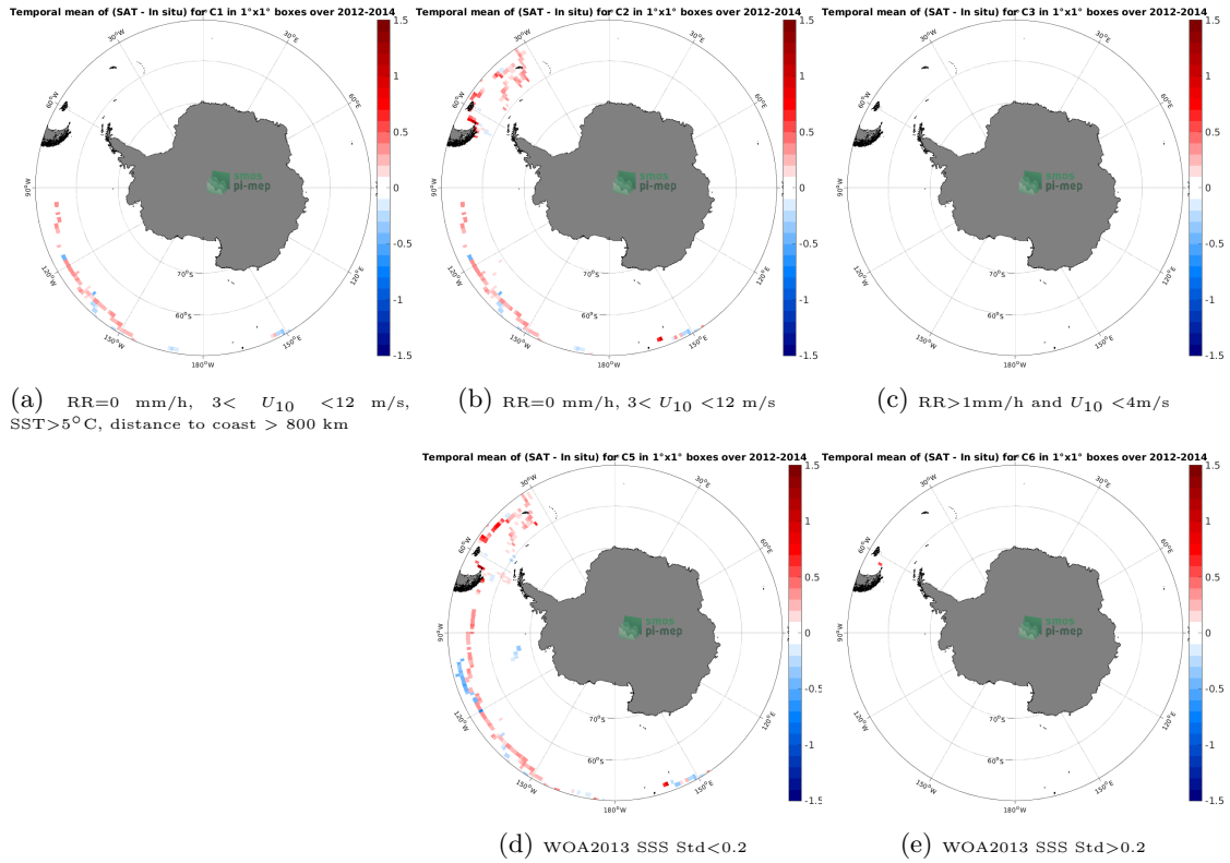
Figure 12: Temporal mean gridded over spatial boxes of size 1^\circ \times 1^\circ of \Delta SSS (Aquarius SSS L4 OI v5 - Monthly (IPRC) - TSG (GOSUD-Sailing-ship)) for 5 different subdatasets corresponding to: RR=0 mm/h, 3 < U_{10} < 12 m/s, SST>5°C, distance to coast > 800 km (a), RR=0 mm/h, 3 < U_{10} < 12 m/s (b), RR>1mm/h and U_{10} < 4 m/s (c), WOA2013 SSS Std<0.2 (d), WOA2013 SSS Std>0.2 (e).
