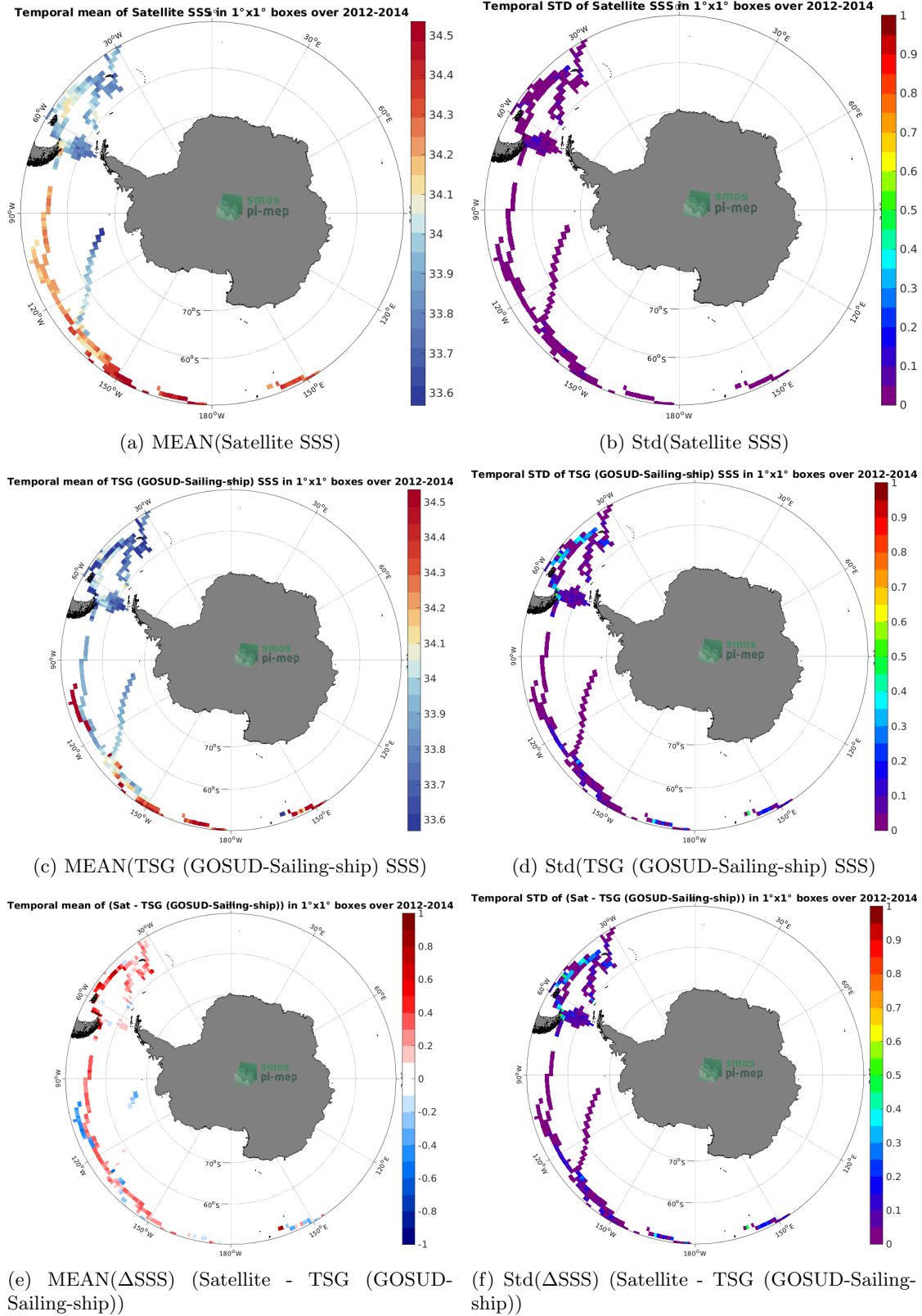
Figure 6: Temporal mean (left) and Std (right) of SSS from Aquarius SSS L4 OI v5 - Monthly (IPRC) (top), TSG (GOSUD-Sailing-ship) (middle), and of \Delta SSS (Satellite - TSG (GOSUD-Sailing-ship)). Only match-up pairs are used to generate these maps.
