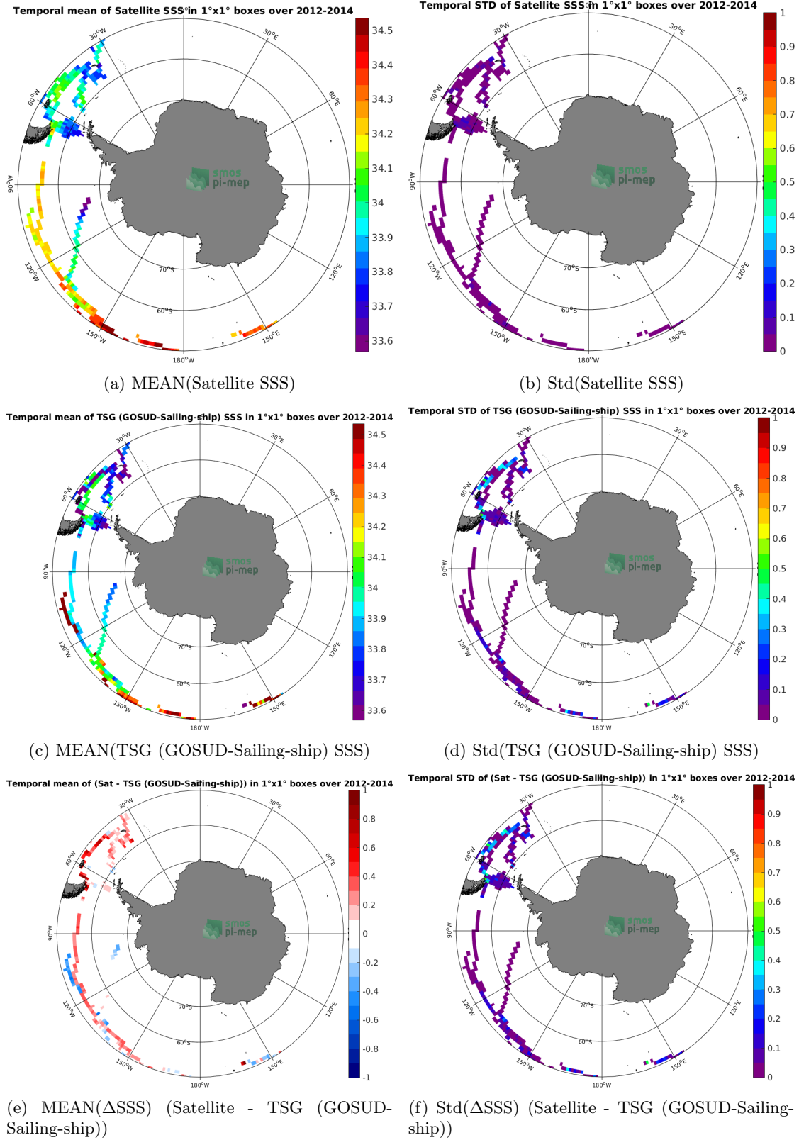
Figure 6: Temporal mean (left) and Std (right), of SSS from Aquarius SSS L4 OI v5 - Monthly (IPRC) (top), TSG (GOSUD-Sailing-ship) (middle), and of \Delta SSS (Satellite - TSG (GOSUD-Sailing-ship)). Only match-up pairs are used to generate these maps.
