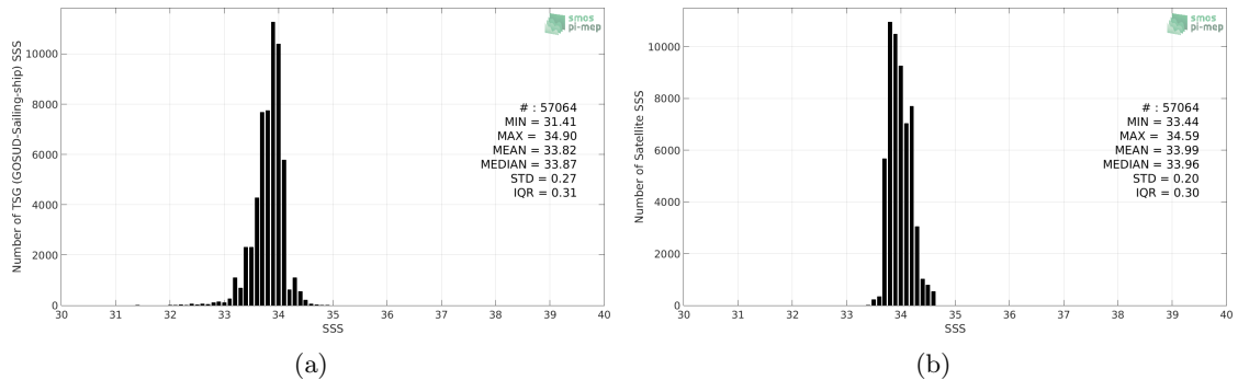
Figure 2: Histograms of SSS from TSG (GOSUD-Sailing-ship) (a) and Aquarius SSS L4 OI v5 - Monthly (IPRC) (b) considering all match-up pairs per bins of 0.1 over the Southern Ocean Pi-MEP region and for the full satellite product period.
