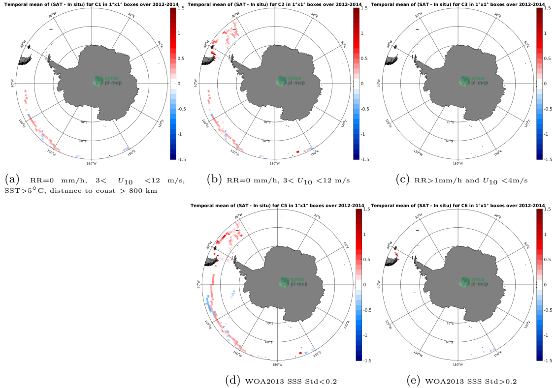
Figure 12: Temporal mean gridded over spatial boxes of size 1°x1° of \Delta SSS (Aquarius SSS L4 OI v5 - Monthly (IPRC) - TSG (GOSUD-Sailing-ship)) for 5 different subdatasets corresponding to:RR=0 mm/h, 3 < U_{10} < 12 m/s, SST>5°C, distance to coast > 800 km (a), RR=0 mm/h, 3 < U_{10} < 12 m/s (b), RR>1mm/h and U_{10} < 4 m/s (c), WOA2013 SSS Std<0.2 (d), WOA2013 SSS Std>0.2 (e).
