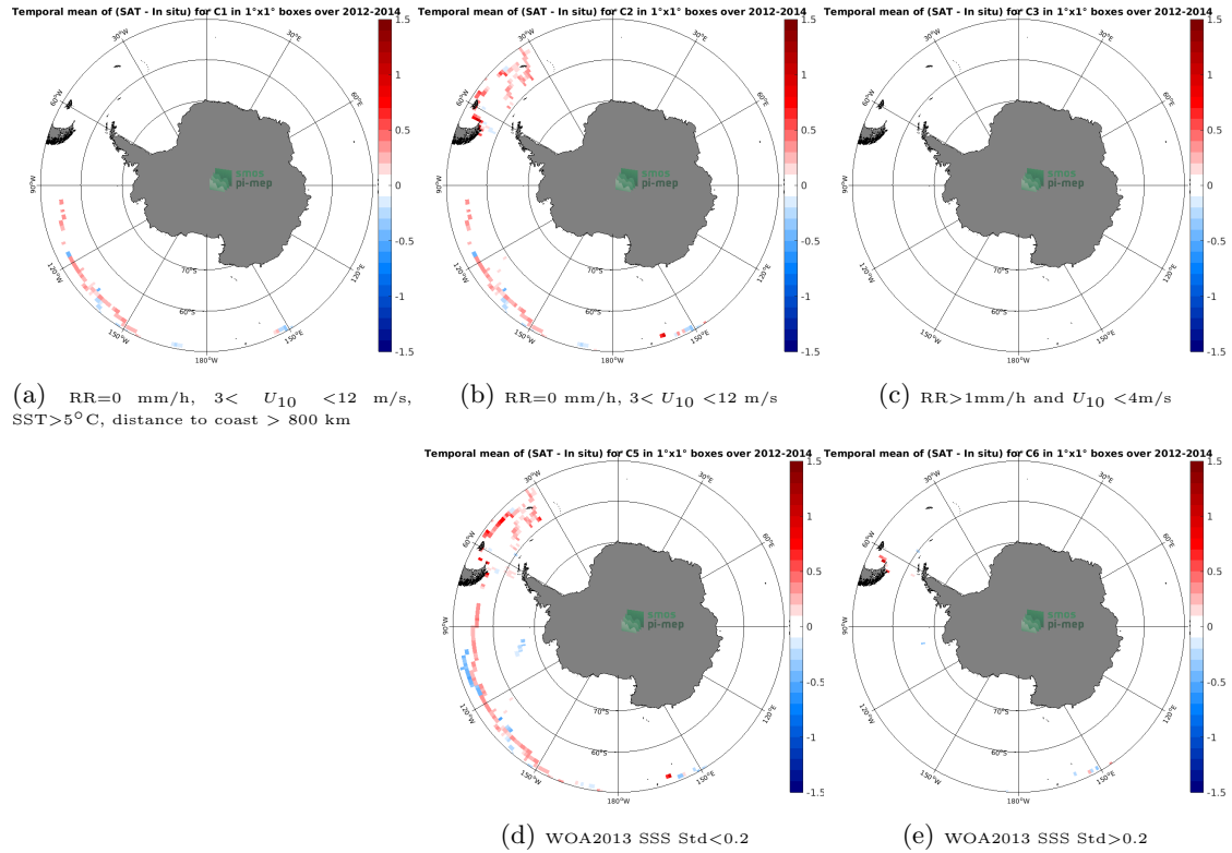
Figure 12: Temporal mean gridded over spatial boxes of size 1°x1° of \Delta SSS (Aquarius SSS L4 OI v5 - Monthly (IPRC) - TSG (GOSUD-Sailing-ship)) for 5 different subdatasets corresponding to: RR=0 mm/h, 3 < U_{10} < 12 m/s, SST > 5°C, distance to coast > 800 km (a), RR=0 mm/h, 3 < U_{10} < 12 m/s (b), RR > 1mm/h and U_{10} < 4 m/s (c), WOA2013 SSS Std < 0.2 (d), WOA2013 SSS Std > 0.2 (e).
