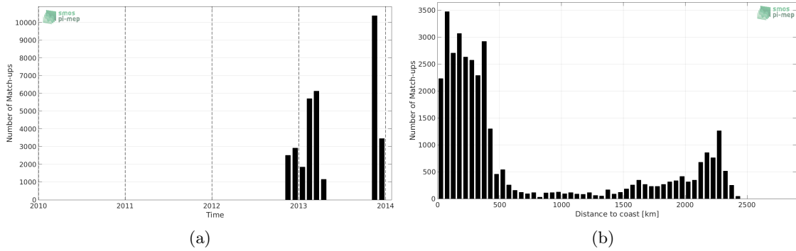
Figure 1: Number of match-ups between TSG-GOSUD-Sailing-ship and Aquarius-L4-IPRC-V5-MONTHLY SSS as a function of time (a) and as function of the distance to coast (b) over the Southern Ocean Pi-MEP region and for the full satellite product period.
