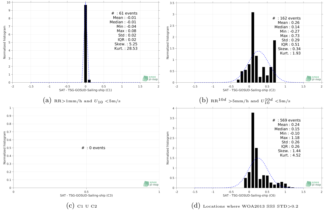
Figure 13: Normalized histogram of \Delta SSS (Aquarius-L4-IPRC-V5-MONTHLY - TSG-GOSUD-Sailing-ship) for 6 different subdatasets corresponding to: RR > 1\text{mm/h} and U_{10} < 5\text{m/s} (a), RR^{10d} > 5\text{mm/h} and U_{10}^{10d} < 5\text{m/s} (b), C1 U C2 (c), Locations where WOA2013 SSS STD > 0.2 (d).
