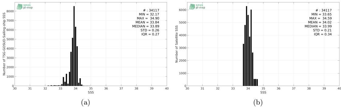
Figure 2: Histograms of SSS from TSG-GOSUD-Sailing-ship (a) and Aquarius-L4-IPRC-V5-MONTHLY (b) considering all match-up pairs per bins of 0.1 over the Southern Ocean Pi-MEP region and for the full satellite product period.
