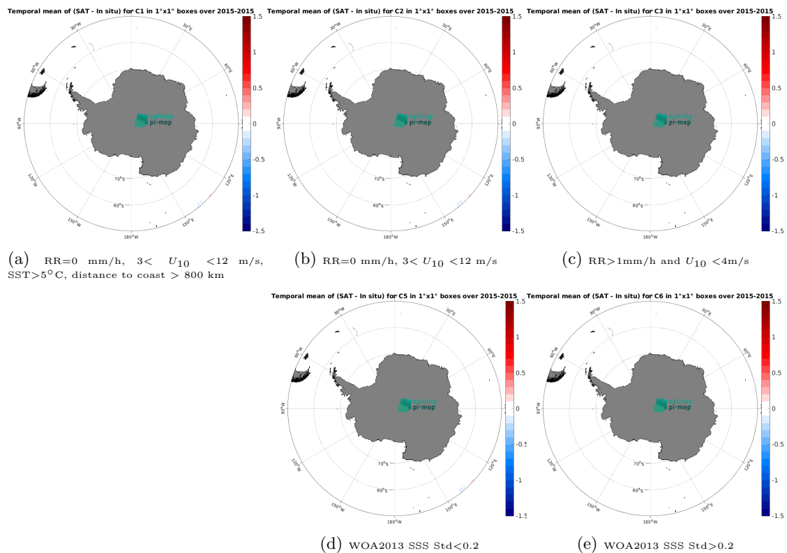
Figure 14: Temporal mean gridded over spatial boxes of size 1^\circ \times 1^\circ of \Delta SSS (Aquarius SSS L4 OI v5 - Monthly (IPRC) - TSG (GOSUD-Research-vessel)) for 5 different subdatasets corresponding to:RR=0 mm/h, 3 < U_{10} < 12 m/s, SST >5^\circ C, distance to coast > 800 km (a), RR=0 mm/h, 3 < U_{10} < 12 m/s (b), RR >1 mm/h and U_{10} < 4 m/s (c), WOA2013 SSS Std <0.2 (d), WOA2013 SSS Std >0.2 (e).
