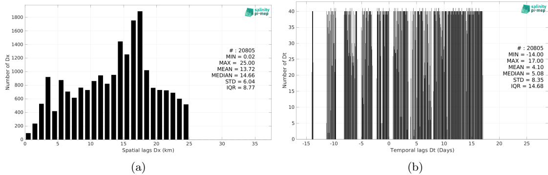
Figure 6: Histograms of the spatial (a) and temporal (b) lags between the location/time of the TSG (GOSUD-Research-vessel) measurement and the date of the corresponding Aquarius SSS L4 OI v5 - Monthly (IPRC) SSS pixel.
