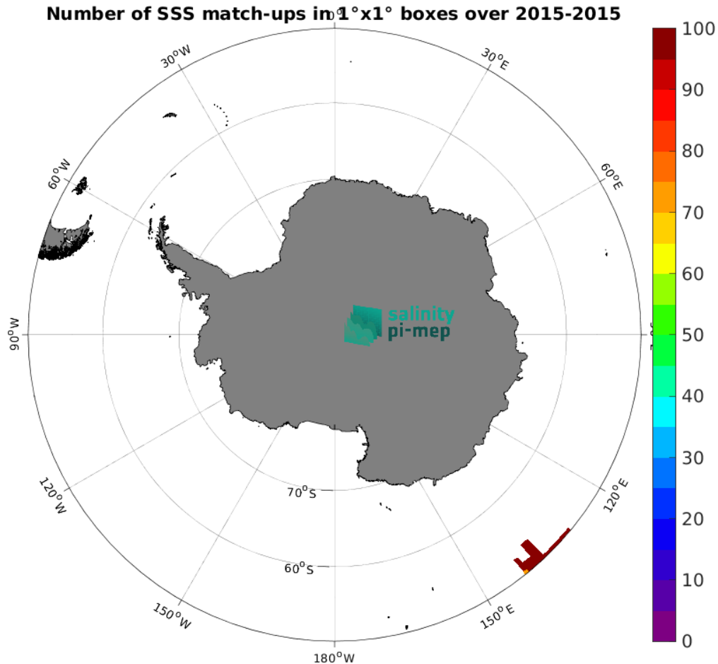
Figure 5: Number of SSS match-ups between TSG (GOSUD-Research-vessel) SSS and the Aquarius SSS L4 OI v5 - Monthly (IPRC) SSS product for the Southern Ocean Pi-MEP region over 1^\circ \times 1^\circ boxes and for the full satellite product period.
