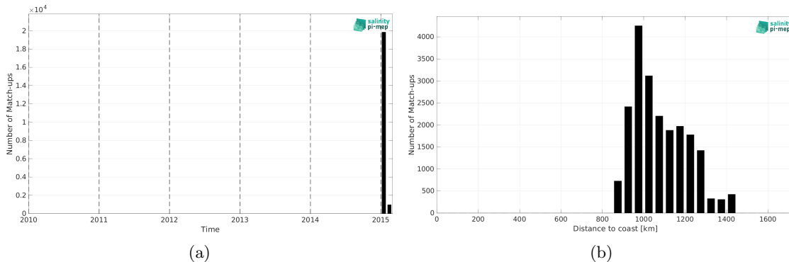
Figure 2: Number of match-ups between TSG (GOSUD-Research-vessel) and Aquarius SSS L4 OI v5 - Monthly (IPRC) SSS as a function of time (a) and as function of the distance to coast (b) over the Southern Ocean Pi-MEP region and for the full satellite product period.
