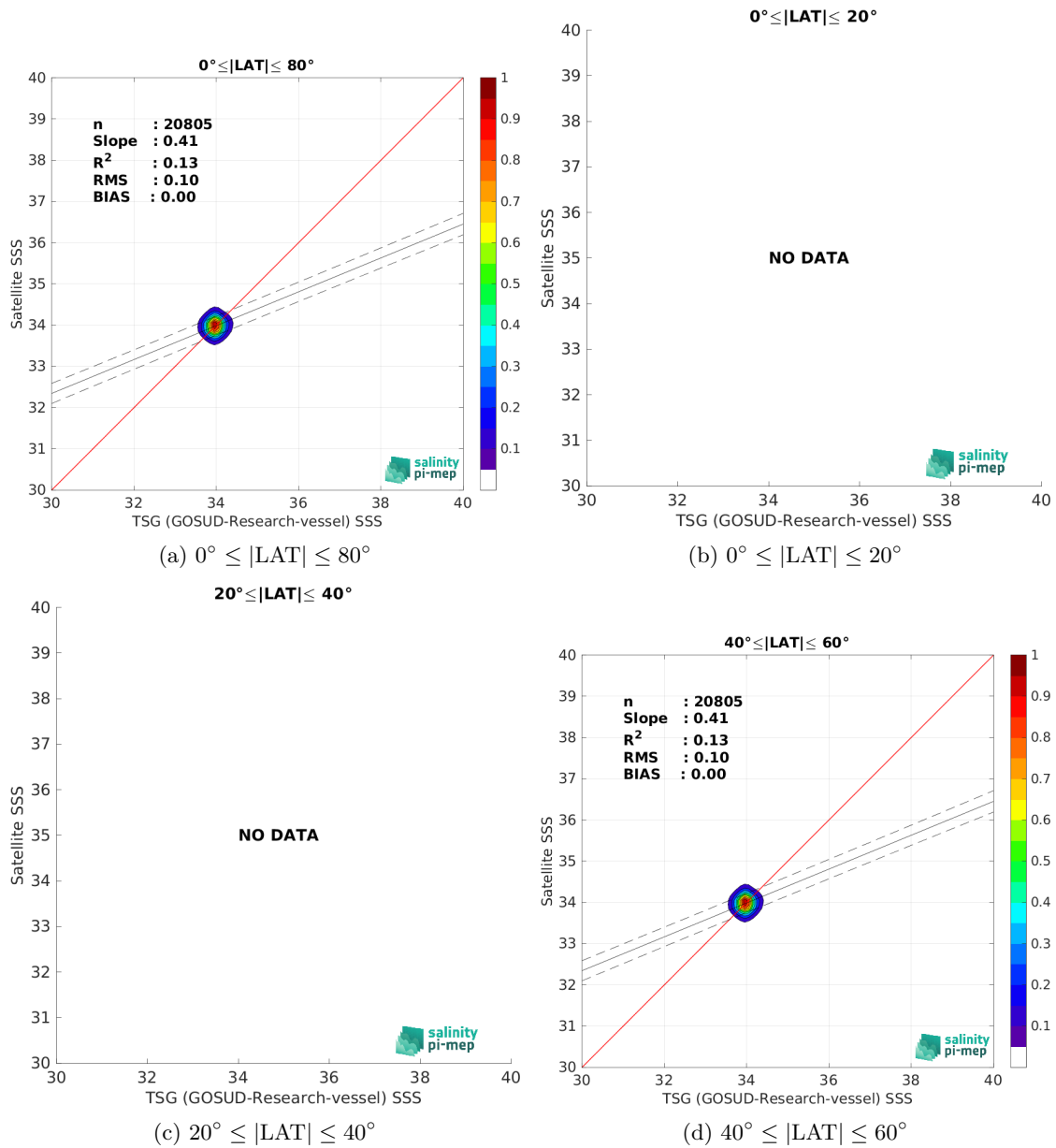
Figure 10: Contour maps of the concentration of Aquarius SSS L4 OI v5 - Monthly (IPRC) SSS (y-axis) versus TSG (GOSUD-Research-vessel) SSS (x-axis) at match-up pairs for different latitude bands. For each plot, the red line shows x=y . The black thin and dashed lines indicate a linear fit through the data cloud and the \pm 95\% confidence levels, respectively. The number match-up pairs n , the slope and R^2 coefficient of the linear fit, the root mean square (RMS) and the mean bias between satellite and in situ data are indicated for each latitude band in each plots.
