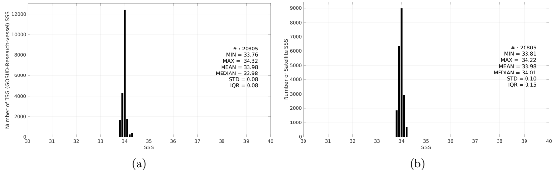
Figure 3: Histograms of SSS from TSG (GOSUD-Research-vessel) (a) and Aquarius SSS L4 OI v5 - Monthly (IPRC) (b) considering all match-up pairs per bins of 0.1 over the Southern Ocean Pi-MEP region and for the full satellite product period.
