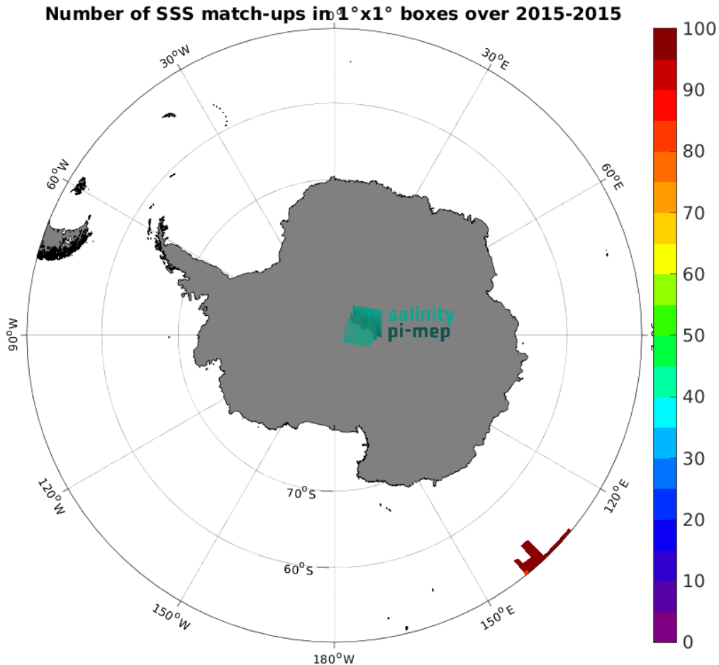
Figure 4: Number of SSS match-ups between TSG (GOSUD-Research-vessel) SSS and the Aquarius SSS L4 OI v5 - Monthly (IPRC) SSS product for the Southern Ocean Pi-MEP region over 1^\circ \times 1^\circ boxes and for the full satellite product period.
