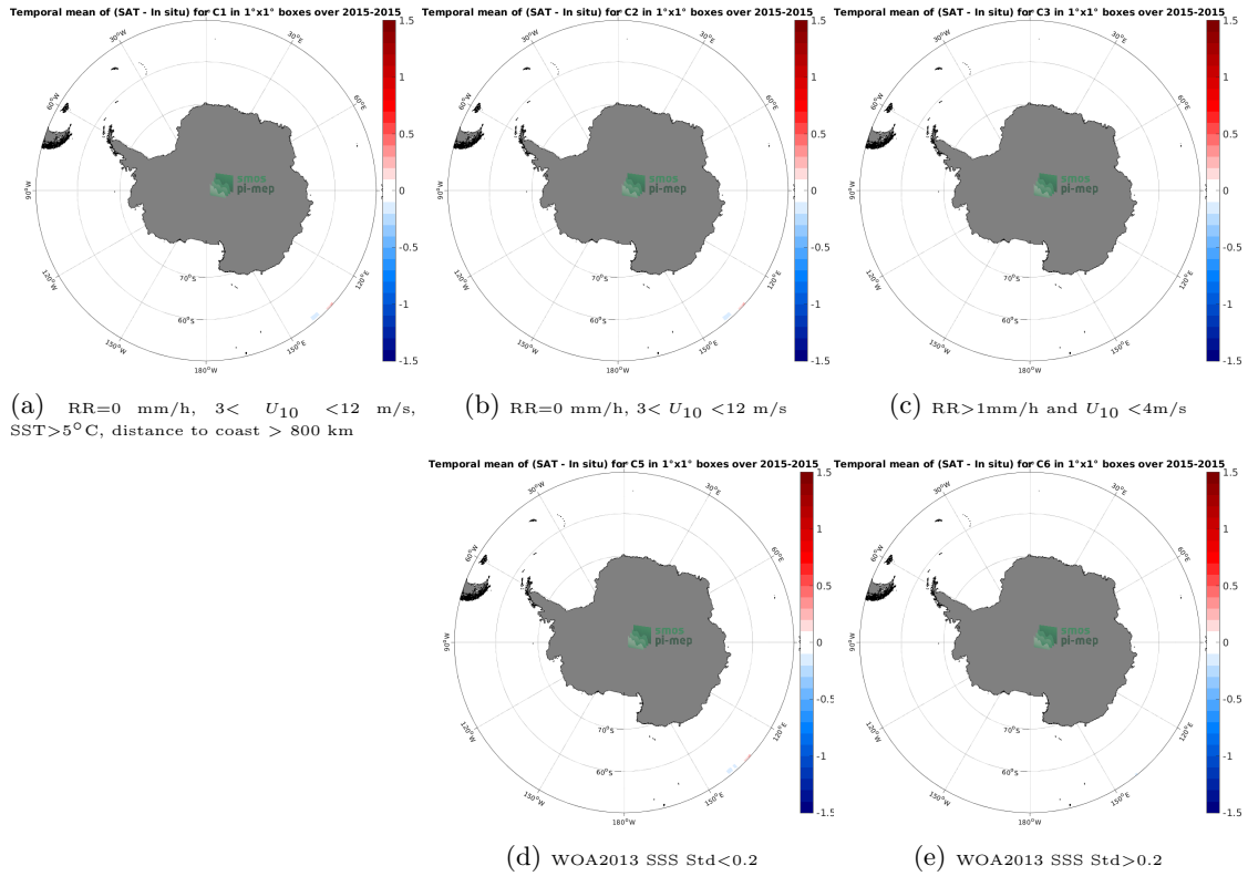
Figure 12: Temporal mean gridded over spatial boxes of size 1°x1° of \Delta SSS (Aquarius SSS L4 OI v5 - Monthly (IPRC) - TSG (GOSUD-Research-vessel)) for 5 different subdatasets corresponding to: RR=0 mm/h, 3 < U_{10} < 12 m/s, SST>5°C, distance to coast > 800 km (a), RR=0 mm/h, 3 < U_{10} < 12 m/s (b), RR>1mm/h and U_{10} < 4 m/s (c), WOA2013 SSS Std<0.2 (d), WOA2013 SSS Std>0.2 (e).
