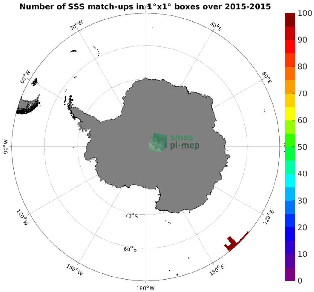
Figure 4: Number of SSS match-ups between TSG (GOSUD-Research-vessel) SSS and the Aquarius SSS L4 OI v5 - Monthly (IPRC) SSS product for the Southern Ocean Pi-MEP region over 1^\circ \times 1^\circ boxes and for the full satellite product period.
