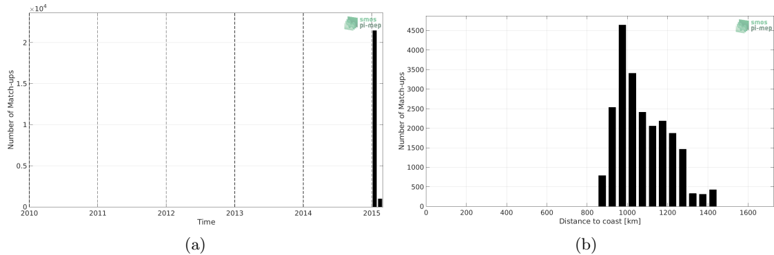
Figure 1: Number of match-ups between TSG (GOSUD-Research-vessel) and Aquarius SSS L4 OI v5 - Monthly (IPRC) SSS as a function of time (a) and as function of the distance to coast (b) over the Southern Ocean Pi-MEP region and for the full satellite product period.
