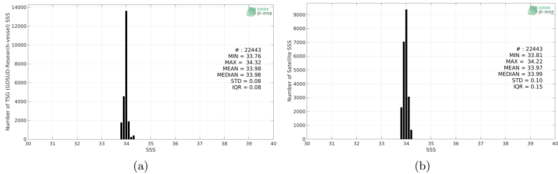
Figure 2: Histograms of SSS from TSG (GOSUD-Research-vessel) (a) and Aquarius SSS L4 OI v5 - Monthly (IPRC) (b) considering all match-up pairs per bins of 0.1 over the Southern Ocean Pi-MEP region and for the full satellite product period.
