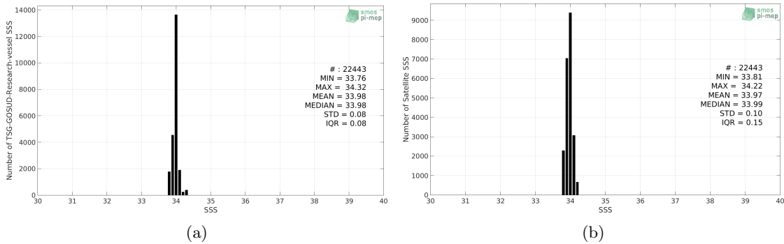
Figure 2: Histograms of SSS from TSG-GOSUD-Research-vessel (a) and Aquarius-L4-IPRC-V5-MONTHLY (b) considering all match-up pairs per bins of 0.1 over the Southern Ocean Pi-MEP region and for the full satellite product period.
