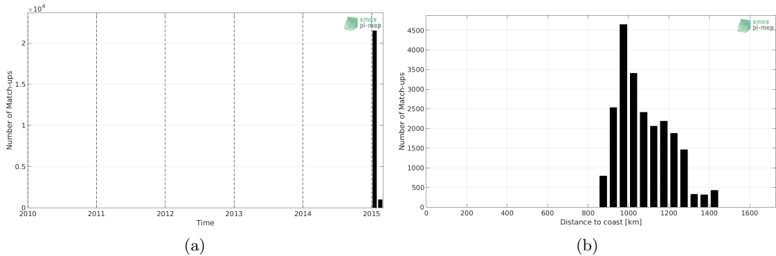
Figure 1: Number of match-ups between TSG-GOSUD-Research-vessel and Aquarius-L4-IPRC-V5-MONTHLY SSS as a function of time (a) and as function of the distance to coast (b) over the Southern Ocean Pi-MEP region and for the full satellite product period.
