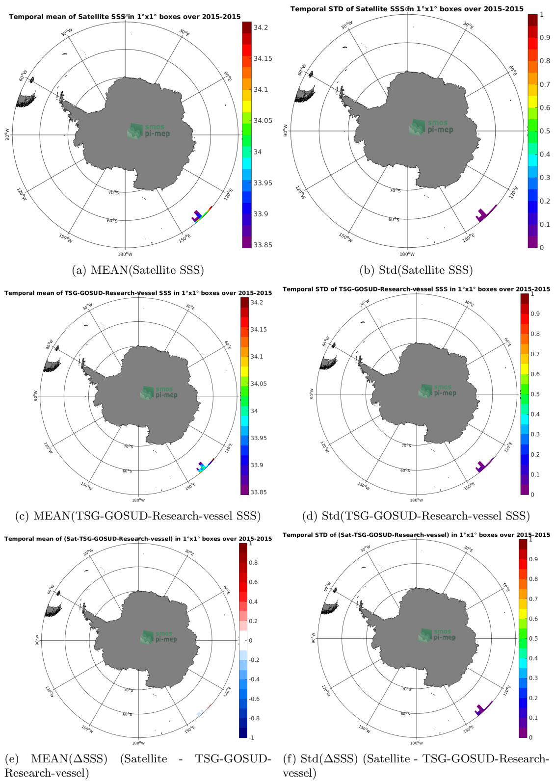
Figure 6: Temporal mean (left) and Std (right) of SSS from Aquarius-L4-IPRC-V5-MONTHLY (top), TSG-GOSUD-Research-vessel (middle), and \Delta SSS (Satellite - TSG-GOSUD-Research-vessel). Only match-up pairs are used to generate these maps.
