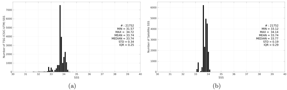
Figure 3: Histograms of SSS from TSG (CSIC-UTM) (a) and Aquarius SSS L4 OI v5 - Monthly (IPRC) (b) considering all match-up pairs per bins of 0.1 over the Southern Ocean Pi-MEP region and for the full satellite product period.
