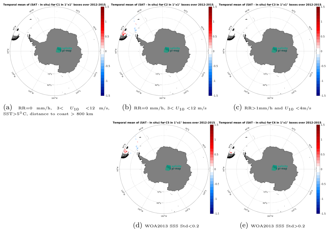
Figure 14: Temporal mean gridded over spatial boxes of size 1^\circ \times 1^\circ of \Delta SSS (Aquarius SSS L4 OI v5 - Monthly (IPRC) - TSG (CSIC-UTM)) for 5 different subdatasets corresponding to: RR=0 mm/h, 3 < U_{10} < 12 m/s, SST > 5^\circ\text{C} , distance to coast > 800 km (a), RR=0 mm/h, 3 < U_{10} < 12 m/s (b), RR > 1 mm/h and U_{10} < 4 m/s (c), WOA2013 SSS Std < 0.2 (d), WOA2013 SSS Std > 0.2 (e).
