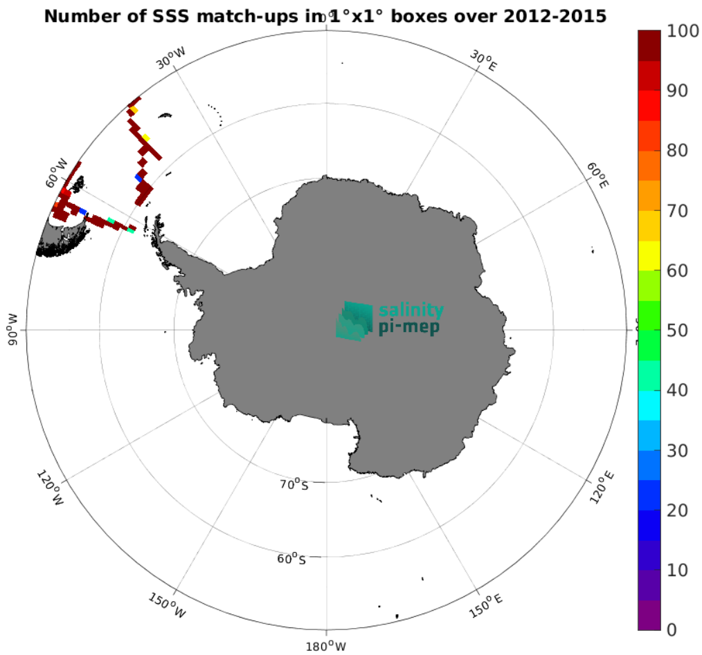
Figure 5: Number of SSS match-ups between TSG (CSIC-UTM) SSS and the Aquarius SSS L4 OI v5 - Monthly (IPRC) SSS product for the Southern Ocean Pi-MEP region over 1^{\circ} \times 1^{\circ} boxes and for the full satellite product period.
