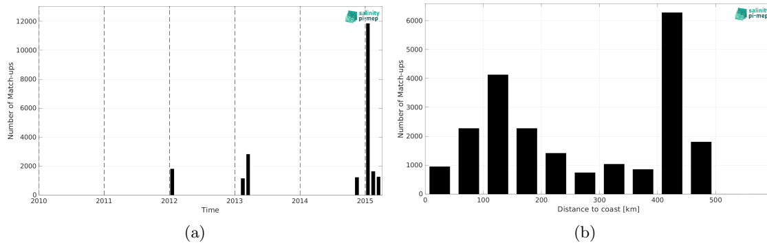
Figure 2: Number of match-ups between TSG (CSIC-UTM) and Aquarius SSS L4 OI v5 - Monthly (IPRC) SSS as a function of time (a) and as function of the distance to coast (b) over the Southern Ocean Pi-MEP region and for the full satellite product period.
