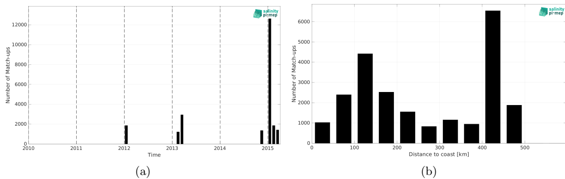
Figure 1: Number of match-ups between TSG (CSIC-UTM) and Aquarius SSS L4 OI v5 - Monthly (IPRC) SSS as a function of time (a) and as function of the distance to coast (b) over the Southern Ocean Pi-MEP region and for the full satellite product period.
