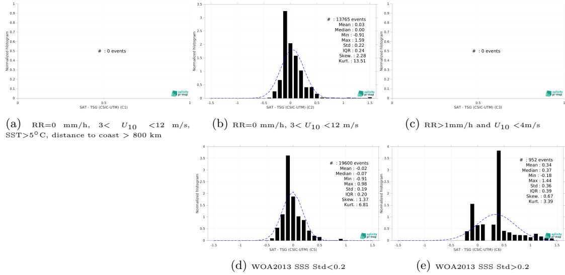
Figure 13: Normalized histogram of \Delta SSS (Aquarius SSS L4 OI v5 - Monthly (IPRC) - TSG (CSIC-UTM)) for 5 different subdatasets corresponding to: RR=0 mm/h, 3 < U_{10} < 12 m/s, SST > 5°C, distance to coast > 800 km (a), RR=0 mm/h, 3 < U_{10} < 12 m/s (b), RR > 1mm/h and U_{10} < 4 m/s (c), WOA2013 SSS Std < 0.2 (d), WOA2013 SSS Std > 0.2 (e).
