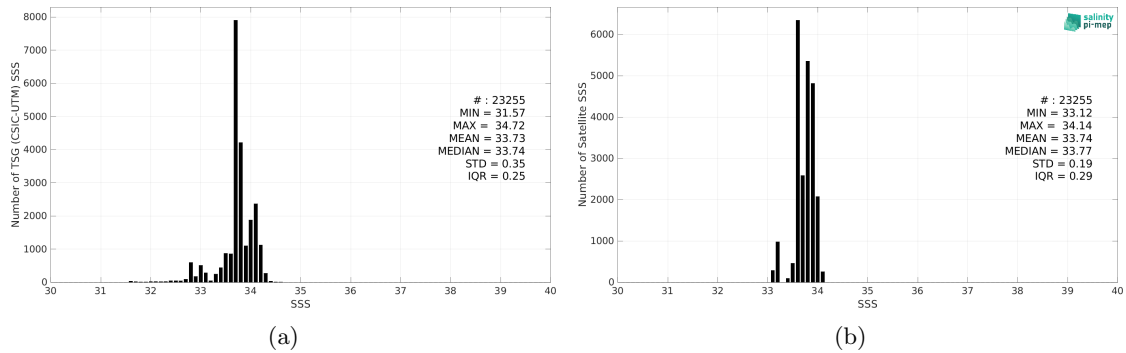
Figure 2: Histograms of SSS from TSG (CSIC-UTM) (a) and Aquarius SSS L4 OI v5 - Monthly (IPRC) (b) considering all match-up pairs per bins of 0.1 over the Southern Ocean Pi-MEP region and for the full satellite product period.
