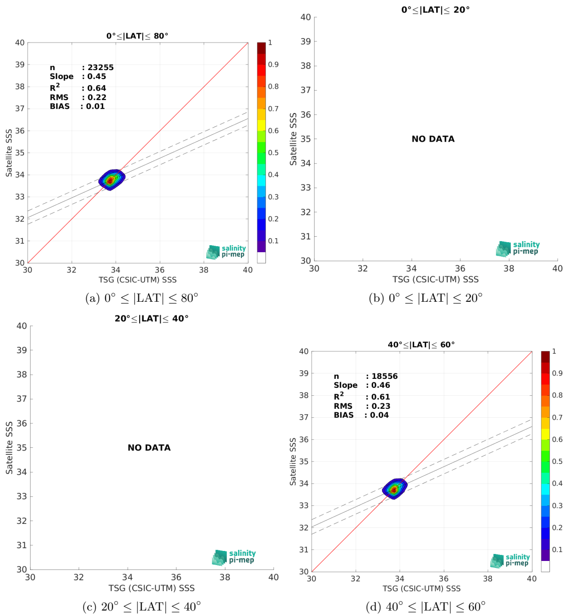
Figure 9: Contour maps of the concentration of Aquarius SSS L4 OI v5 - Monthly (IPRC) SSS (y-axis) versus TSG (CSIC-UTM) SSS (x-axis) at match-up pairs for different latitude bands. For each plot, the red line shows x=y . The black thin and dashed lines indicate a linear fit through the data cloud and the \pm 95\% confidence levels, respectively. The number match-up pairs n , the slope and R^2 coefficient of the linear fit, the root mean square (RMS) and the mean bias between satellite and in situ data are indicated for each latitude band in each plots.
