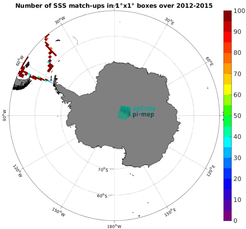
Figure 4: Number of SSS match-ups between TSG (CSIC-UTM) SSS and the Aquarius SSS L4 OI v5 - Monthly (IPRC) SSS product for the Southern Ocean Pi-MEP region over 1^{\circ} \times 1^{\circ} boxes and for the full satellite product period.
