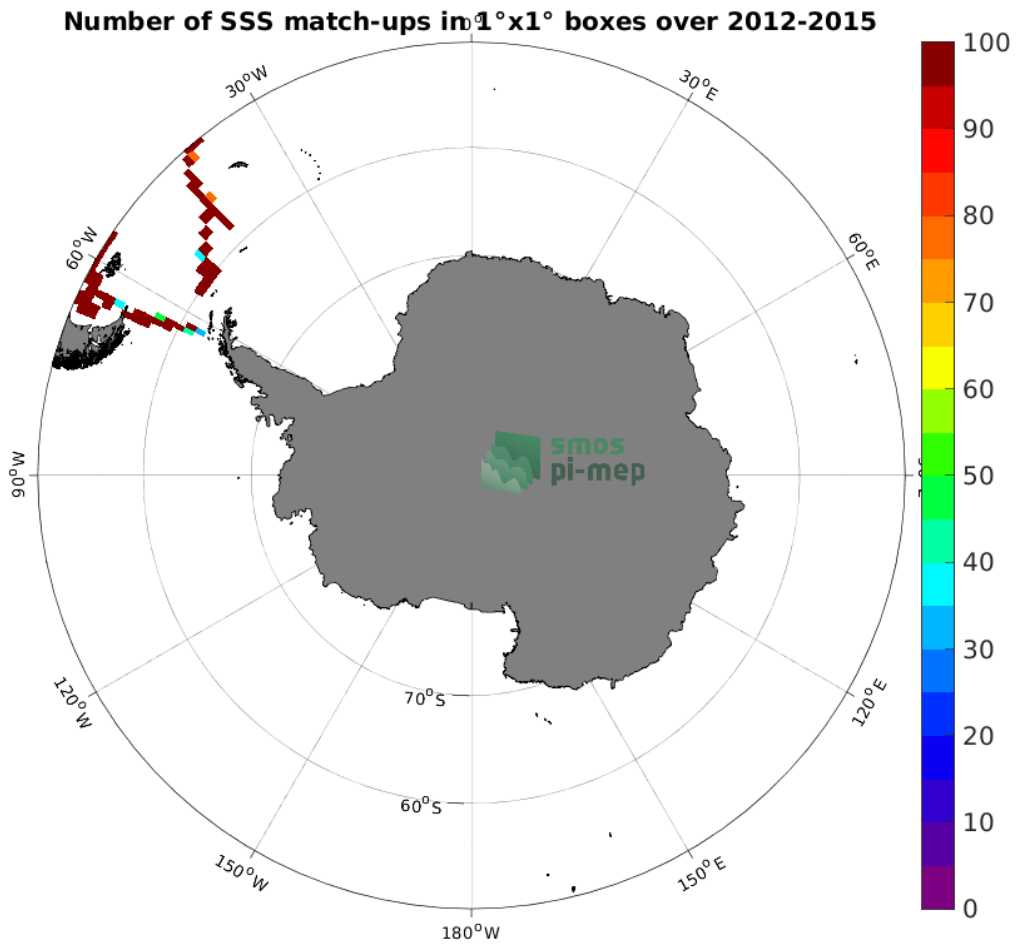
Figure 4: Number of SSS match-ups between TSG (CSIC-UTM) SSS and the Aquarius SSS L4 OI v5 - Monthly (IPRC) SSS product for the Southern Ocean Pi-MEP region over 1^\circ \times 1^\circ boxes and for the full satellite product period.
