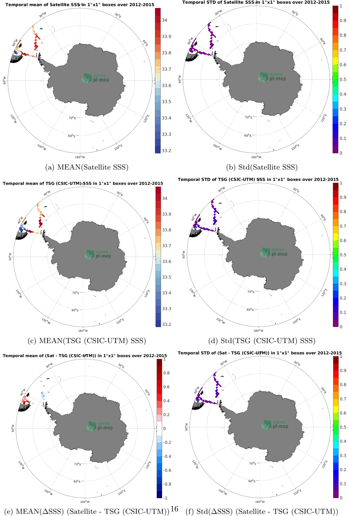
Figure 6: Temporal mean (left) and Std (right) of SSS from Aquarius SSS L4 OI v5 - Monthly (IPRC) (top), TSG (CSIC-UTM) (middle), and of \Delta SSS (Satellite - TSG (CSIC-UTM)). Only match-up pairs are used to generate these maps.
