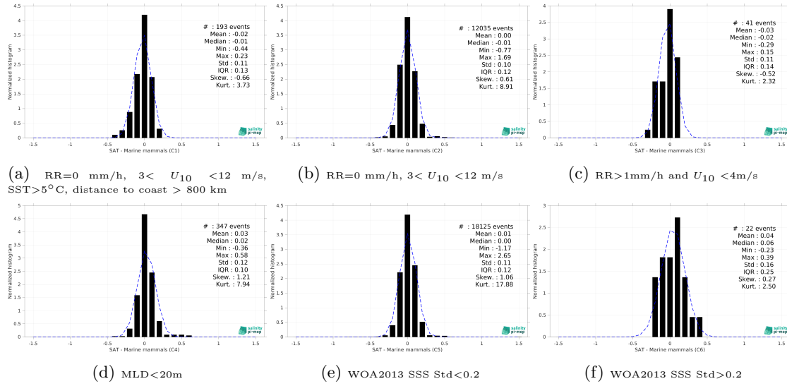
Figure 15: Normalized histogram of \Delta SSS (Aquarius SSS L4 OI v5 - Monthly (IPRC) - Marine mammals) for 6 different subdatasets corresponding to: RR=0 mm/h, 3 < U_{10} < 12 m/s, SST > 5°C, distance to coast > 800 km (a), RR=0 mm/h, 3 < U_{10} < 12 m/s (b), RR > 1mm/h and U_{10} < 4 m/s (c), MLD < 20m (d), WOA2013 SSS Std < 0.2 (e), WOA2013 SSS Std > 0.2 (f).
