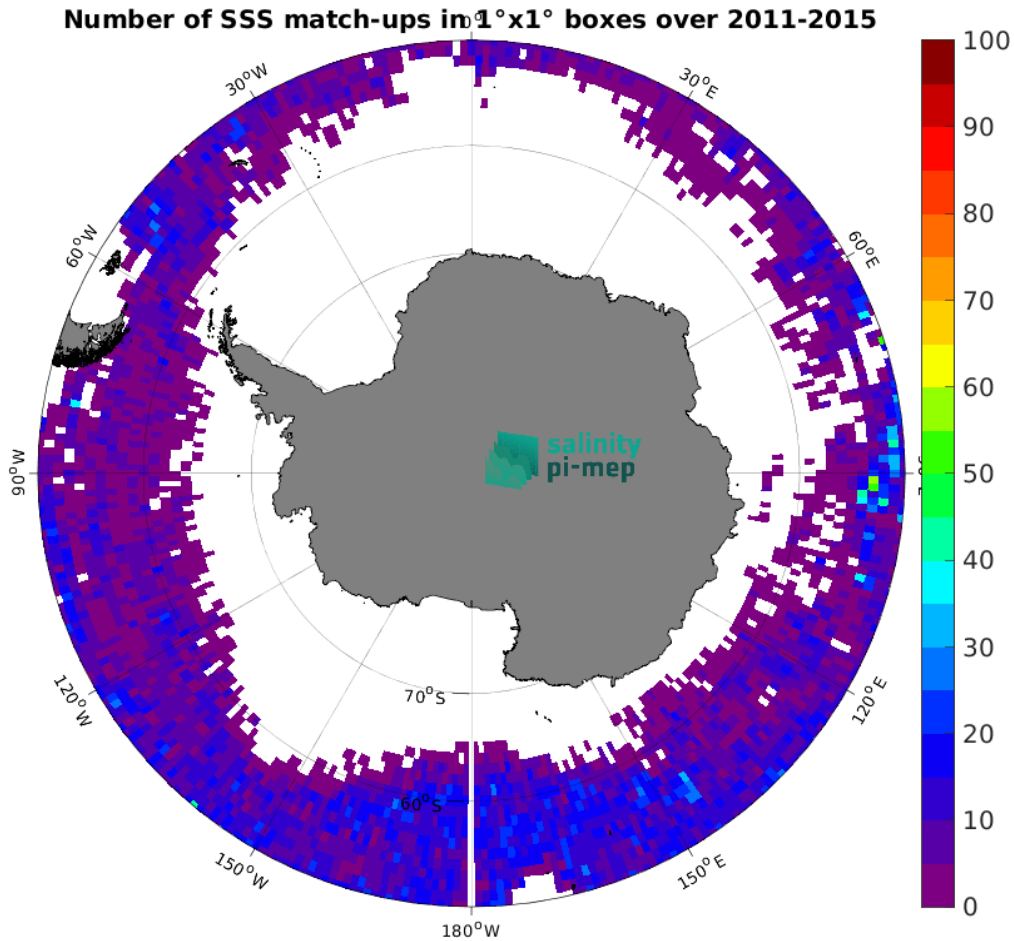
Figure 5: Number of SSS match-ups between Argo SSS and the Aquarius SSS L4 OI v5 - Monthly (IPRC) SSS product for the Southern Ocean Pi-MEP region over 1^\circ \times 1^\circ boxes and for the full satellite product period.
