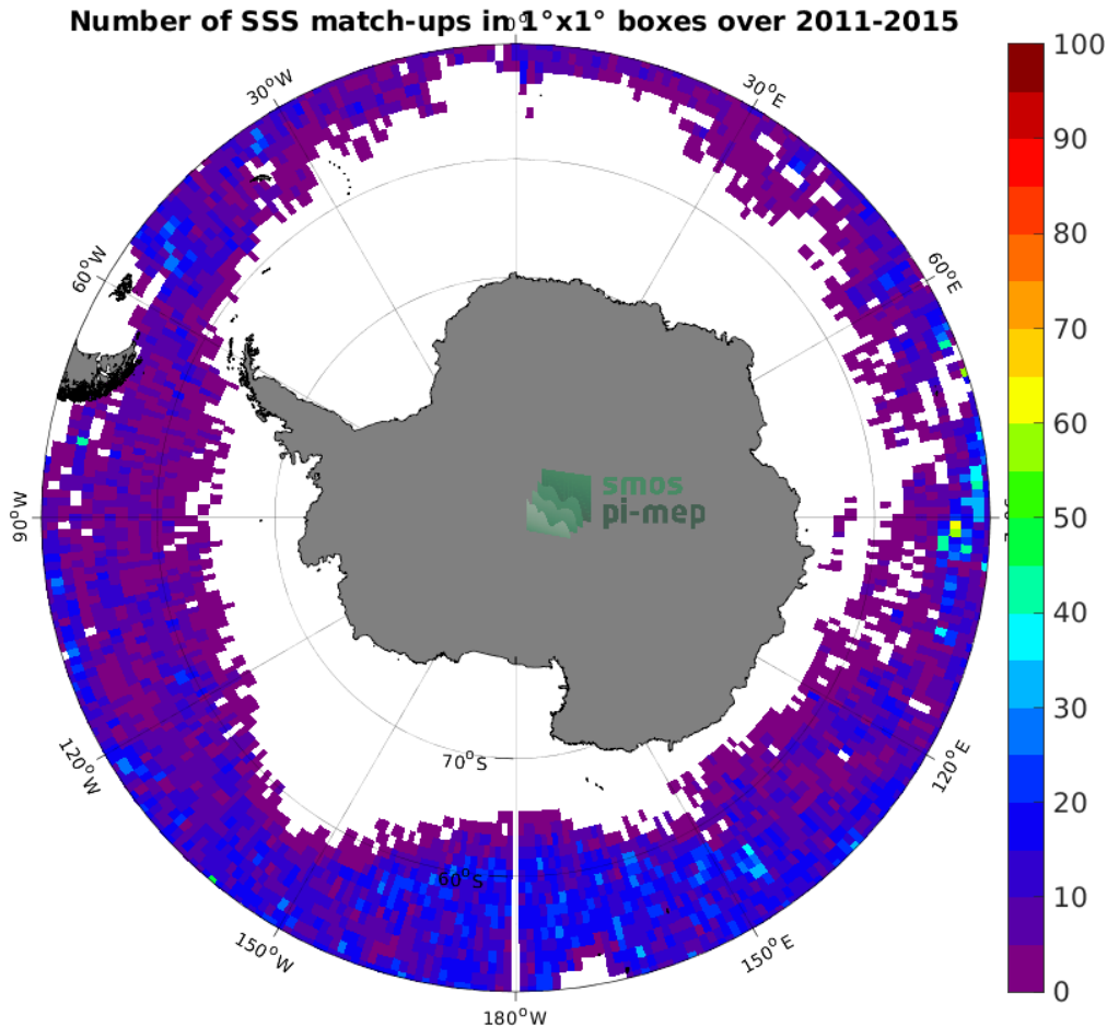
Figure 4: Number of SSS match-ups between Argo SSS and the Aquarius SSS L4 OI v5 - Monthly (IPRC) SSS product for the Southern Ocean Pi-MEP region over 1^\circ \times 1^\circ boxes and for the full satellite product period.
