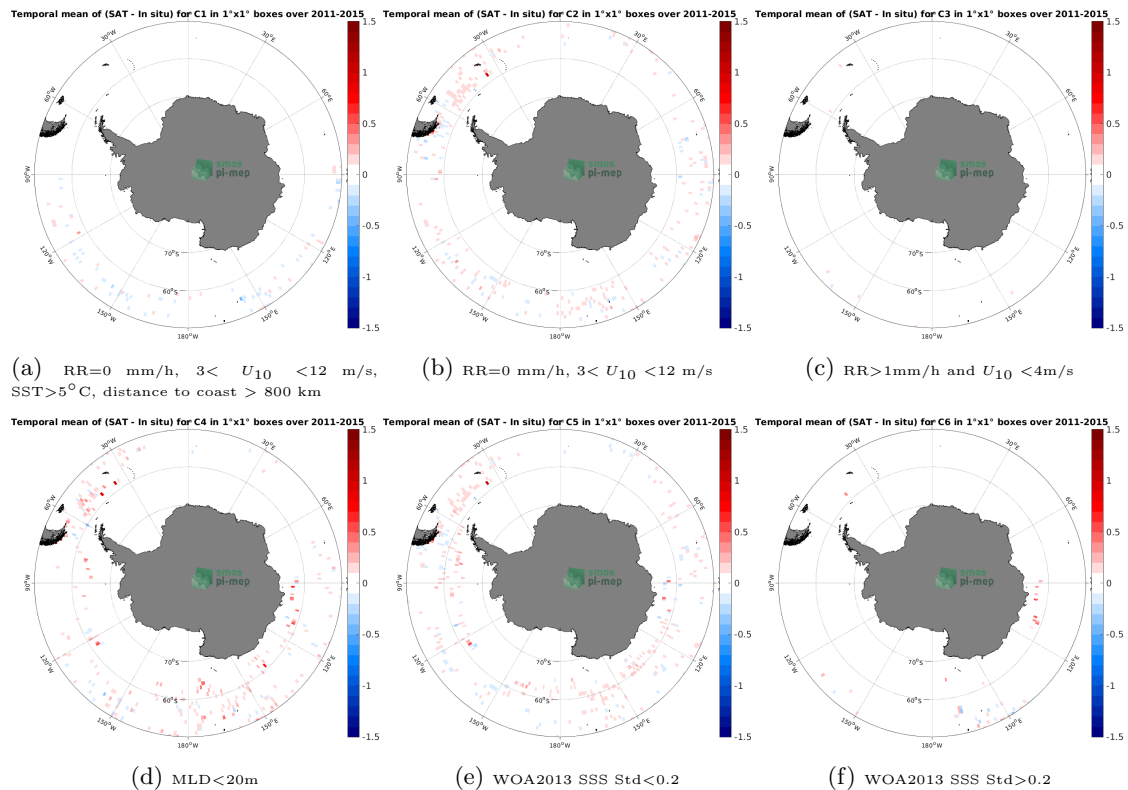
Figure 12: Temporal mean gridded over spatial boxes of size 1^{\circ}\times 1^{\circ} of \Delta\text{SSS} (Aquarius SSS L4 OI v5 - Monthly (IPRC) - Argo) for 6 different subdatasets corresponding to: \text{RR}=0 mm/h, 3 < U_{10} < 12 m/s, \text{SST} > 5^{\circ}\text{C} , distance to coast > 800 km (a), \text{RR}=0 mm/h, 3 < U_{10} < 12 m/s (b), \text{RR} > 1\text{mm/h} and U_{10} < 4\text{m/s} (c), \text{MLD} < 20\text{m} (d), WOA2013 SSS Std < 0.2 (e), WOA2013 SSS Std > 0.2 (f).
