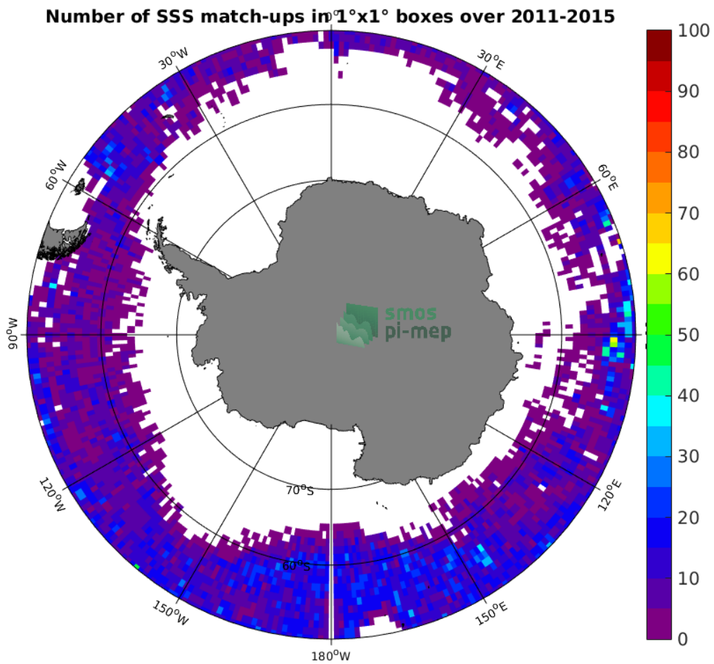
Figure 4: Number of SSS match-ups between Argo SSS and the Aquarius-L4-IPRC-V5-MONTHLY SSS product for the Southern Ocean Pi-MEP region over 1^\circ \times 1^\circ boxes and for the full satellite product period.
