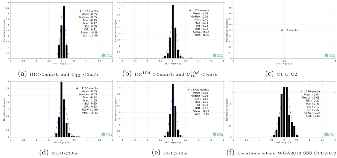
Figure 13: Normalized histogram of \Delta SSS (Aquarius-L4-IPRC-V5-MONTHLY - Argo) for 6 different subdatasets corresponding to: RR > 1mm/h and U_{10} < 5 m/s (a), RR 10d > 5mm/h and U_{10}^{10d} < 5 m/s (b), C1 U C2 (c), MLD < 20m (d), BLT > 10m (e), Locations where WOA2013 SSS STD > 0.2 (f).
