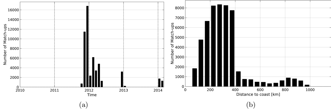
Figure 1: Number of match-ups between TSG-SAMOS and Aquarius-L4-IPRC-V4-WEEKLY SSS as a function of time (a) and as function of the distance to coast (b) over the Southern Ocean Pi-MEP region and for the full satellite product period.
