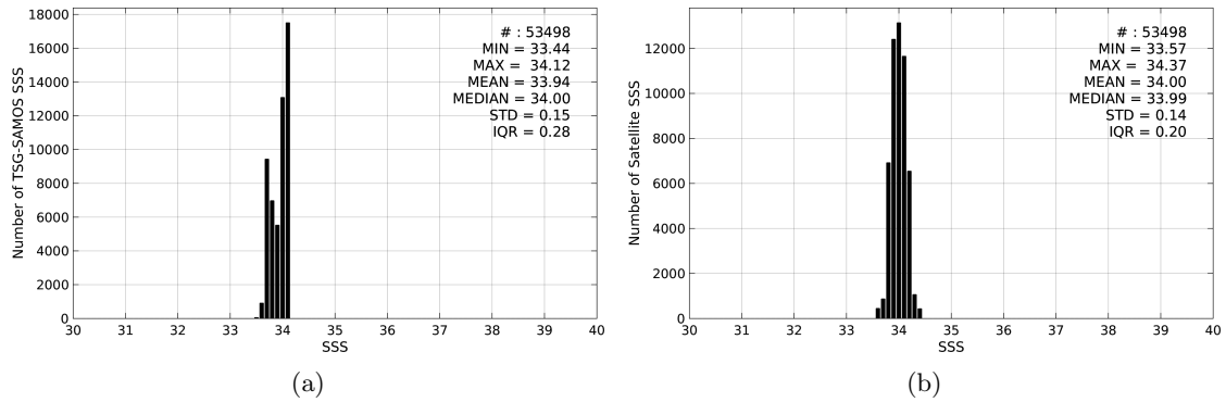
Figure 2: Histograms of SSS from TSG-SAMOS (a) and Aquarius-L4-IPRC-V4-WEEKLY (b) considering all match-up pairs per bins of 0.1 over the Southern Ocean Pi-MEP region and for the full satellite product period.
