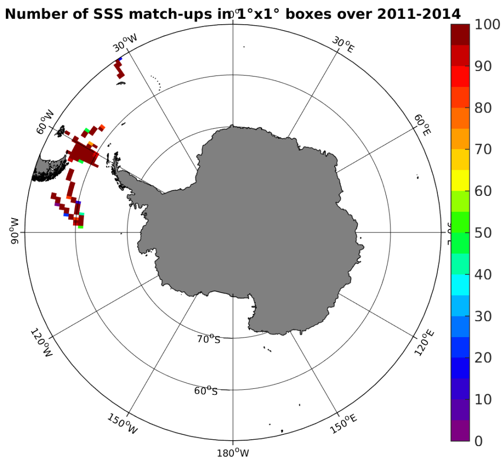
Figure 4: Number of SSS match-ups between TSG-SAMOS SSS and the Aquarius-L4-IPRC-V4-WEEKLY SSS product for the Southern Ocean Pi-MEP region over 1^\circ \times 1^\circ boxes and for the full satellite product period.
