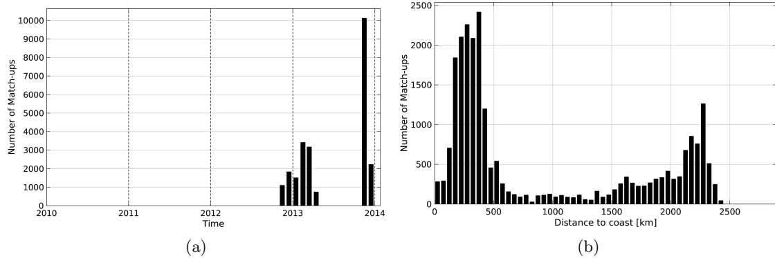
Figure 1: Number of match-ups between TSG-GOSUD-Sailing-ship and Aquarius-L4-IPRC-V4-WEEKLY SSS as a function of time (a) and as function of the distance to coast (b) over the Southern Ocean Pi-MEP region and for the full satellite product period.
