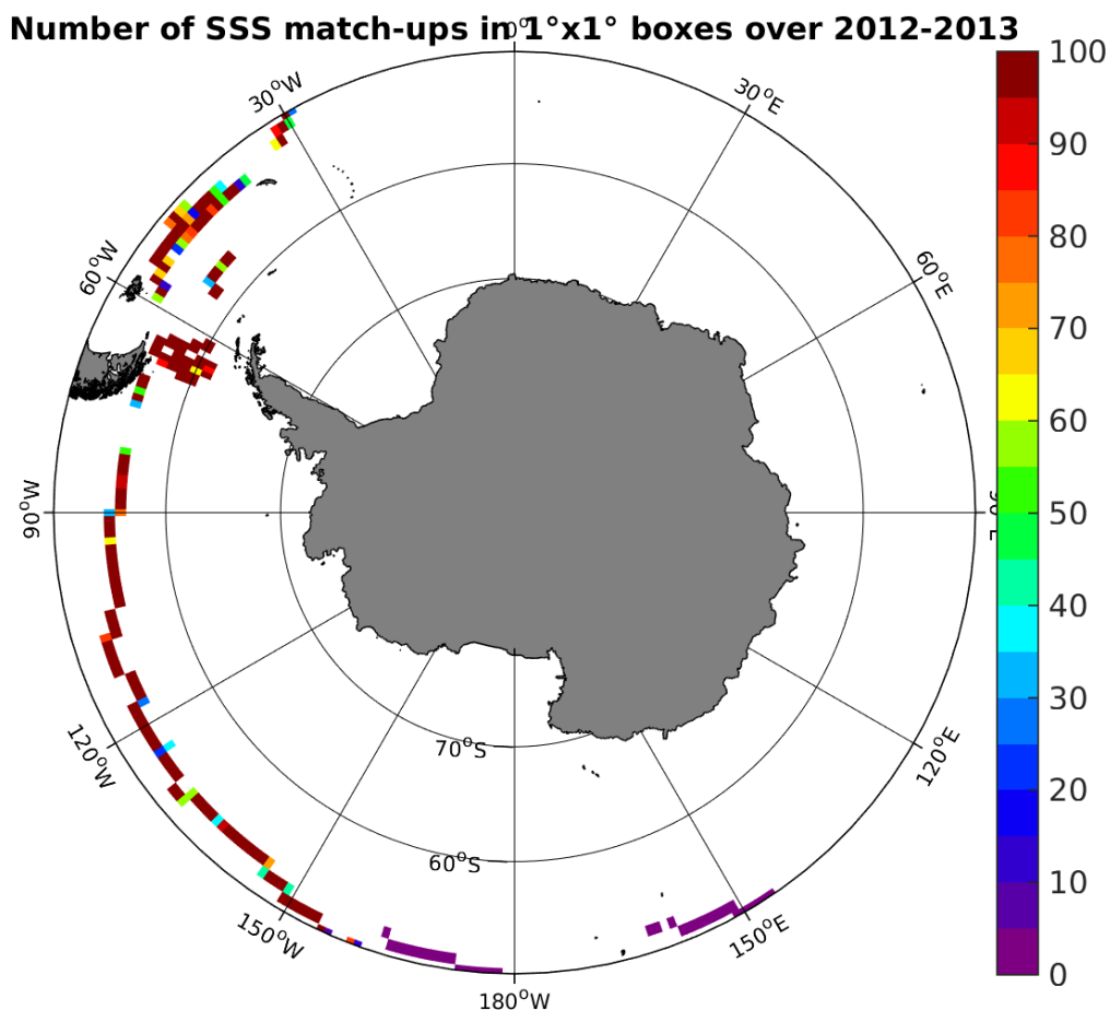
Figure 4: Number of SSS match-ups between TSG-GOSUD-Sailing-ship SSS and the Aquarius-L4-IPRC-V4-WEEKLY SSS product for the Southern Ocean Pi-MEP region over 1°x1° boxes and for the full satellite product period.
