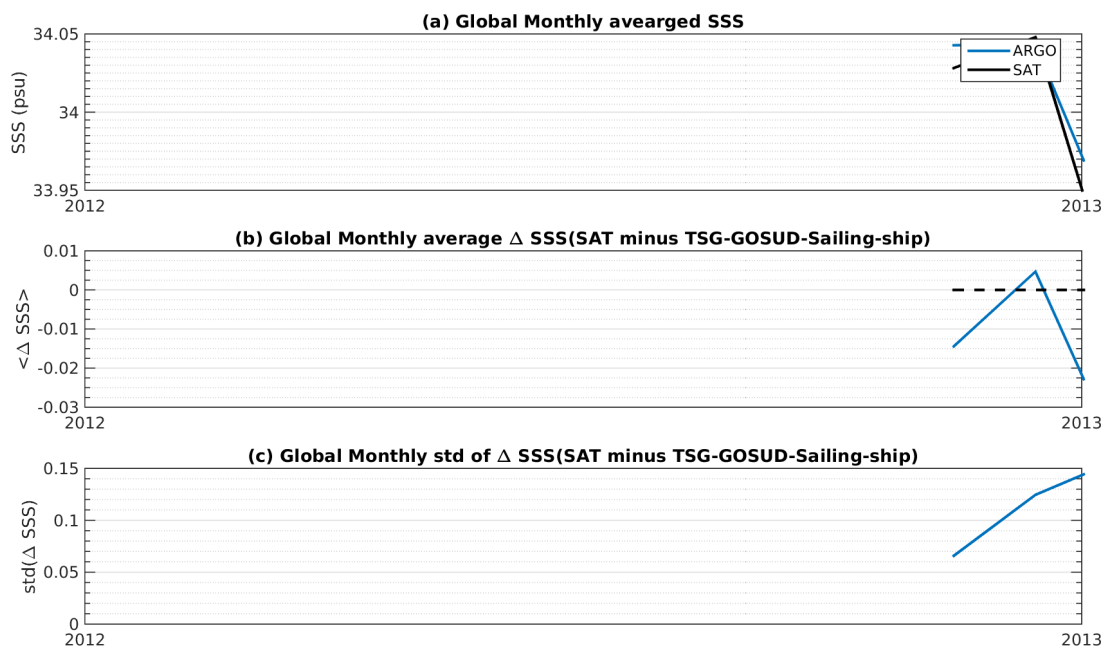
Figure 7: Time series of the monthly averaged mean SSS (top), mean \Delta SSS (Satellite - TSG-GOSUD-Sailing-ship) and STD of \Delta SSS (Satellite - TSG-GOSUD-Sailing-ship) over the Southern Ocean Pi-MEP region considering all match-ups collected by the Pi-MEP platform.
