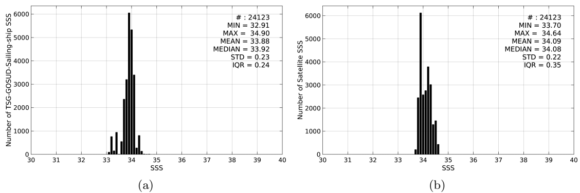
Figure 2: Histograms of SSS from TSG-GOSUD-Sailing-ship (a) and Aquarius-L4-IPRC-V4-WEEKLY (b) considering all match-up pairs per bins of 0.1 over the Southern Ocean Pi-MEP region and for the full satellite product period.
