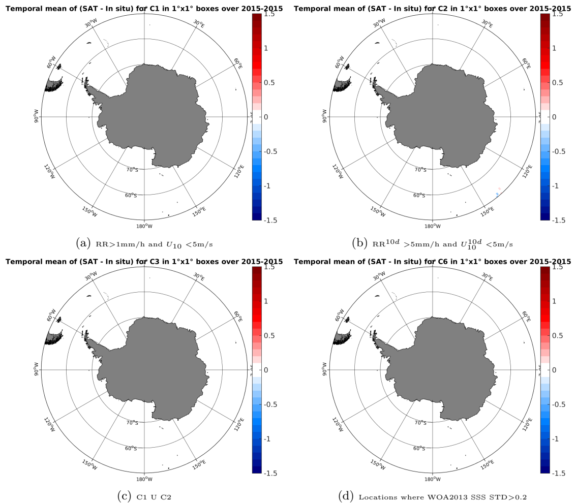
Figure 12: Temporal mean gridded over spatial boxes of size 1^\circ \times 1^\circ of \Delta SSS (Aquarius-L4-IPRC-V4-WEEKLY - TSG-GOSUD-Research-vessel) for 4 different subdatasets corresponding to:RR > 1 mm/h and U_{10} < 5 m/s (a), RR^{10d} > 5 mm/h and U_{10}^{10d} < 5 m/s (b), C1 U C2 (c),Locations where WOA2013 SSS STD > 0.2 (d).
