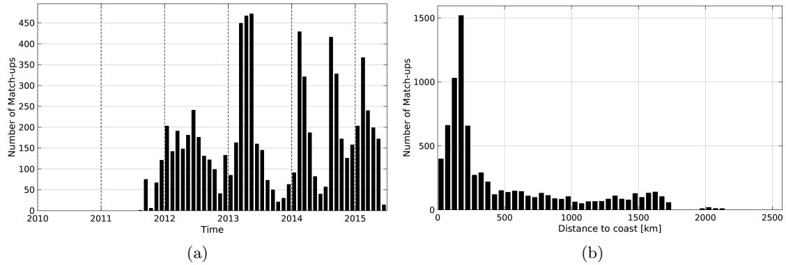
Figure 1: Number of match-ups between Sea mammals and Aquarius-L4-IPRC-V4-WEEKLY SSS as a function of time (a) and as function of the distance to coast (b) over the Southern Ocean Pi-MEP region and for the full satellite product period.
