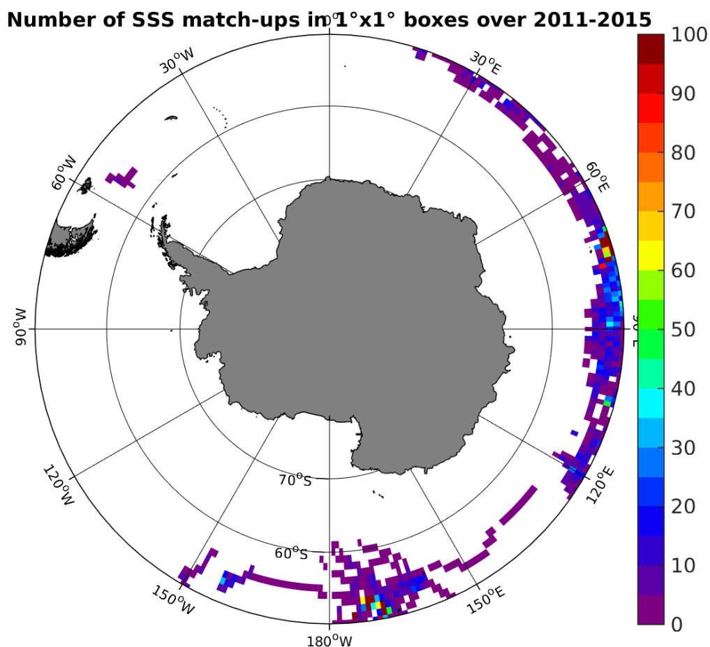
Figure 4: Number of SSS match-ups between Sea mammals SSS and the Aquarius-L4-IPRC-V4-WEEKLY SSS product for the Southern Ocean Pi-MEP region over 1^\circ \times 1^\circ boxes and for the full satellite product period.
