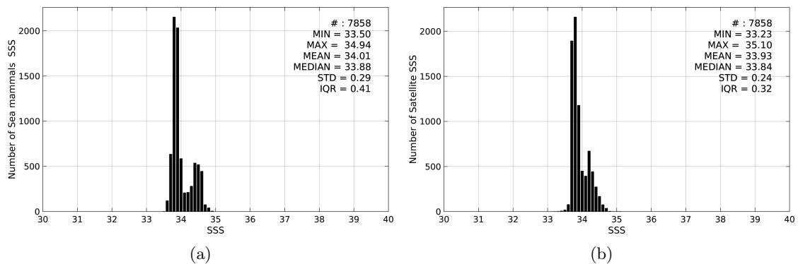
Figure 2: Histograms of SSS from Sea mammals (a) and Aquarius-L4-IPRC-V4-WEEKLY (b) considering all match-up pairs per bins of 0.1 over the Southern Ocean Pi-MEP region and for the full satellite product period.
