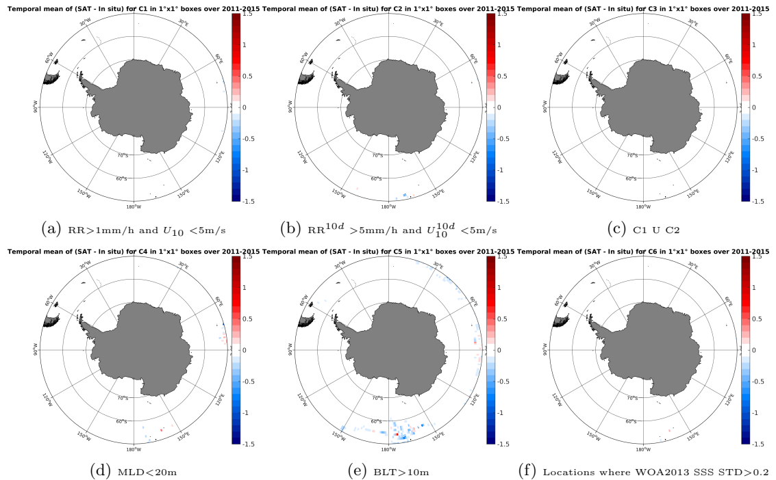
Figure 12: Temporal mean gridded over spatial boxes of size 1^{\circ} \times 1^{\circ} of \Delta SSS (Aquarius-L4-IPRC-V4-WEEKLY - Sea mammals) for 6 different subdatasets corresponding to: RR > 1\text{mm/h} and U_{10} < 5\text{m/s} (a), RR^{10d} > 5\text{mm/h} and U_{10}^{10d} < 5\text{m/s} (b), C1 U C2 (c), MLD < 20\text{m} (d), BLT > 10\text{m} (e), Locations where WOA2013 SSS STD > 0.2 (f).
