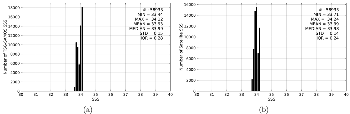
Figure 2: Histograms of SSS from TSG-SAMOS (a) and Aquarius-L4-IPRC-V4-MONTHLY (b) considering all match-up pairs per bins of 0.1 over the Southern Ocean Pi-MEP region and for the full satellite product period.
