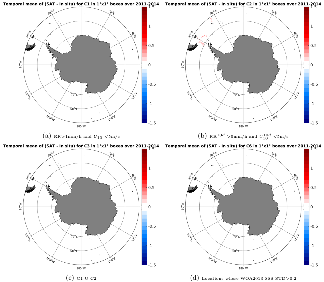
Figure 12: Temporal mean gridded over spatial boxes of size 1°x1° of \Delta SSS (Aquarius-L4-IPRC-V4-MONTHLY - TSG-SAMOS) for 4 different subdatasets corresponding to: RR > 1\text{mm/h} and U_{10} < 5\text{m/s} (a), RR^{10d} > 5\text{mm/h} and U_{10}^{10d} < 5\text{m/s} (b), C1 U C2 (c), Locations where WOA2013 SSS STD > 0.2 (d).
