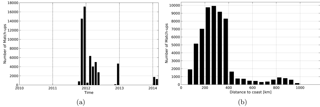
Figure 1: Number of match-ups between TSG-SAMOS and Aquarius-L4-IPRC-V4-MONTHLY SSS as a function of time (a) and as function of the distance to coast (b) over the Southern Ocean Pi-MEP region and for the full satellite product period.
