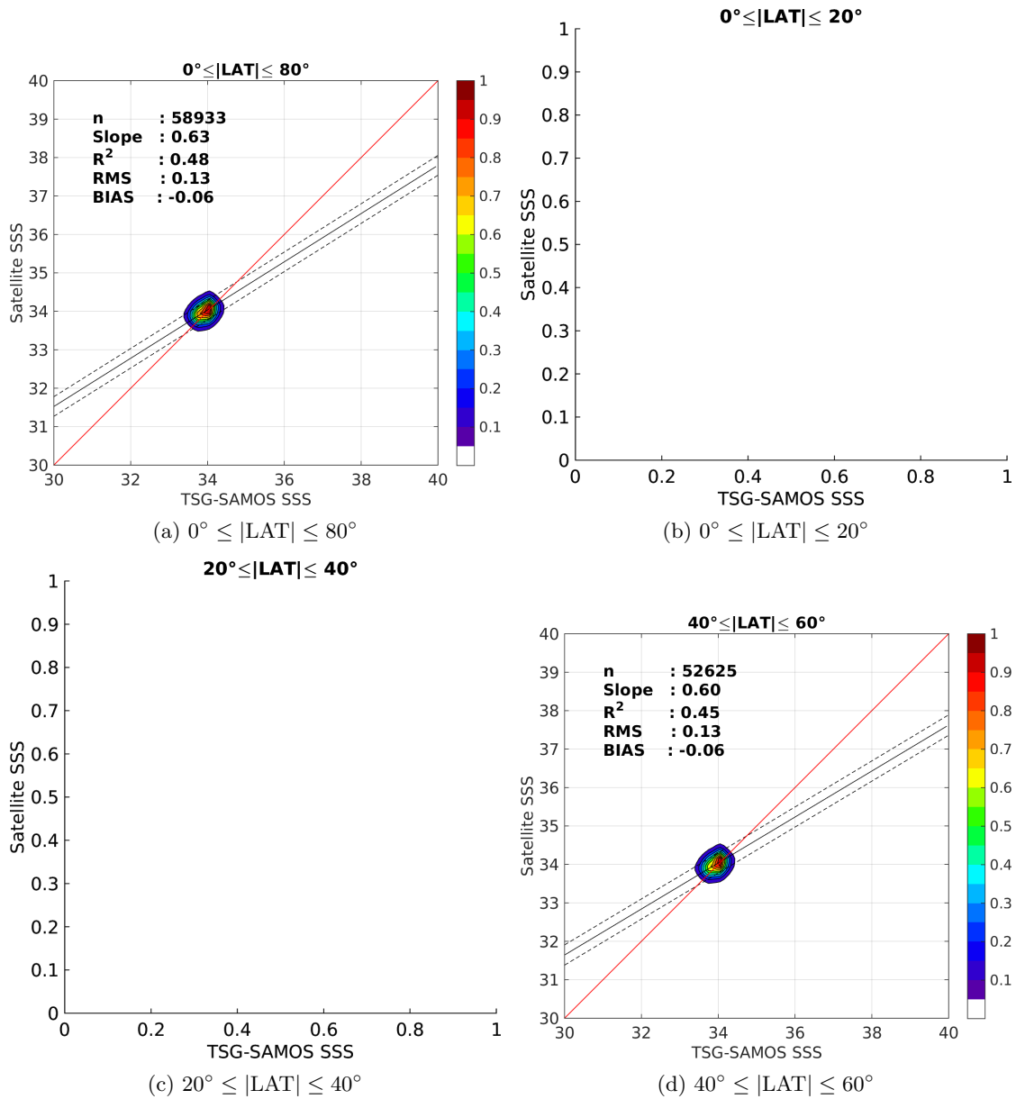
Figure 9: Contour maps of the concentration of Aquarius-L4-IPRC-V4-MONTHLY SSS (y-axis) versus TSG-SAMOS SSS (x-axis) at match-up pairs for different latitude bands. For each plot, the red line shows x=y . The black thin and dashed lines indicate a linear fit through the data cloud and the \pm 95\% confidence levels, respectively. The number match-up pairs n , the slope and R^2 coefficient of the linear fit, the root mean square (RMS) and the mean bias between satellite and in situ data are indicated for each latitude band in each plots.
