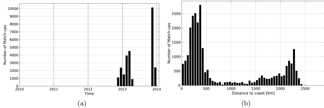
Figure 1: Number of match-ups between TSG-GOSUD-Sailing-ship and Aquarius-L4-IPRC-V4-MONTHLY SSS as a function of time (a) and as function of the distance to coast (b) over the Southern Ocean Pi-MEP region and for the full satellite product period.
