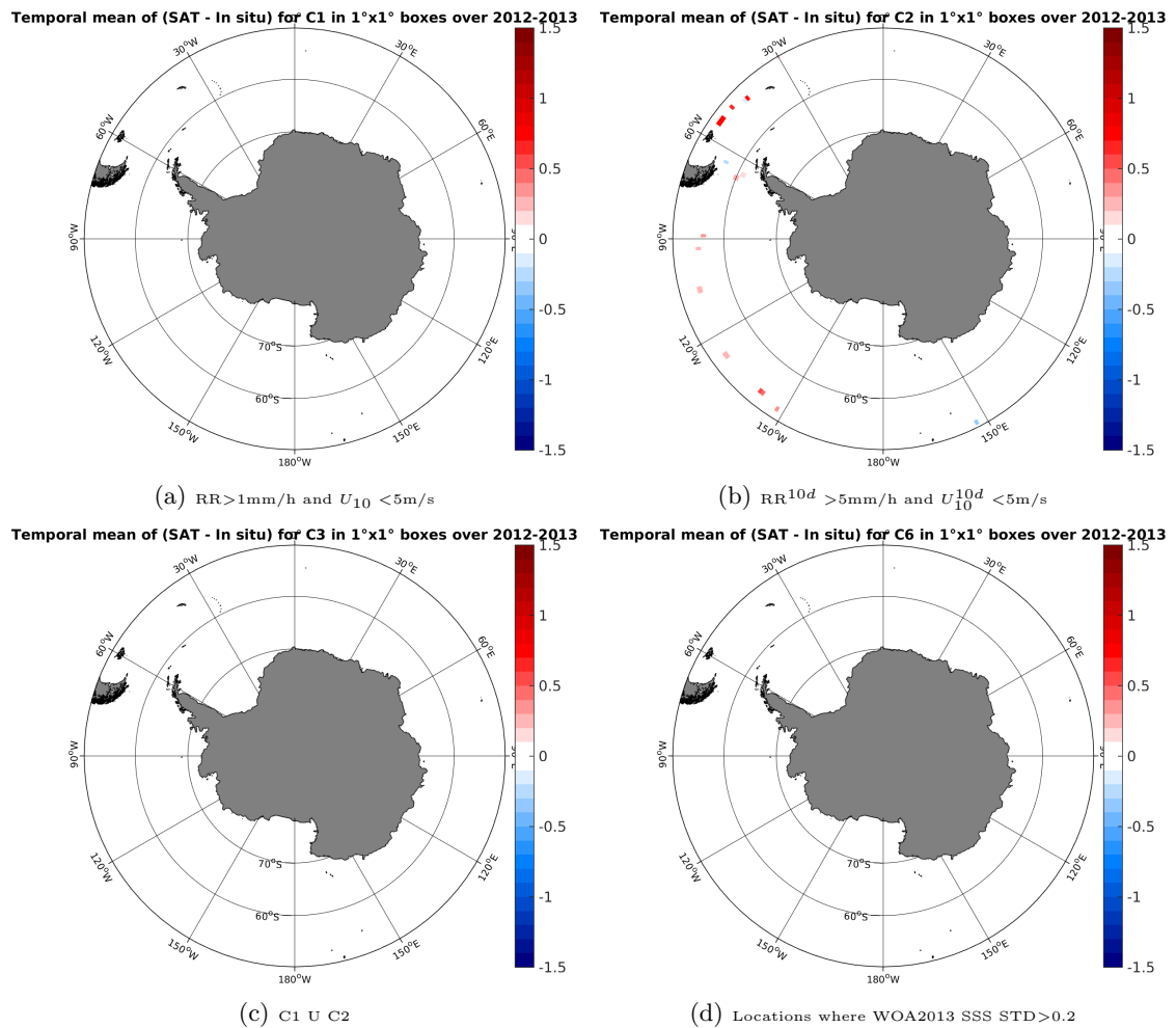
Figure 12: Temporal mean gridded over spatial boxes of size 1^\circ \times 1^\circ of \Delta SSS (Aquarius-L4-IPRC-V4-MONTHLY - TSG-GOSUD-Sailing-ship) for 4 different subdatasets corresponding to: RR > 1\text{mm/h} and U_{10} < 5\text{m/s} (a), RR^{10d} > 5\text{mm/h} and U_{10}^{10d} < 5\text{m/s} (b), C1 U C2 (c), Locations where WOA2013 SSS STD > 0.2 (d).
