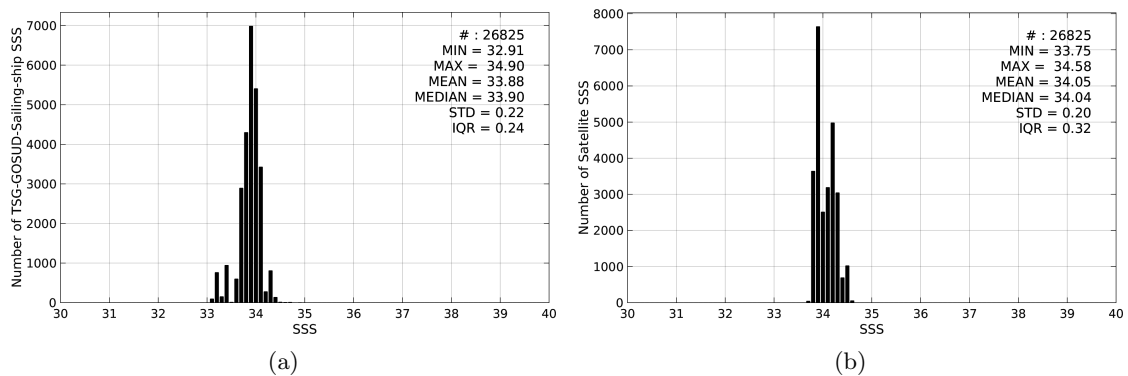
Figure 2: Histograms of SSS from TSG-GOSUD-Sailing-ship (a) and Aquarius-L4-IPRC-V4-MONTHLY (b) considering all match-up pairs per bins of 0.1 over the Southern Ocean Pi-MEP region and for the full satellite product period.
