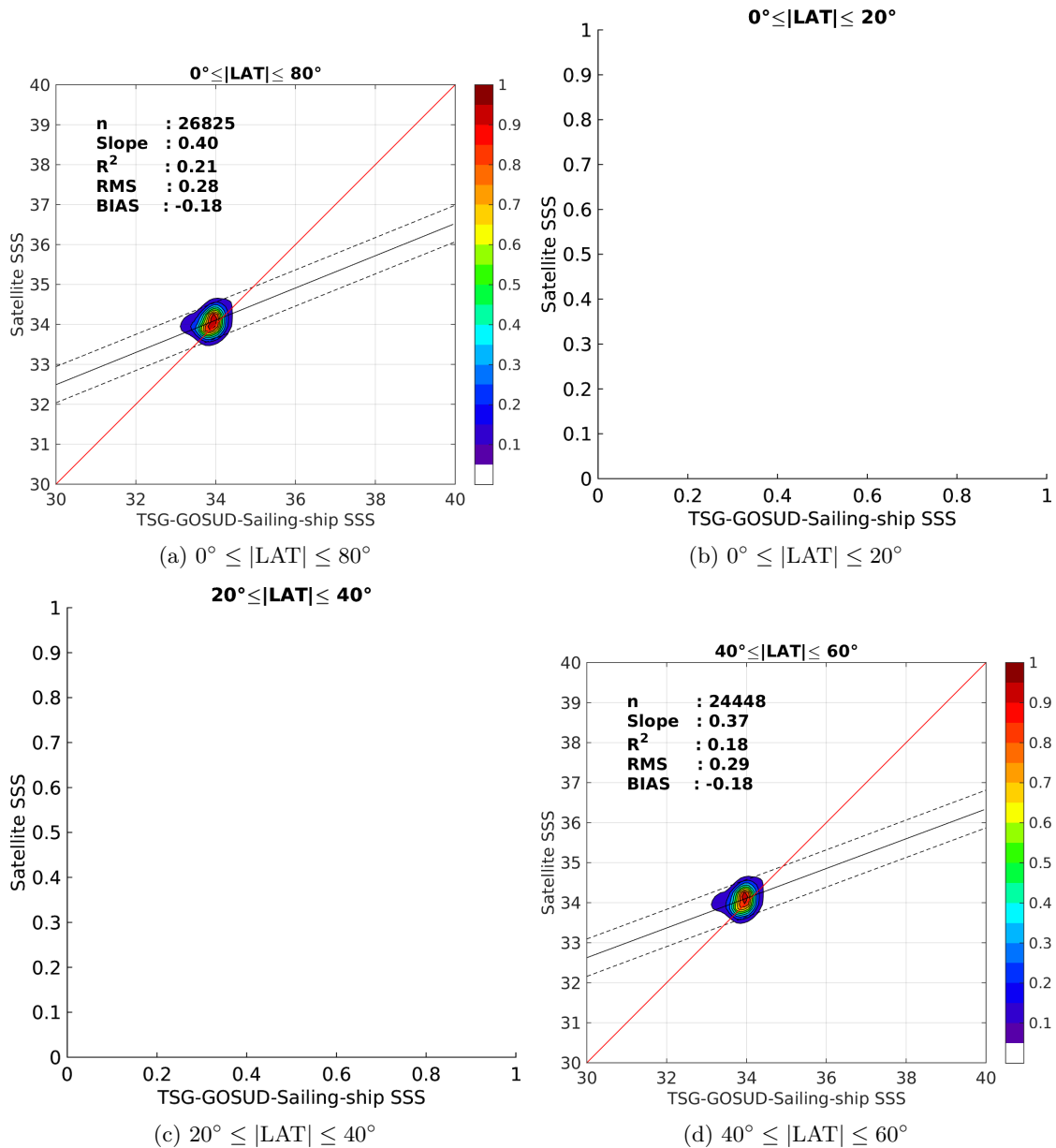
Figure 9: Contour maps of the concentration of Aquarius-L4-IPRC-V4-MONTHLY SSS (y-axis) versus TSG-GOSUD-Sailing-ship SSS (x-axis) at match-up pairs for different latitude bands. For each plot, the red line shows x=y . The black thin and dashed lines indicate a linear fit through the data cloud and the \pm 95\% confidence levels, respectively. The number match-up pairs n , the slope and R^2 coefficient of the linear fit, the root mean square (RMS) and the mean bias between satellite and in situ data are indicated for each latitude band in each plots.
