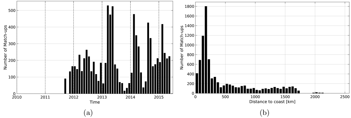
Figure 1: Number of match-ups between Sea mammals and Aquarius-L4-IPRC-V4-MONTHLY SSS as a function of time (a) and as function of the distance to coast (b) over the Southern Ocean Pi-MEP region and for the full satellite product period.
