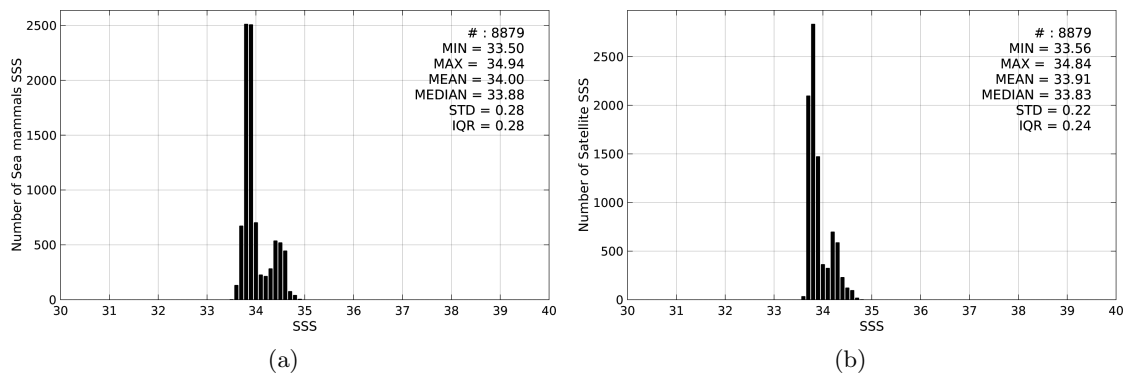
Figure 2: Histograms of SSS from Sea mammals (a) and Aquarius-L4-IPRC-V4-MONTHLY (b) considering all match-up pairs per bins of 0.1 over the Southern Ocean Pi-MEP region and for the full satellite product period.
