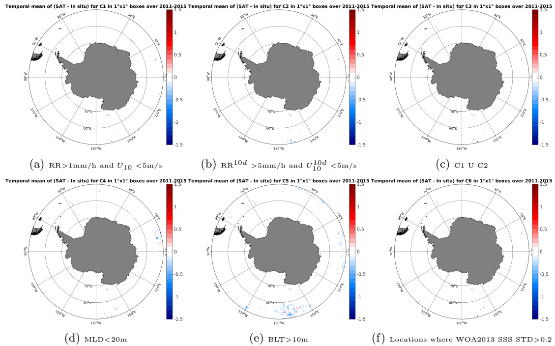
Figure 12: Temporal mean gridded over spatial boxes of size 1°x1° of \Delta SSS (Aquarius-L4-IPRC-V4-MONTHLY - Sea mammals) for 6 different subdatasets corresponding to: RR > 1\text{mm/h} and U_{10} < 5\text{m/s} (a), RR^{10d} > 5\text{mm/h} and U_{10}^{10d} < 5\text{m/s} (b), C1 U C2 (c), MLD < 20\text{m} (d), BLT > 10\text{m} (e), Locations where WOA2013 SSS STD > 0.2 (f).
