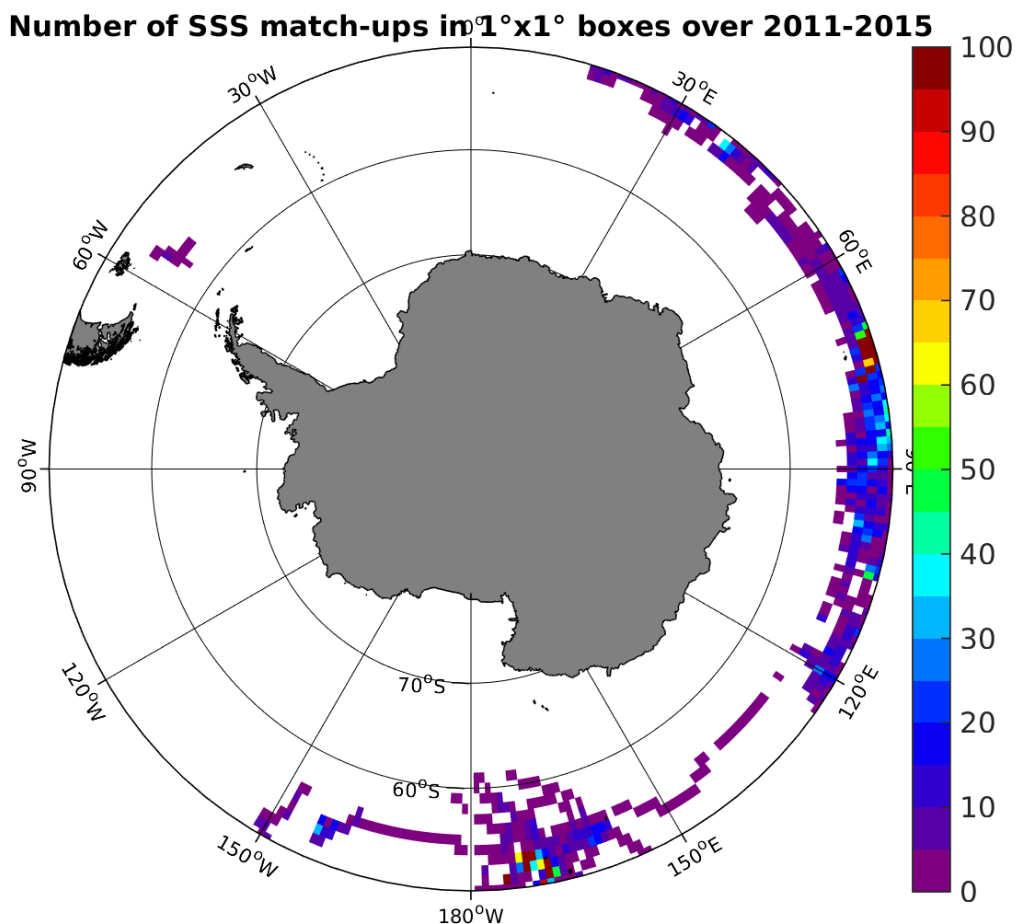
Figure 4: Number of SSS match-ups between Sea mammals SSS and the Aquarius-L4-IPRC-V4-MONTHLY SSS product for the Southern Ocean Pi-MEP region over 1°x1° boxes and for the full satellite product period.
