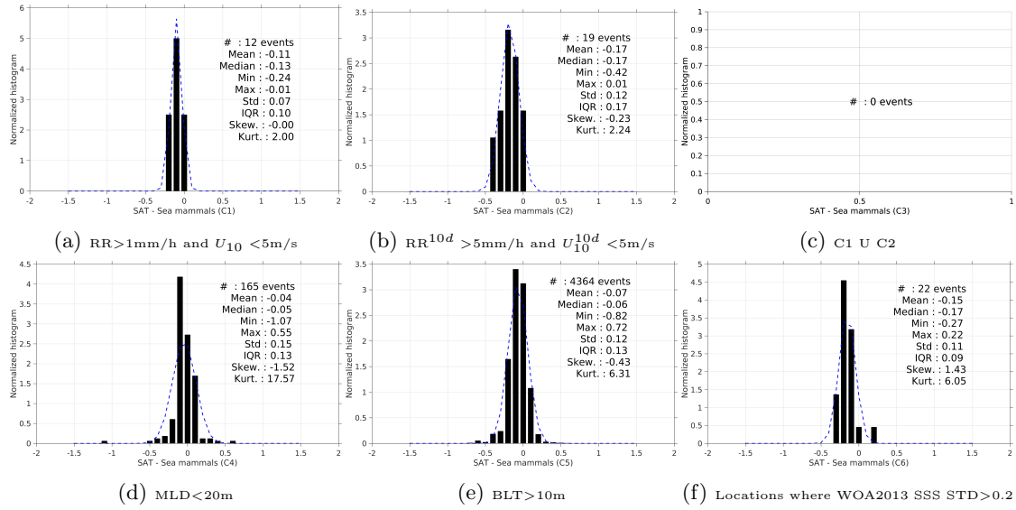
Figure 13: Normalized histogram of \Delta SSS (Aquarius-L4-IPRC-V4-MONTHLY - Sea mammals) for 6 different subdatasets corresponding to: RR > 1mm/h and U_{10} < 5 m/s (a), RR^{10d} > 5 mm/h and U_{10}^{10d} < 5 m/s (b), C1 U C2 (c), MLD < 20m (d), BLT > 10m (e), Locations where WOA2013 SSS STD > 0.2 (f).
