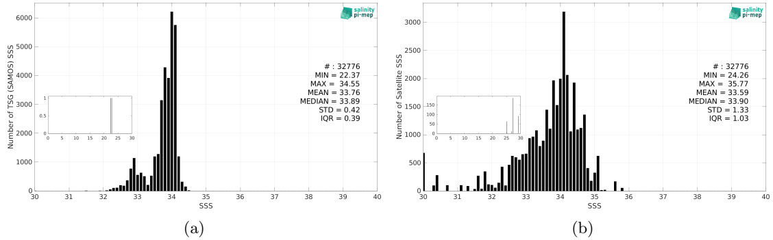
Figure 3: Histograms of SSS from TSG (SAMOS) (a) and Aquarius SSS L3 OR v5 - 7-Day running (NASA-GSFC) (b) considering all match-up pairs per bins of 0.1 over the Southern Ocean Pi-MEP region and for the full satellite product period.
