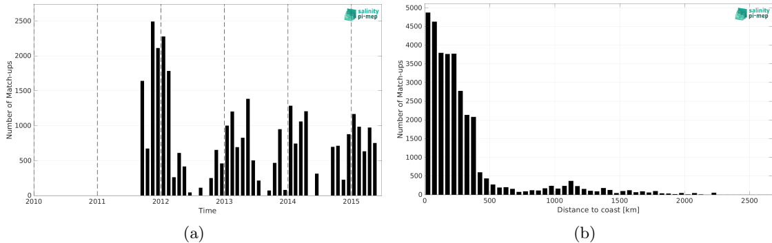
Figure 2: Number of match-ups between TSG (SAMOS) and Aquarius SSS L3 OR v5 - 7-Day running (NASA-GSFC) SSS as a function of time (a) and as function of the distance to coast (b) over the Southern Ocean Pi-MEP region and for the full satellite product period.
