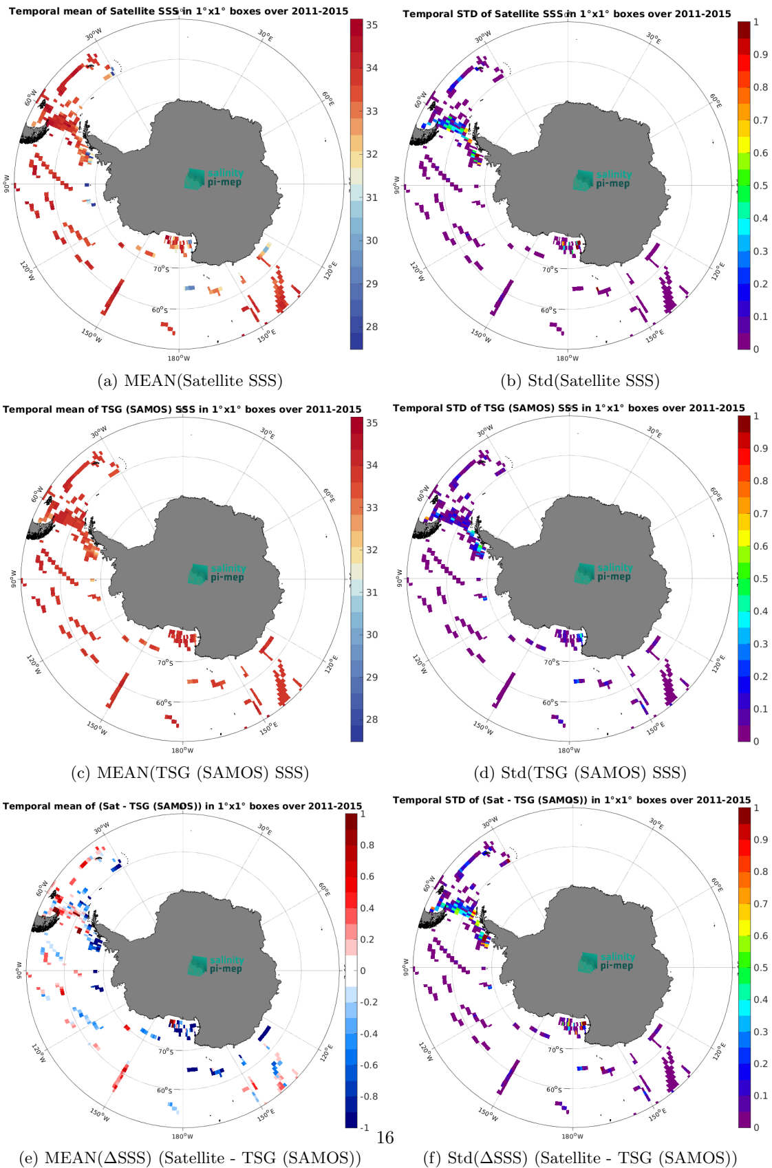
Figure 7: Temporal mean (left) and Std (right) of SSS from Aquarius SSS L3 OR v5 - 7-Day running (NASA-GSFC) (top), TSG (SAMOS) (middle), and of \Delta SSS (Satellite - TSG (SAMOS)). Only match-up pairs are used to generate these maps.
