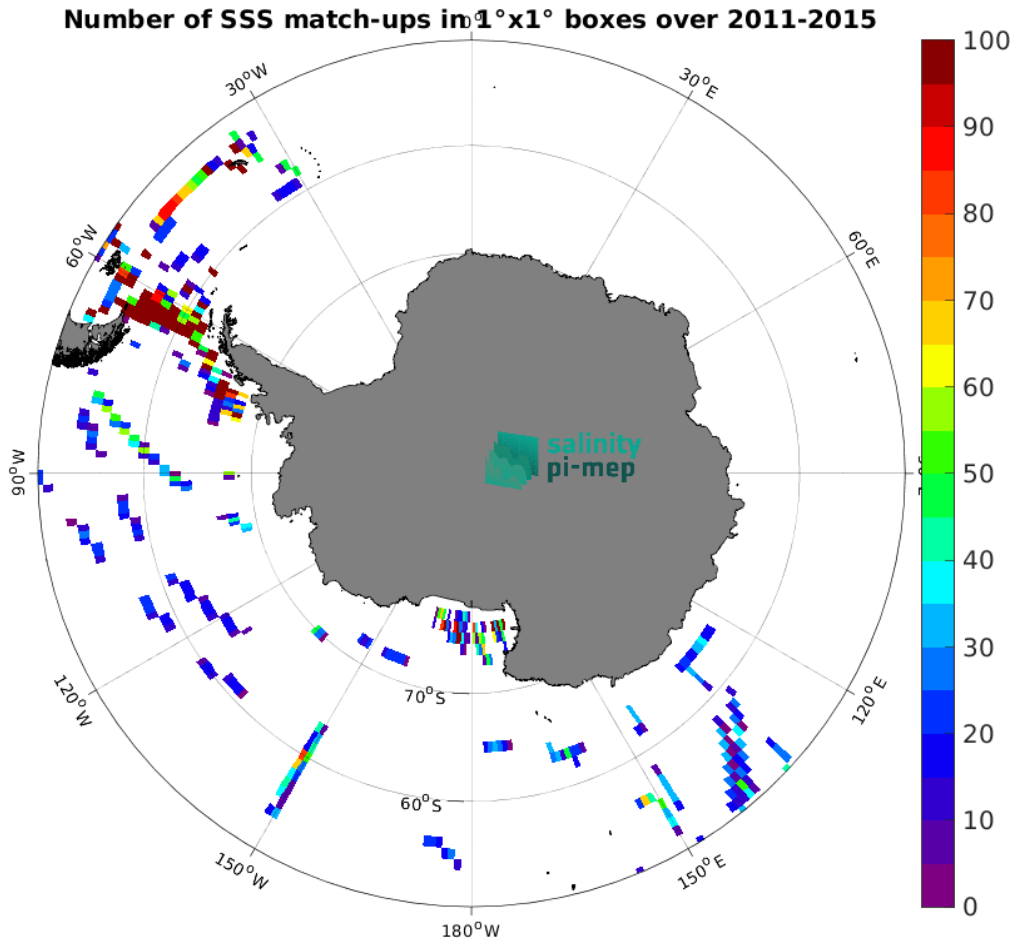
Figure 5: Number of SSS match-ups between TSG (SAMOS) SSS and the Aquarius SSS L3 OR v5 - 7-Day running (NASA-GSFC) SSS product for the Southern Ocean Pi-MEP region over 1^\circ \times 1^\circ boxes and for the full satellite product period.
