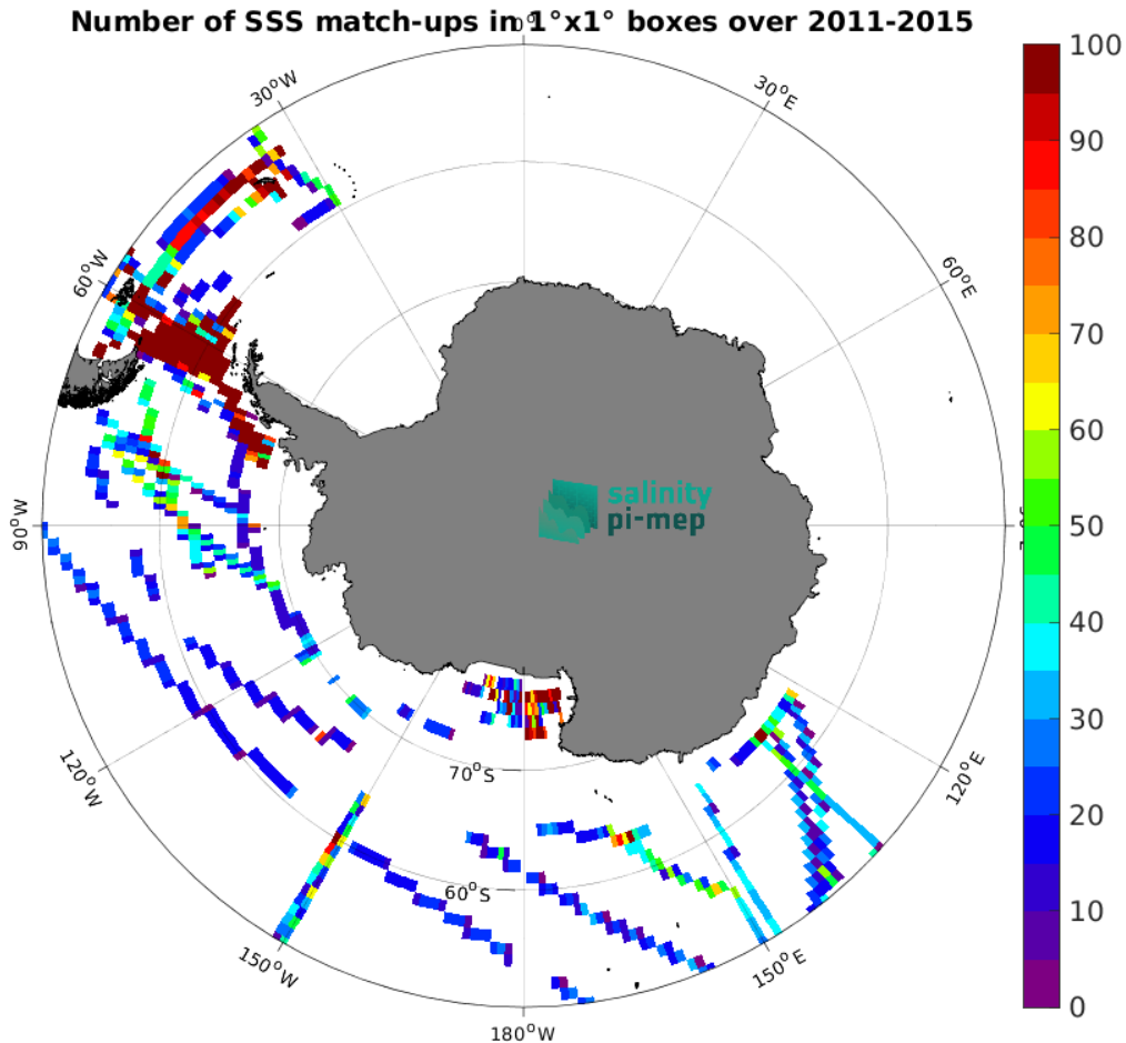
Figure 4: Number of SSS match-ups between TSG (SAMOS) SSS and the Aquarius SSS L3 OR v5 - 7-Day running (NASA-GSFC) SSS product for the Southern Ocean Pi-MEP region over 1^\circ \times 1^\circ boxes and for the full satellite product period.
