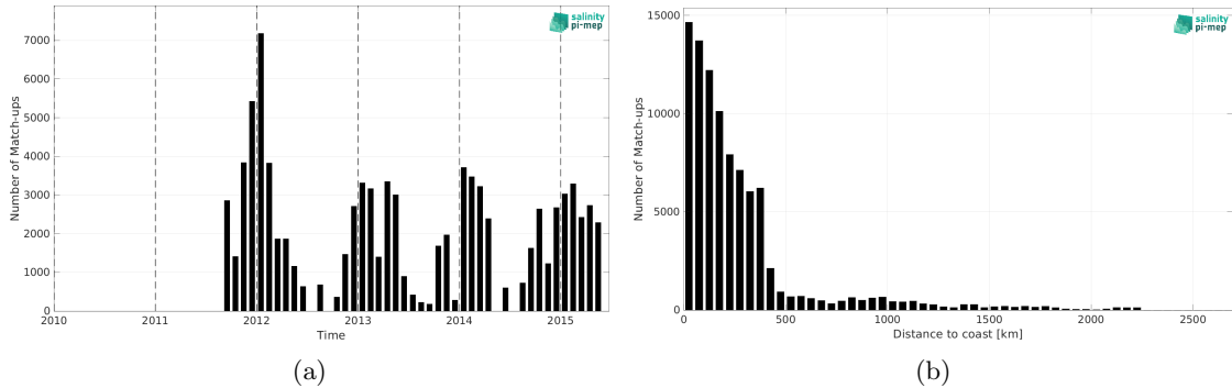
Figure 1: Number of match-ups between TSG (SAMOS) and Aquarius SSS L3 OR v5 - 7-Day running (NASA-GSFC) SSS as a function of time (a) and as function of the distance to coast (b) over the Southern Ocean Pi-MEP region and for the full satellite product period.
