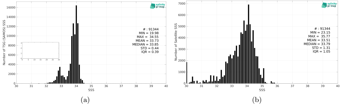
Figure 2: Histograms of SSS from TSG (SAMOS) (a) and Aquarius SSS L3 OR v5 - 7-Day running (NASA-GSFC) (b) considering all match-up pairs per bins of 0.1 over the Southern Ocean Pi-MEP region and for the full satellite product period.
