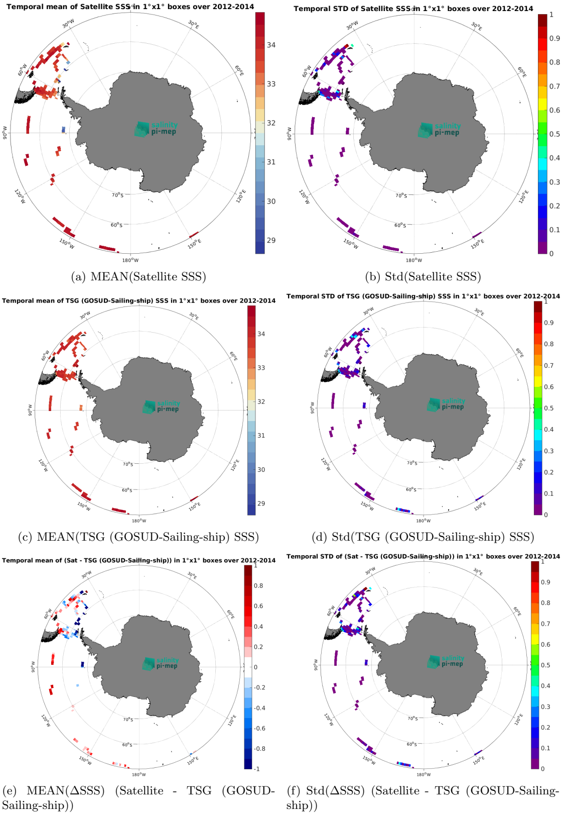
Figure 7: Temporal mean (left) and Std (right) of SSS from Aquarius SSS L3 OR v5 - 7-Day running (NASA-GSFC) (top), TSG (GOSUD-Sailing-ship) (middle), and of \Delta SSS (Satellite - TSG (GOSUD-Sailing-ship)). Only match-up pairs are used to generate these maps.
