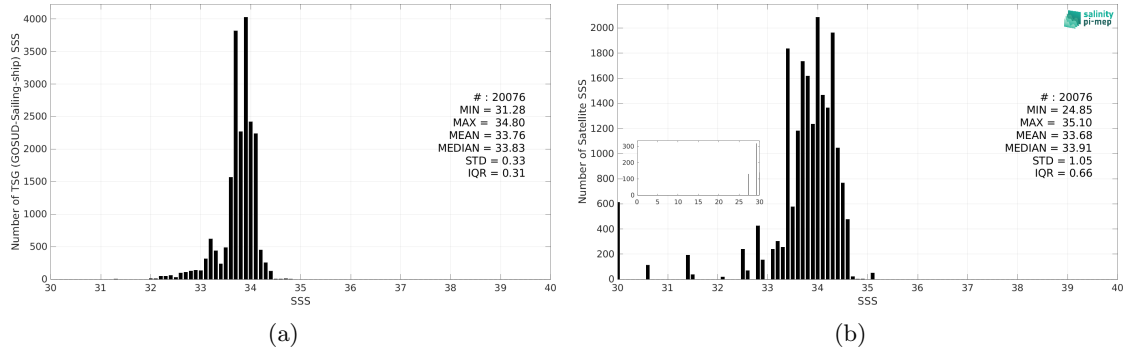
Figure 3: Histograms of SSS from TSG (GOSUD-Sailing-ship) (a) and Aquarius SSS L3 OR v5 - 7-Day running (NASA-GSFC) (b) considering all match-up pairs per bins of 0.1 over the Southern Ocean Pi-MEP region and for the full satellite product period.
