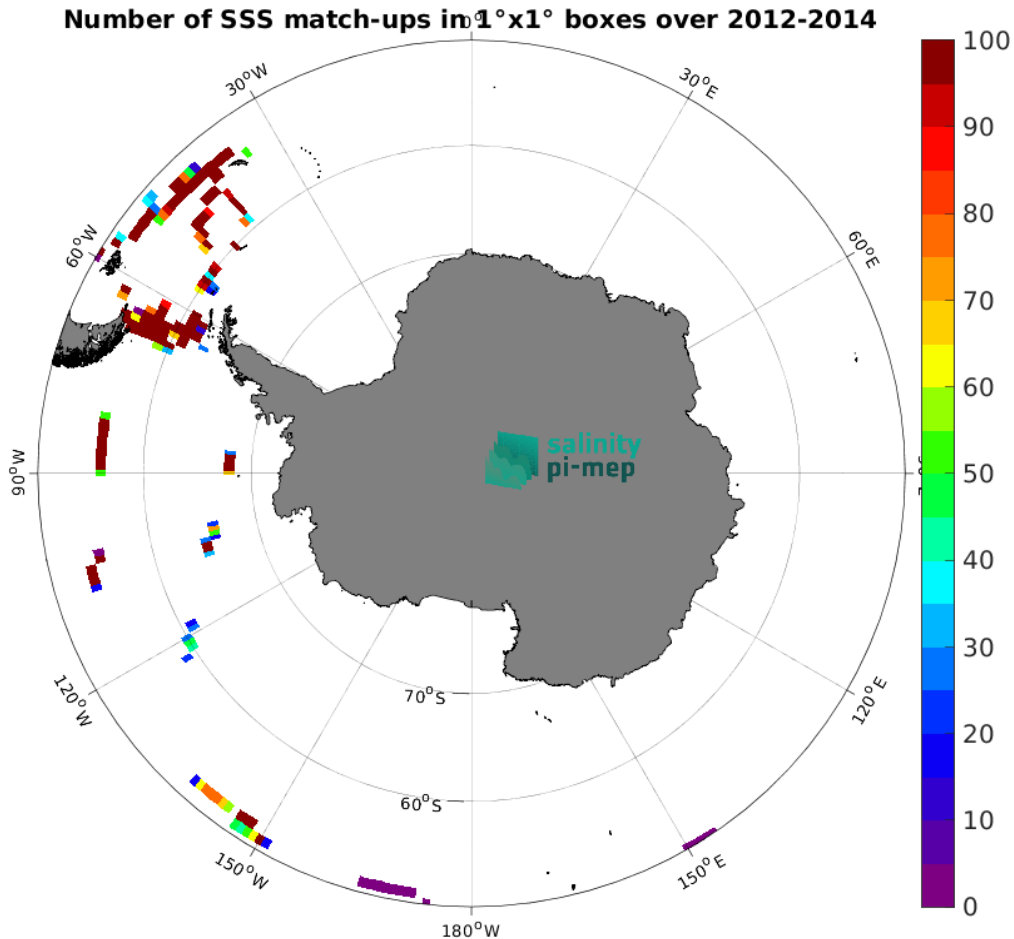
Figure 5: Number of SSS match-ups between TSG (GOSUD-Sailing-ship) SSS and the Aquarius SSS L3 OR v5 - 7-Day running (NASA-GSFC) SSS product for the Southern Ocean Pi-MEP region over 1^\circ \times 1^\circ boxes and for the full satellite product period.
