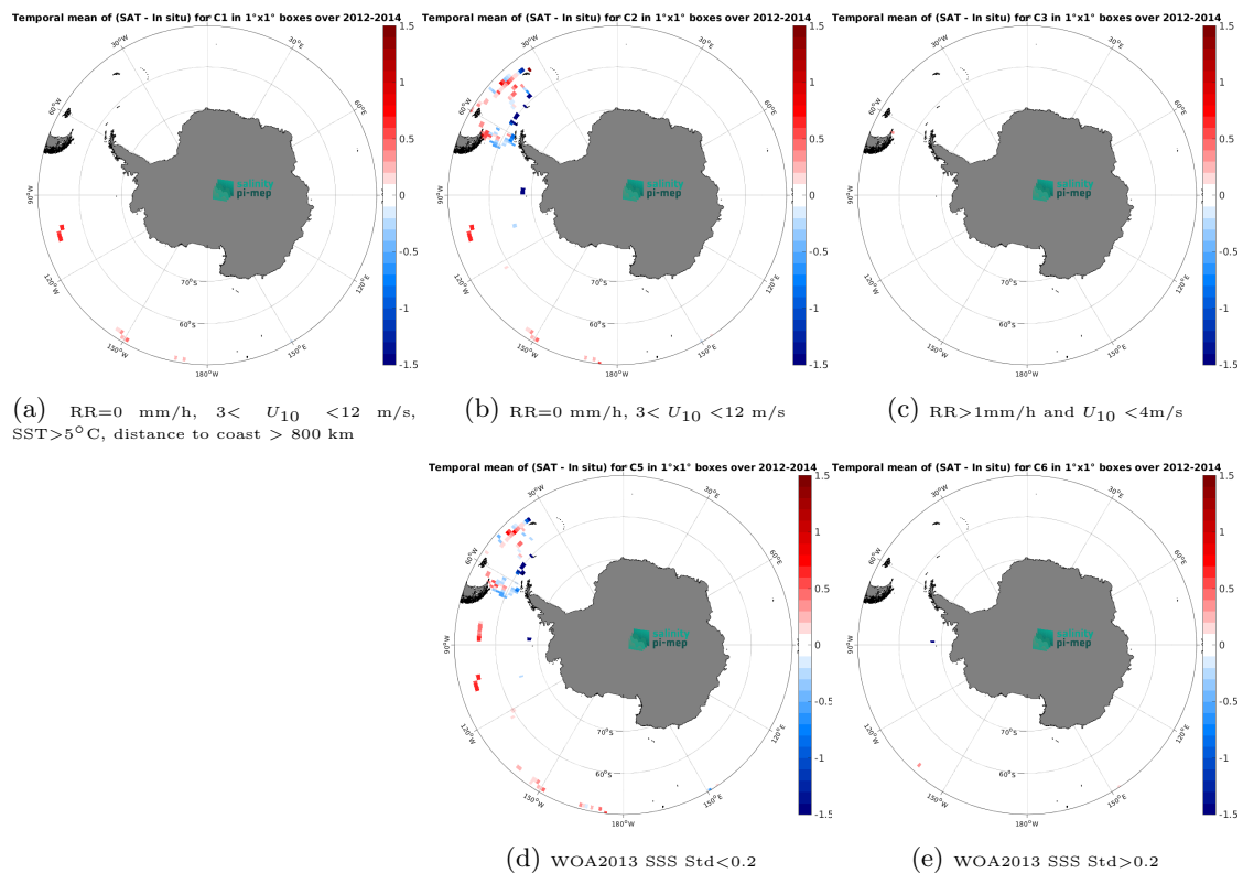
Figure 14: Temporal mean gridded over spatial boxes of size 1^\circ \times 1^\circ of \Delta\text{SSS} (Aquarius SSS L3 OR v5 - 7-Day running (NASA-GSFC) - TSG (GOSUD-Sailing-ship)) for 5 different subdatasets corresponding to:RR=0 mm/h, 3 < U_{10} < 12 m/s, SST>5°C, distance to coast > 800 km (a), RR=0 mm/h, 3 < U_{10} < 12 m/s (b), RR>1mm/h and U_{10} < 4 m/s (c), WOA2013 SSS Std<0.2 (d), WOA2013 SSS Std>0.2 (e).
