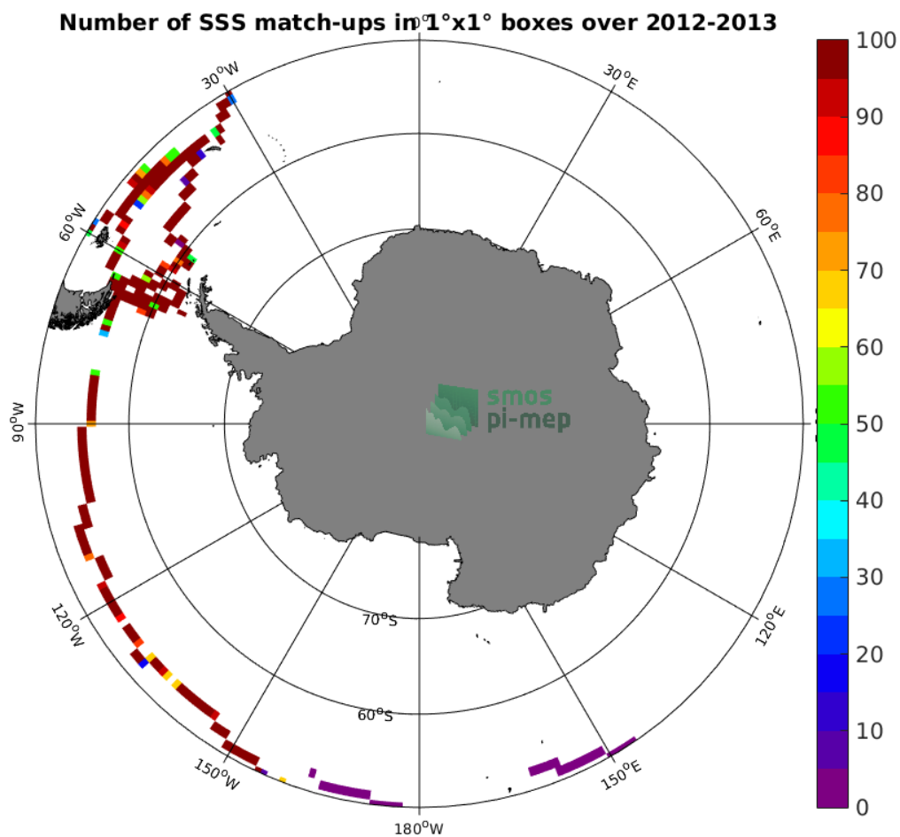
Figure 4: Number of SSS match-ups between TSG-GOSUD-Sailing-ship SSS and the Aquarius-L3-OR-V5-7DAY-RUNNING-1DEG SSS product for the Southern Ocean Pi-MEP region over 1^\circ \times 1^\circ boxes and for the full satellite product period.
