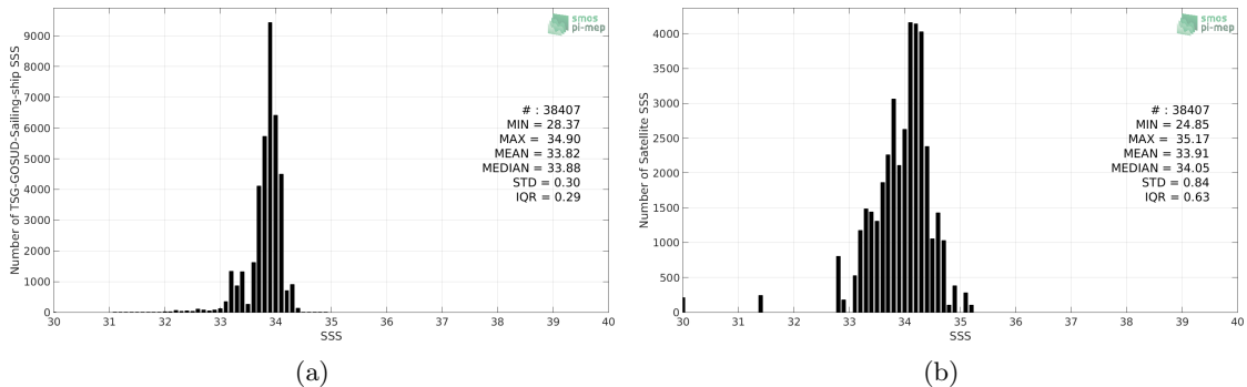
Figure 2: Histograms of SSS from TSG-GOSUD-Sailing-ship (a) and Aquarius-L3-OR-V5-7DAY-RUNNING-1DEG (b) considering all match-up pairs per bins of 0.1 over the Southern Ocean Pi-MEP region and for the full satellite product period.
