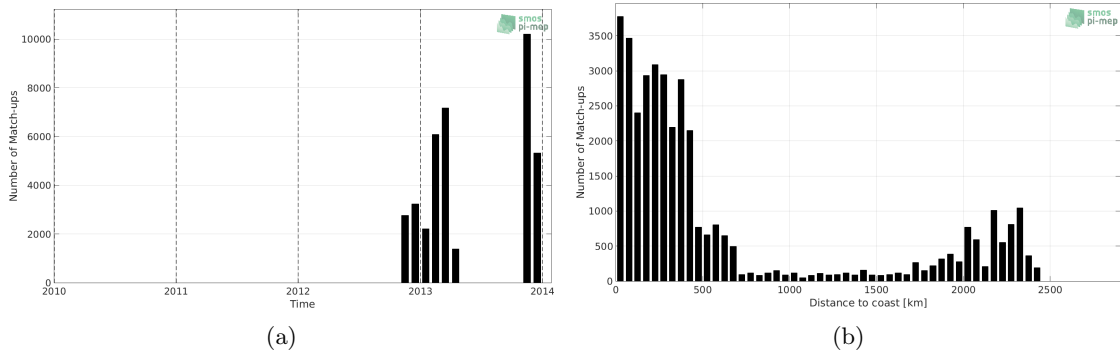
Figure 1: Number of match-ups between TSG-GOSUD-Sailing-ship and Aquarius-L3-OR-V5-7DAY-RUNNING-1DEG SSS as a function of time (a) and as function of the distance to coast (b) over the Southern Ocean Pi-MEP region and for the full satellite product period.
