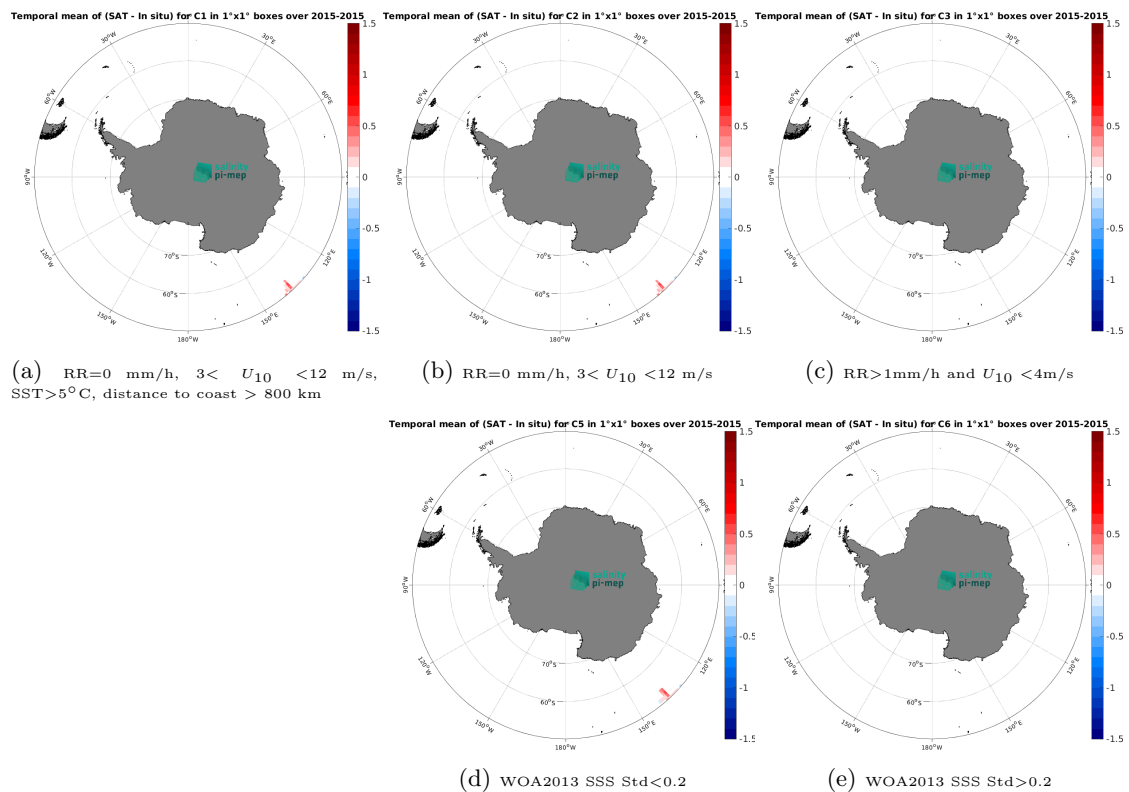
Figure 14: Temporal mean gridded over spatial boxes of size 1^\circ \times 1^\circ of \Delta\text{SSS} (Aquarius SSS L3 OR v5 - 7-Day running (NASA-GSFC) - TSG (GOSUD-Research-vessel)) for 5 different subdatasets corresponding to:RR=0 mm/h, 3 < U_{10} < 12 m/s, SST>5°C, distance to coast > 800 km (a), RR=0 mm/h, 3 < U_{10} < 12 m/s (b), RR>1mm/h and U_{10} < 4 m/s (c), WOA2013 SSS Std<0.2 (d), WOA2013 SSS Std>0.2 (e).
