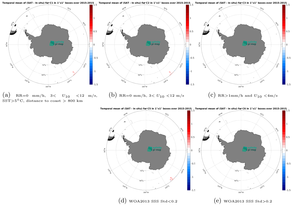
Figure 12: Temporal mean gridded over spatial boxes of size 1°×1° of \Delta SSS (Aquarius SSS L3 OR v5 - 7-Day running (NASA-GSFC) - TSG (GOSUD-Research-vessel)) for 5 different subdatasets corresponding to:RR=0 mm/h, 3 < U_{10} < 12 m/s, SST>5°C, distance to coast > 800 km (a), RR=0 mm/h, 3 < U_{10} < 12 m/s (b), RR>1mm/h and U_{10} < 4 m/s (c), WOA2013 SSS Std<0.2 (d), WOA2013 SSS Std>0.2 (e).
