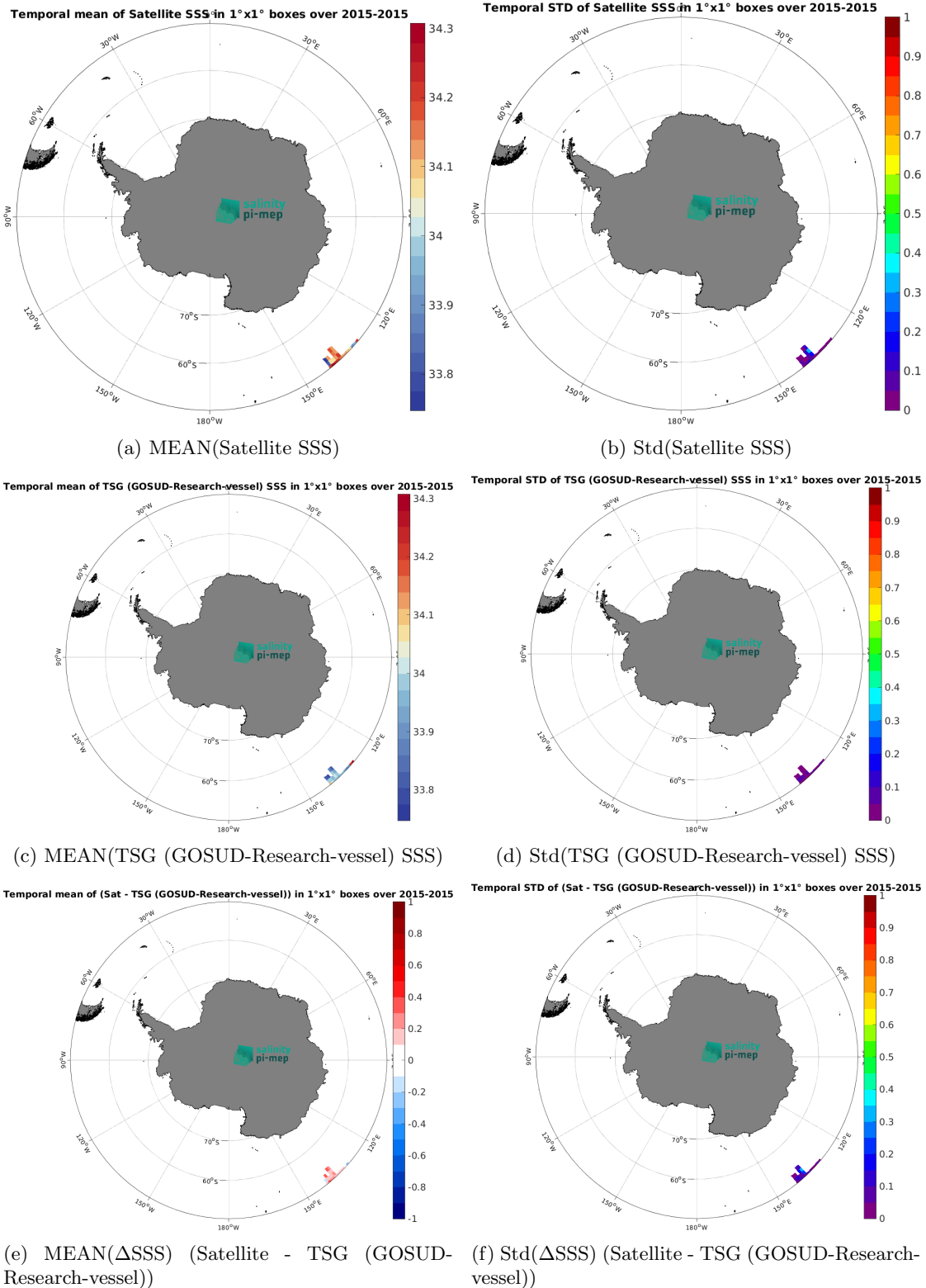
Figure 6: Temporal mean (left) and Std (right) of SSS from Aquarius SSS L3 OR v5 - 7-Day running (NASA-GSFC) (top), TSG (GOSUD-Research-vessel) (middle), and of \Delta SSS (Satellite - TSG (GOSUD-Research-vessel)). Only match-up pairs are used to generate these maps.
