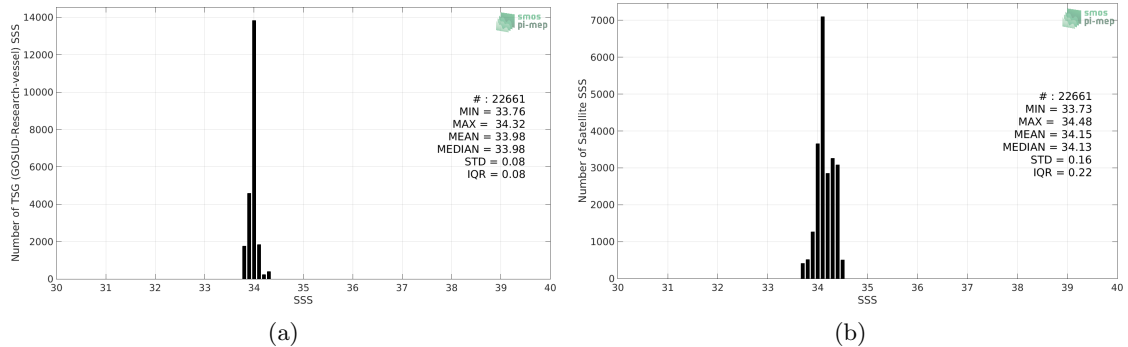
Figure 2: Histograms of SSS from TSG (GOSUD-Research-vessel) (a) and Aquarius SSS L3 OR v5 - 7-Day running (NASA-GSFC) (b) considering all match-up pairs per bins of 0.1 over the Southern Ocean Pi-MEP region and for the full satellite product period.
