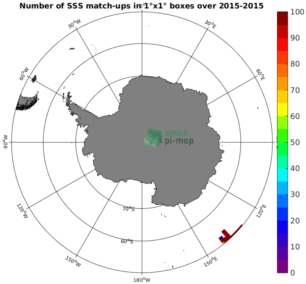
Figure 4: Number of SSS match-ups between TSG-GOSUD-Research-vessel SSS and the Aquarius-L3-OR-V5-7DAY-RUNNING-1DEG SSS product for the Southern Ocean Pi-MEP region over 1°x1° boxes and for the full satellite product period.
