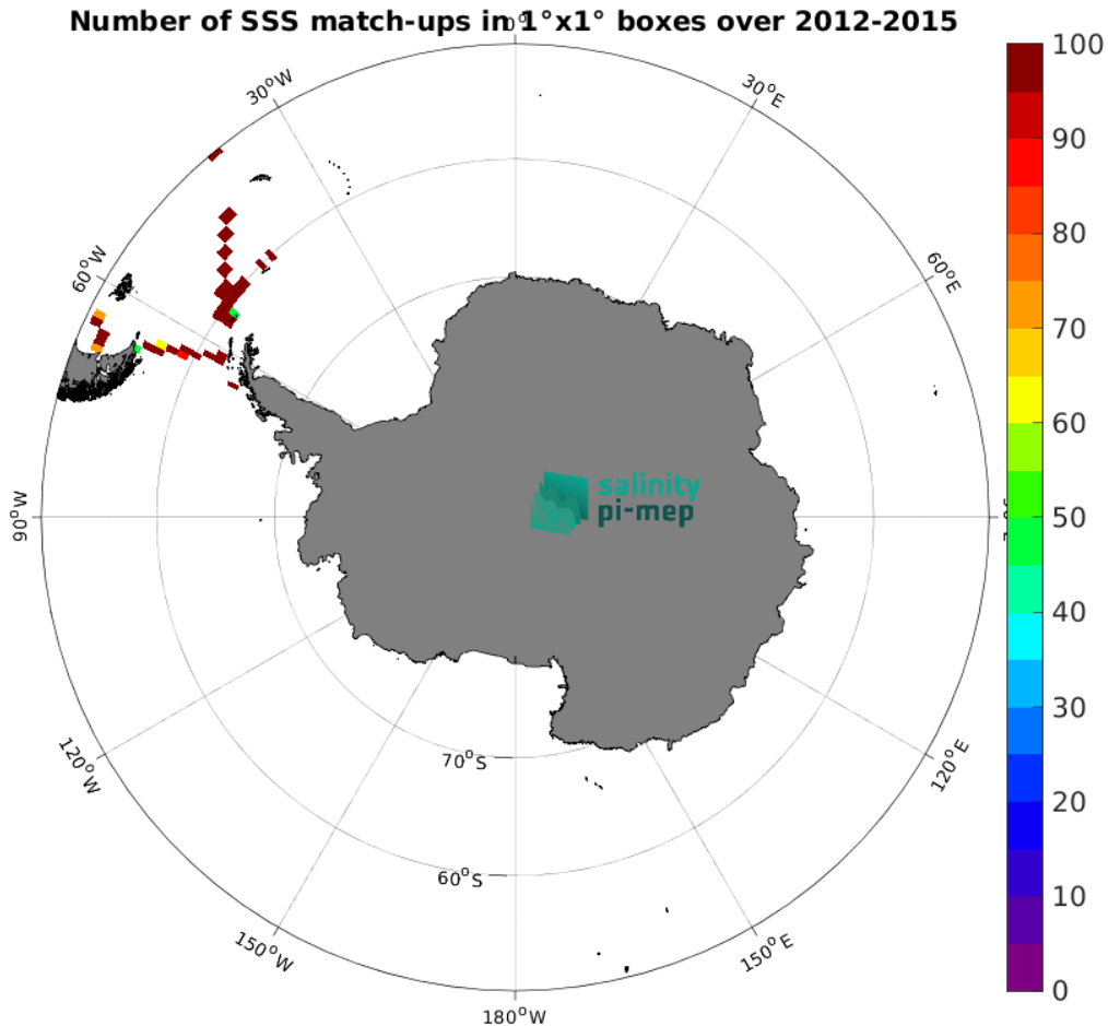
Figure 5: Number of SSS match-ups between TSG (CSIC-UTM) SSS and the Aquarius SSS L3 OR v5 - 7-Day running (NASA-GSFC) SSS product for the Southern Ocean Pi-MEP region over 1^\circ \times 1^\circ boxes and for the full satellite product period.
