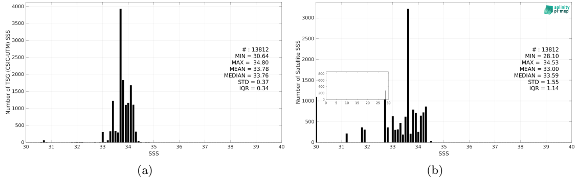
Figure 3: Histograms of SSS from TSG (CSIC-UTM) (a) and Aquarius SSS L3 OR v5 - 7-Day running (NASA-GSFC) (b) considering all match-up pairs per bins of 0.1 over the Southern Ocean Pi-MEP region and for the full satellite product period.
