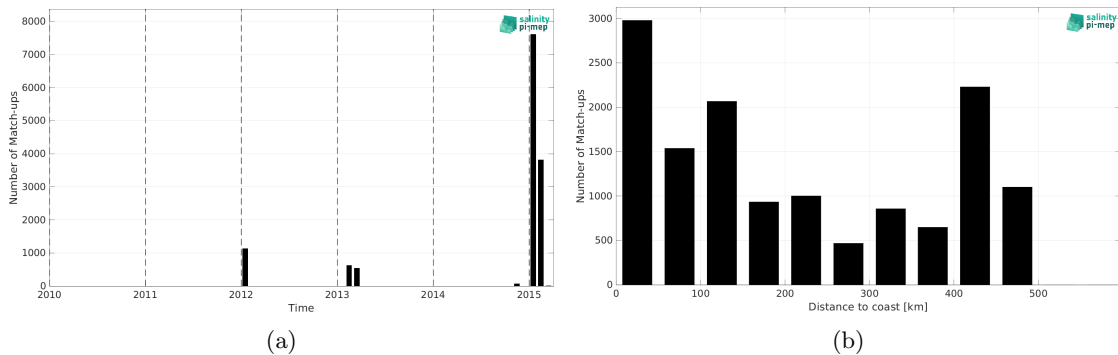
Figure 2: Number of match-ups between TSG (CSIC-UTM) and Aquarius SSS L3 OR v5 - 7-Day running (NASA-GSFC) SSS as a function of time (a) and as function of the distance to coast (b) over the Southern Ocean Pi-MEP region and for the full satellite product period.
