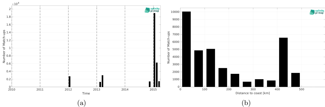
Figure 1: Number of match-ups between TSG (CSIC-UTM) and Aquarius SSS L3 OR v5 - 7-Day running (NASA-GSFC) SSS as a function of time (a) and as function of the distance to coast (b) over the Southern Ocean Pi-MEP region and for the full satellite product period.
