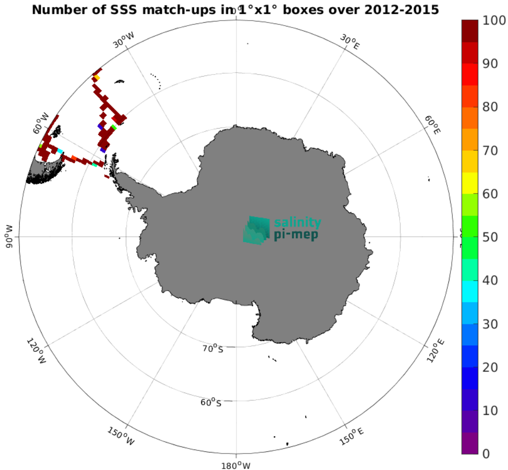
Figure 4: Number of SSS match-ups between TSG (CSIC-UTM) SSS and the Aquarius SSS L3 OR v5 - 7-Day running (NASA-GSFC) SSS product for the Southern Ocean Pi-MEP region over 1^\circ \times 1^\circ boxes and for the full satellite product period.
