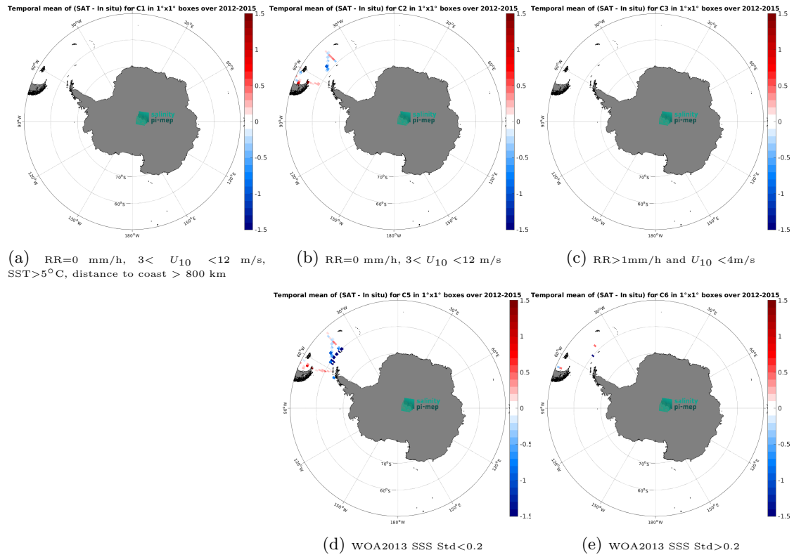
Figure 12: Temporal mean gridded over spatial boxes of size 1^{\circ}\times 1^{\circ} of \Delta\text{SSS} (Aquarius SSS L3 OR v5 - 7-Day running (NASA-GSFC) - TSG (CSIC-UTM)) for 5 different subdatasets corresponding to:RR=0 mm/h, 3 < U_{10} < 12 m/s, SST >5^{\circ}\text{C} , distance to coast > 800 km (a), RR=0 mm/h, 3 < U_{10} < 12 m/s (b), RR >1 mm/h and U_{10} < 4 m/s (c), WOA2013 SSS Std <0.2 (d), WOA2013 SSS Std >0.2 (e).
