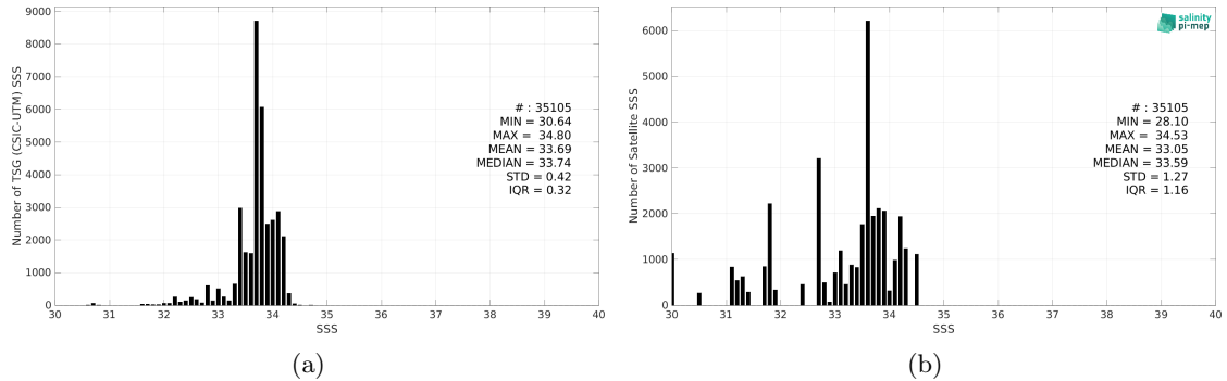
Figure 2: Histograms of SSS from TSG (CSIC-UTM) (a) and Aquarius SSS L3 OR v5 - 7-Day running (NASA-GSFC) (b) considering all match-up pairs per bins of 0.1 over the Southern Ocean Pi-MEP region and for the full satellite product period.
