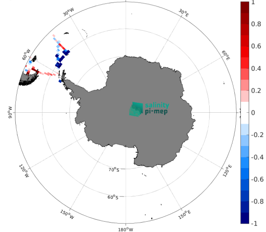
(e) MEAN( \Delta SSS) (Satellite - TSG (CSIC-UTM)) 16
