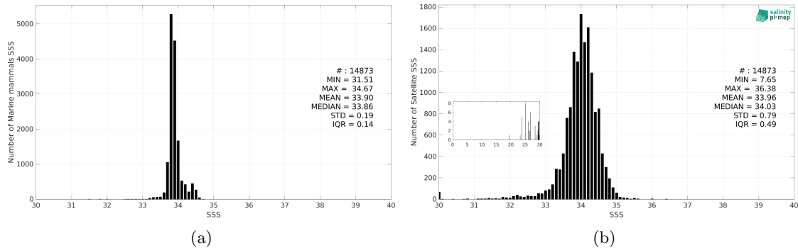
Figure 3: Histograms of SSS from Marine mammals (a) and Aquarius SSS L3 OR v5 - 7-Day running (NASA-GSFC) (b) considering all match-up pairs per bins of 0.1 over the Southern Ocean Pi-MEP region and for the full satellite product period.
