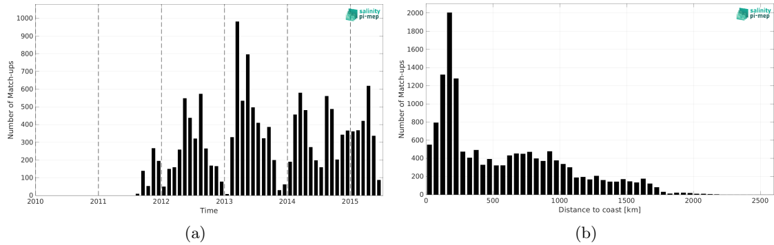
Figure 2: Number of match-ups between Marine mammals and Aquarius SSS L3 OR v5 - 7-Day running (NASA-GSFC) SSS as a function of time (a) and as function of the distance to coast (b) over the Southern Ocean Pi-MEP region and for the full satellite product period.
