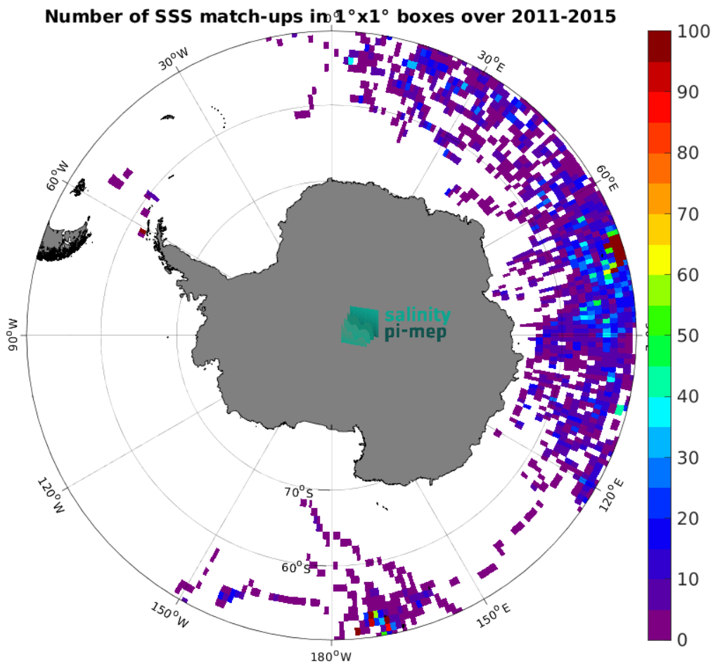
Figure 5: Number of SSS match-ups between Marine mammals SSS and the Aquarius SSS L3 OR v5 - 7-Day running (NASA-GSFC) SSS product for the Southern Ocean Pi-MEP region over 1^\circ \times 1^\circ boxes and for the full satellite product period.
