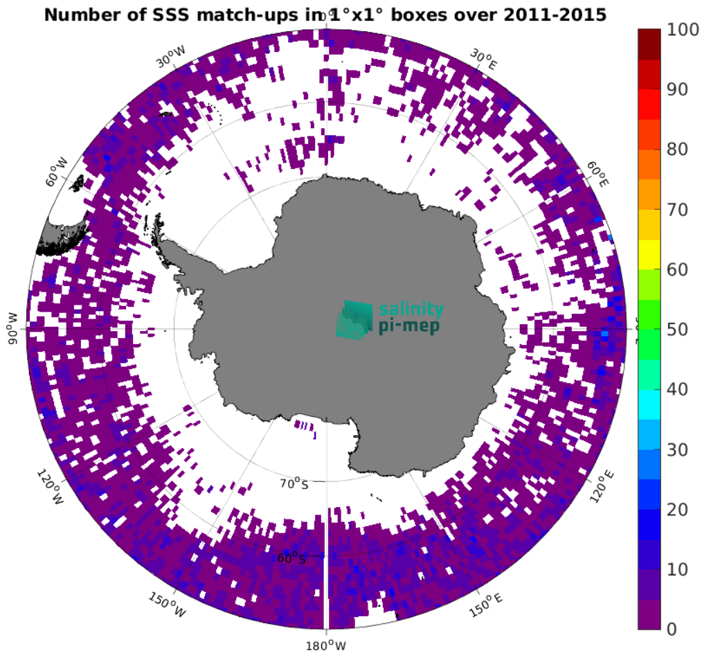
Figure 5: Number of SSS match-ups between Argo SSS and the Aquarius SSS L3 OR v5 - 7-Day running (NASA-GSFC) SSS product for the Southern Ocean Pi-MEP region over 1^\circ \times 1^\circ boxes and for the full satellite product period.
