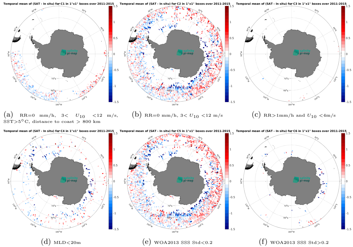
Figure 14: Temporal mean gridded over spatial boxes of size 1^\circ \times 1^\circ of \Delta SSS (Aquarius SSS L3 OR v5 - 7-Day running (NASA-GSFC) - Argo) for 6 different subdatasets corresponding to:RR=0 mm/h, 3 < U_{10} < 12 m/s, SST>5°C, distance to coast > 800 km (a), RR=0 mm/h, 3 < U_{10} < 12 m/s (b), RR>1mm/h and U_{10} < 4 m/s (c),MLD<20m (d),WOA2013 SSS Std<0.2 (e),WOA2013 SSS Std>0.2 (f).
