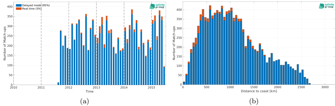
Figure 2: Number of match-ups between Argo and Aquarius SSS L3 OR v5 - 7-Day running (NASA-GSFC) SSS as a function of time (a) and as function of the distance to coast (b) over the Southern Ocean Pi-MEP region and for the full satellite product period.
