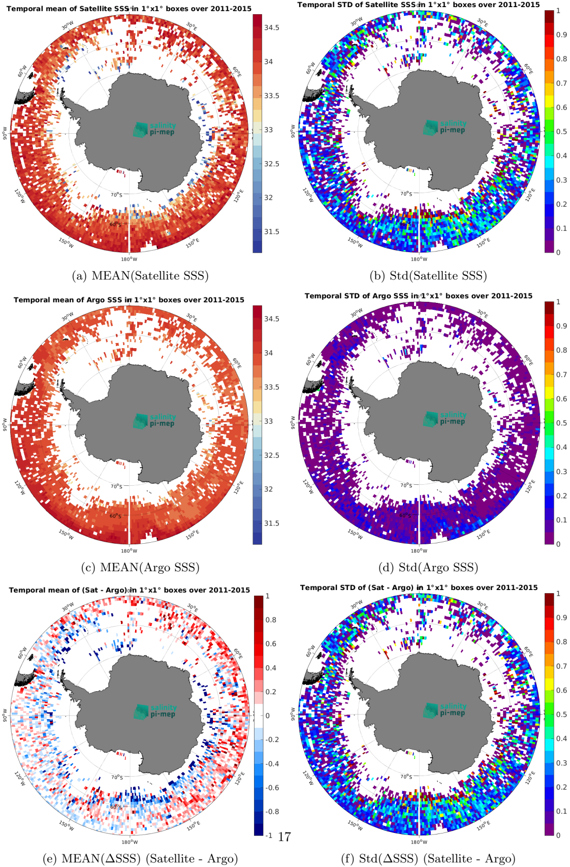
Figure 7: Temporal mean (left) and Std (right) of SSS from Aquarius SSS L3 OR v5 - 7-Day running (NASA-GSFC) (top), Argo (middle), and of \Delta SSS (Satellite - Argo). Only match-up pairs are used to generate these maps.
