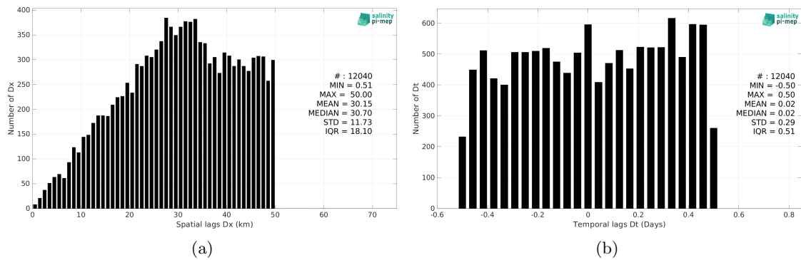
Figure 6: Histograms of the spatial (a) and temporal (b) lags between the location/time of the Argo measurement and the date of the corresponding Aquarius SSS L3 OR v5 - 7-Day running (NASA-GSFC) SSS pixel.
