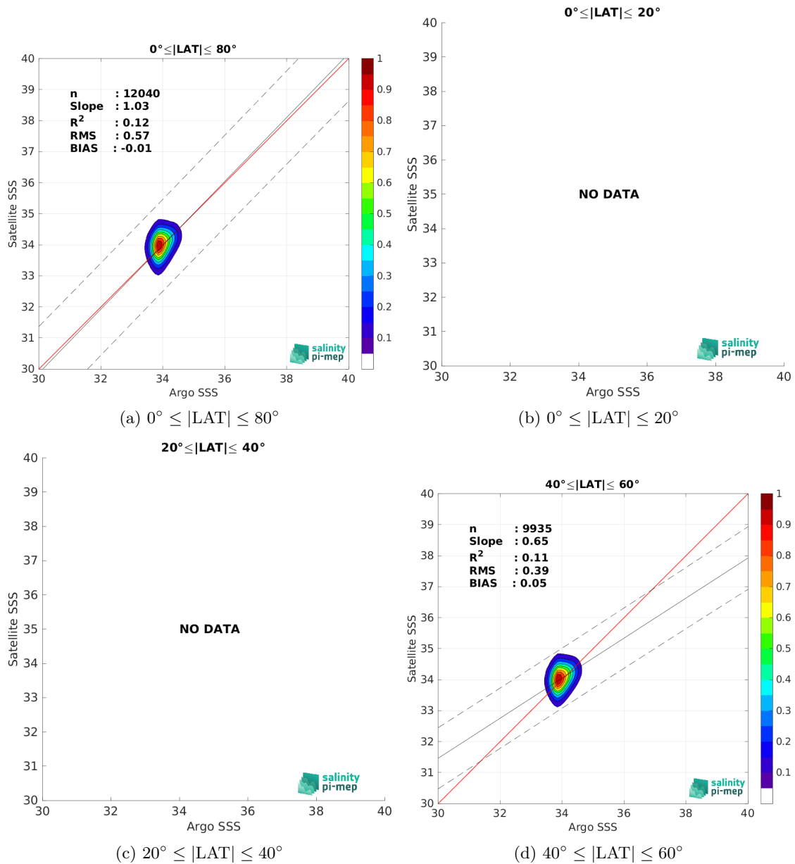
Figure 10: Contour maps of the concentration of Aquarius SSS L3 OR v5 - 7-Day running (NASA-GSFC) SSS (y-axis) versus Argo SSS (x-axis) at match-up pairs for different latitude bands. For each plot, the red line shows x=y . The black thin and dashed lines indicate a linear fit through the data cloud and the \pm 95\% confidence levels, respectively. The number match-up pairs n , the slope and R^2 coefficient of the linear fit, the root mean square (RMS) and the mean bias between satellite and in situ data are indicated for each latitude band in each plots.
