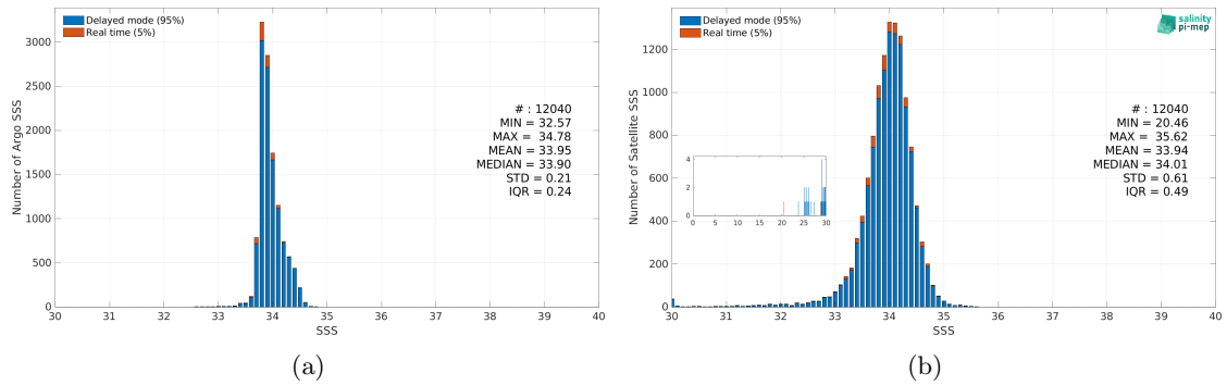
Figure 3: Histograms of SSS from Argo (a) and Aquarius SSS L3 OR v5 - 7-Day running (NASA-GSFC) (b) considering all match-up pairs per bins of 0.1 over the Southern Ocean Pi-MEP region and for the full satellite product period.
