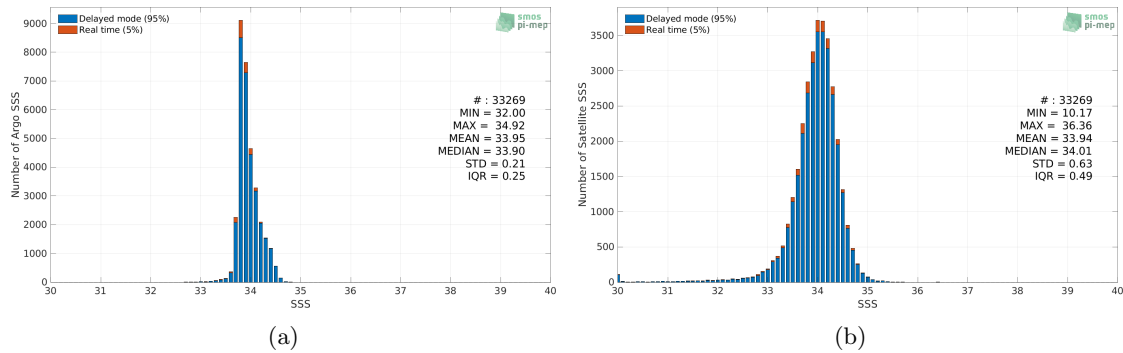
Figure 2: Histograms of SSS from Argo (a) and Aquarius SSS L3 OR v5 - 7-Day running (NASA-GSFC) (b) considering all match-up pairs per bins of 0.1 over the Southern Ocean Pi-MEP region and for the full satellite product period.
