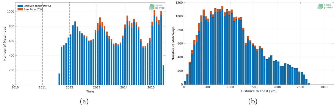
Figure 1: Number of match-ups between Argo and Aquarius SSS L3 OR v5 - 7-Day running (NASA-GSFC) SSS as a function of time (a) and as function of the distance to coast (b) over the Southern Ocean Pi-MEP region and for the full satellite product period.
