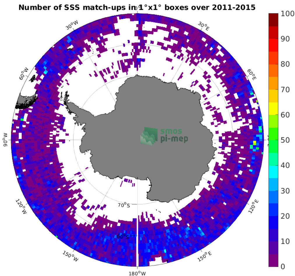
Figure 4: Number of SSS match-ups between Argo SSS and the Aquarius SSS L3 OR v5 - 7-Day running (NASA-GSFC) SSS product for the Southern Ocean Pi-MEP region over 1^\circ \times 1^\circ boxes and for the full satellite product period.
