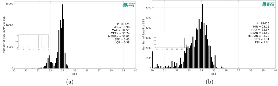
Figure 3: Histograms of SSS from TSG (SAMOS) (a) and Aquarius SSS L3 OR v5 - 7-Day running - Rain mask (NASA-GSFC) (b) considering all match-up pairs per bins of 0.1 over the Southern Ocean Pi-MEP region and for the full satellite product period.
