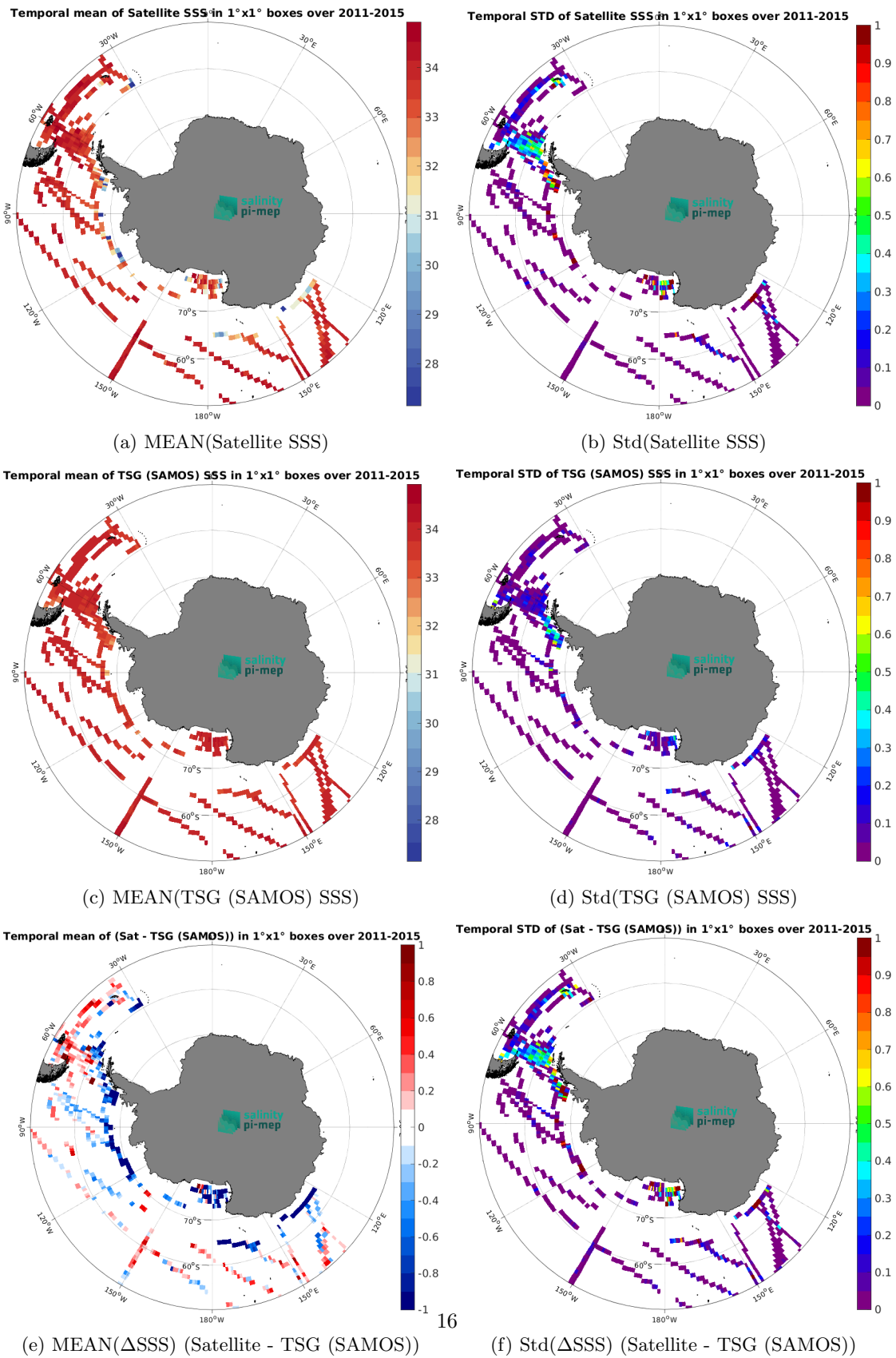
Figure 7: Temporal mean (left) and Std (right) of SSS from Aquarius SSS L3 OR v5 - 7-Day running - Rain mask (NASA-GSFC) (top), TSG (SAMOS) (middle), and of \Delta SSS (Satellite - TSG (SAMOS)). Only match-up pairs are used to generate these maps.
