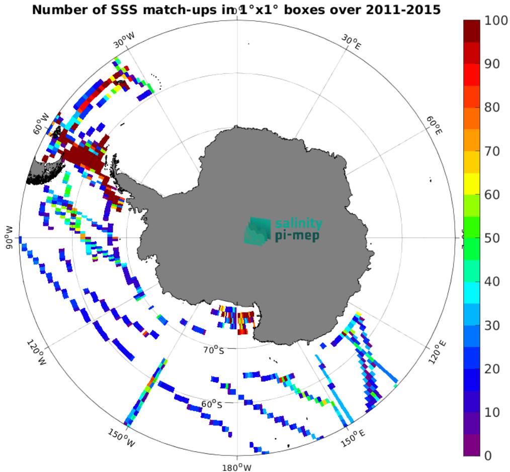
Figure 5: Number of SSS match-ups between TSG (SAMOS) SSS and the Aquarius SSS L3 OR v5 - 7-Day running - Rain mask (NASA-GSFC) SSS product for the Southern Ocean Pi-MEP region over 1^\circ \times 1^\circ boxes and for the full satellite product period.
