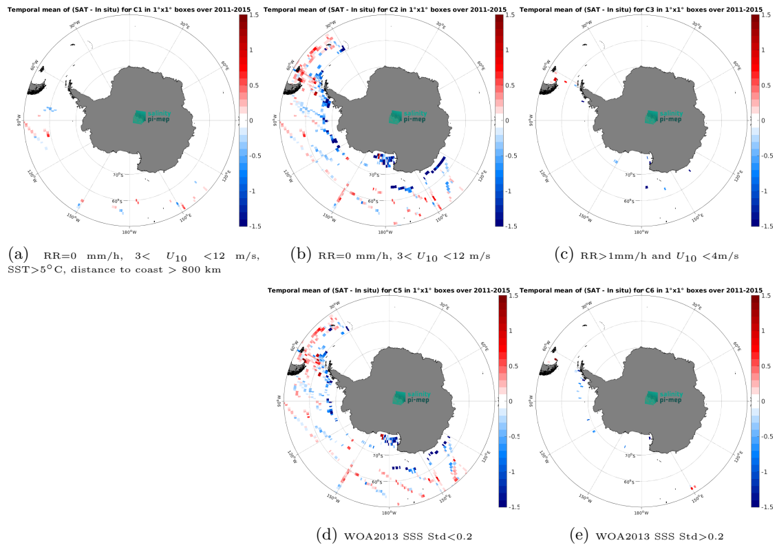
Figure 14: Temporal mean gridded over spatial boxes of size 1^\circ \times 1^\circ of \Delta SSS (Aquarius SSS L3 OR v5 - 7-Day running - Rain mask (NASA-GSFC) - TSG (SAMOS)) for 5 different subdatasets corresponding to:RR=0 mm/h, 3 < U_{10} < 12 m/s, SST >5^\circ\text{C} , distance to coast > 800 km (a), RR=0 mm/h, 3 < U_{10} < 12 m/s (b), RR >1 mm/h and U_{10} < 4 m/s (c), WOA2013 SSS Std <0.2 (d), WOA2013 SSS Std >0.2 (e).
