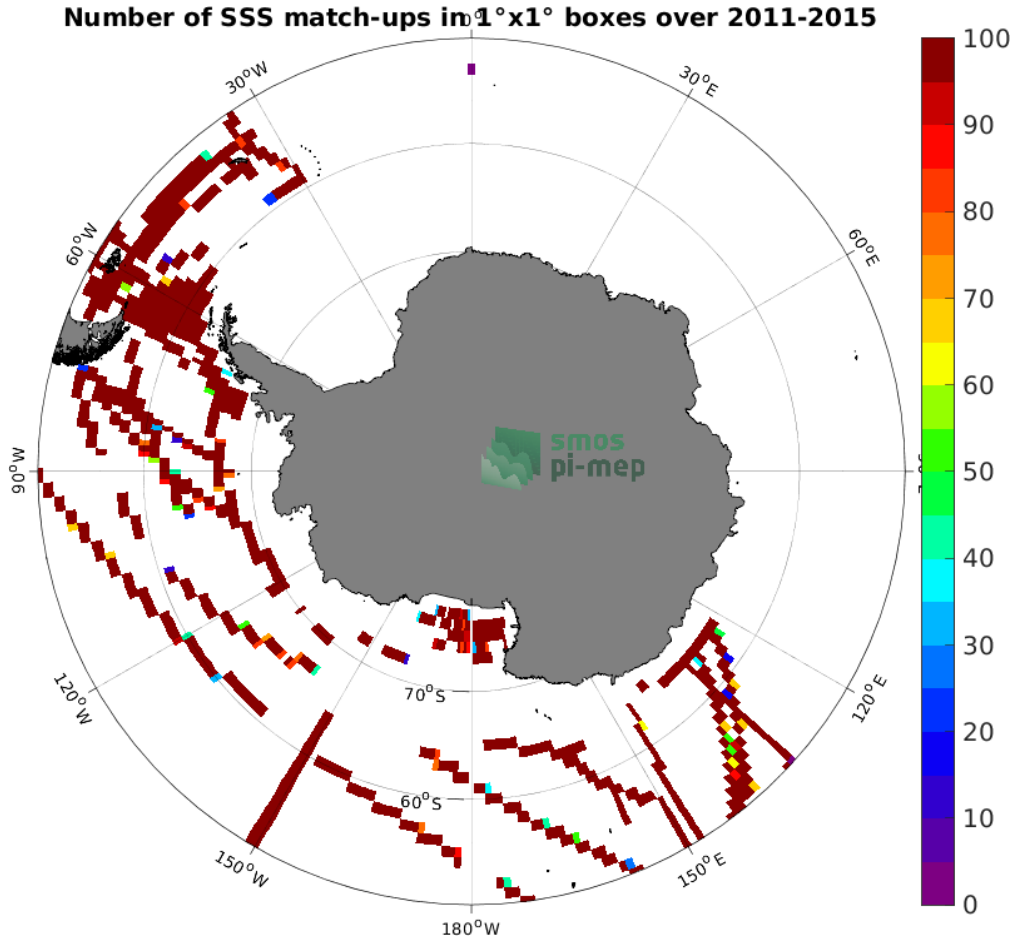
Figure 4: Number of SSS match-ups between TSG (SAMOS) SSS and the Aquarius SSS L3 OR v5 - 7-Day running - Rain mask (NASA-GSFC) SSS product for the Southern Ocean Pi-MEP region over 1^\circ \times 1^\circ boxes and for the full satellite product period.
