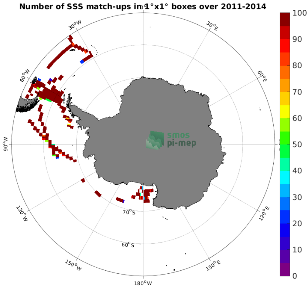
Figure 4: Number of SSS match-ups between TSG (SAMOS) SSS and the Aquarius SSS L3 OR v5 - 7-Day running - Rain mask (NASA-GSFC) SSS product for the Southern Ocean Pi-MEP region over 1^\circ \times 1^\circ boxes and for the full satellite product period.
