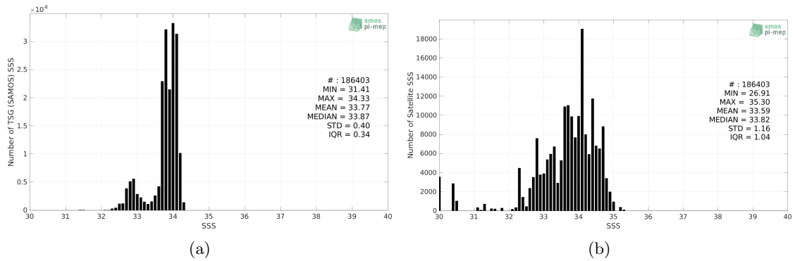
Figure 2: Histograms of SSS from TSG (SAMOS) (a) and Aquarius SSS L3 OR v5 - 7-Day running - Rain mask (NASA-GSFC) (b) considering all match-up pairs per bins of 0.1 over the Southern Ocean Pi-MEP region and for the full satellite product period.
