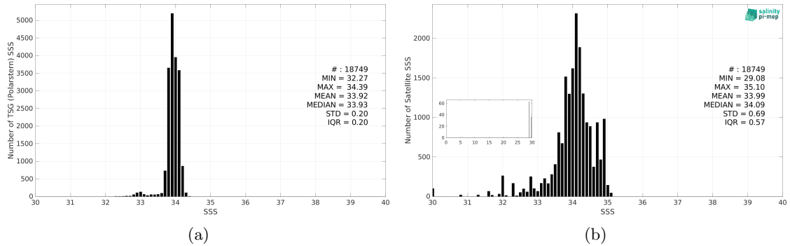
Figure 3: Histograms of SSS from TSG (Polarstern) (a) and Aquarius SSS L3 OR v5 - 7-Day running - Rain mask (NASA-GSFC) (b) considering all match-up pairs per bins of 0.1 over the Southern Ocean Pi-MEP region and for the full satellite product period.
