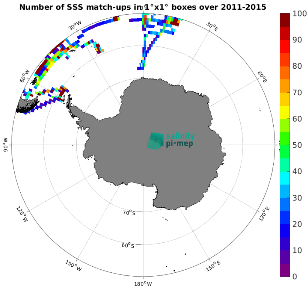
Figure 5: Number of SSS match-ups between TSG (Polarstern) SSS and the Aquarius SSS L3 OR v5 - 7-Day running - Rain mask (NASA-GSFC) SSS product for the Southern Ocean Pi-MEP region over 1^\circ \times 1^\circ boxes and for the full satellite product period.
