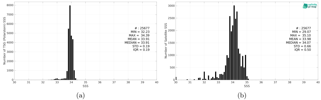
Figure 2: Histograms of SSS from TSG (Polarstern) (a) and Aquarius SSS L3 OR v5 - 7-Day running - Rain mask (NASA-GSFC) (b) considering all match-up pairs per bins of 0.1 over the Southern Ocean Pi-MEP region and for the full satellite product period.
