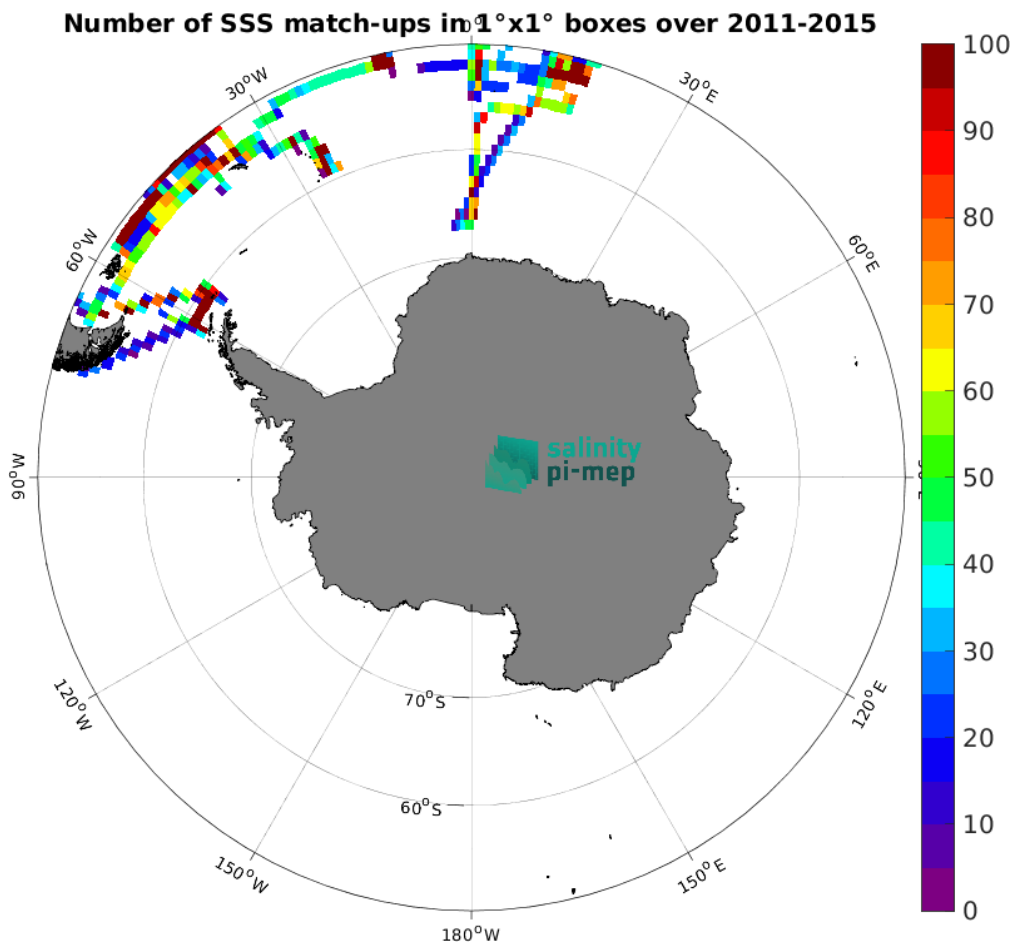
Figure 4: Number of SSS match-ups between TSG (Polarstern) SSS and the Aquarius SSS L3 OR v5 - 7-Day running - Rain mask (NASA-GSFC) SSS product for the Southern Ocean Pi-MEP region over 1^\circ \times 1^\circ boxes and for the full satellite product period.
