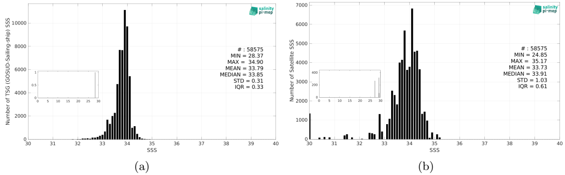
Figure 3: Histograms of SSS from TSG (GOSUD-Sailing-ship) (a) and Aquarius SSS L3 OR v5 - 7-Day running - Rain mask (NASA-GSFC) (b) considering all match-up pairs per bins of 0.1 over the Southern Ocean Pi-MEP region and for the full satellite product period.
