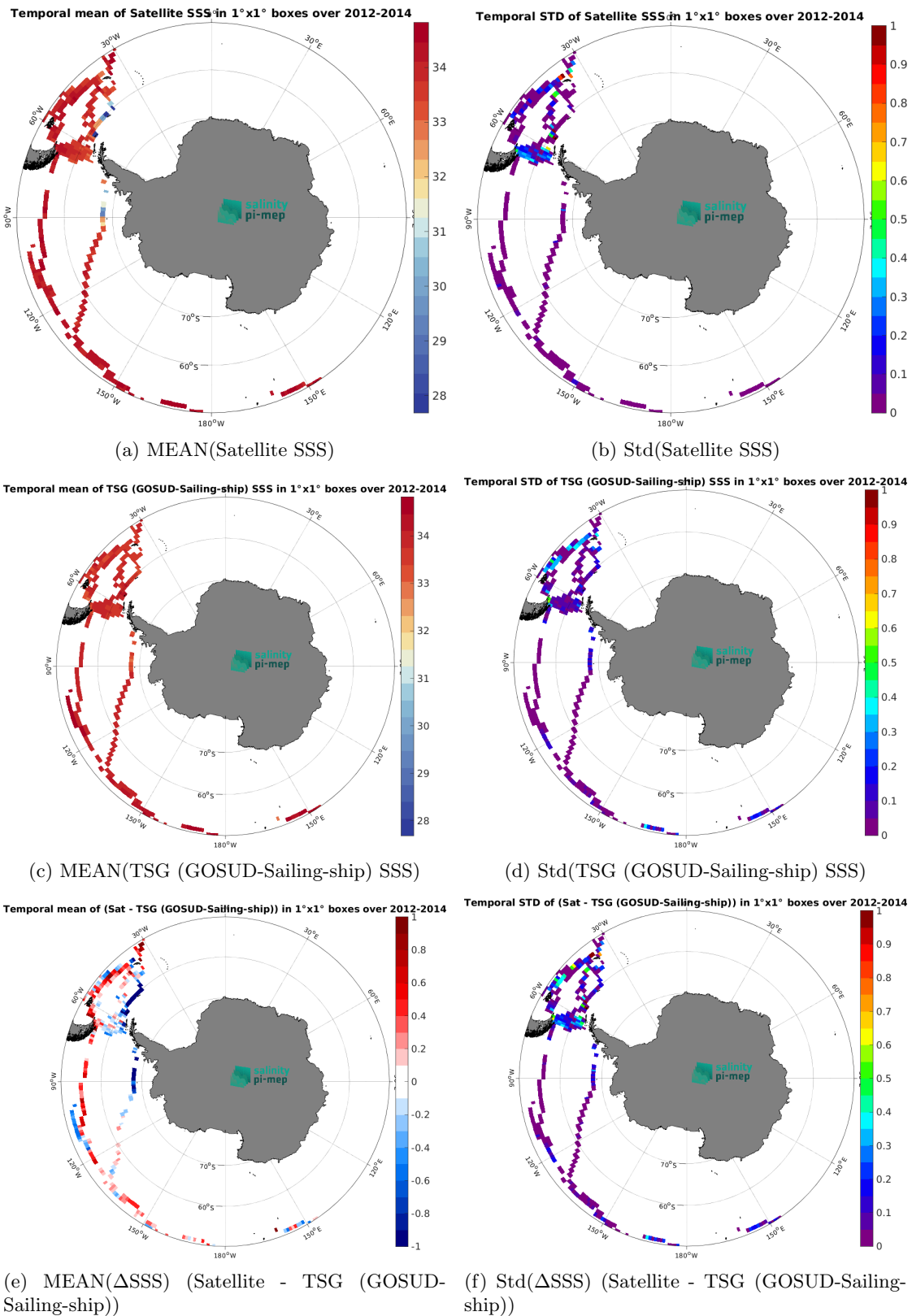
Figure 7: Temporal mean (left) and Std (right) of SSS from Aquarius SSS L3 OR v5 - 7-Day running - Rain mask (NASA-GSFC) (top), TSG (GOSUD-Sailing-ship) (middle), and of \Delta SSS (Satellite - TSG (GOSUD-Sailing-ship)). Only match-up pairs are used to generate these maps.
