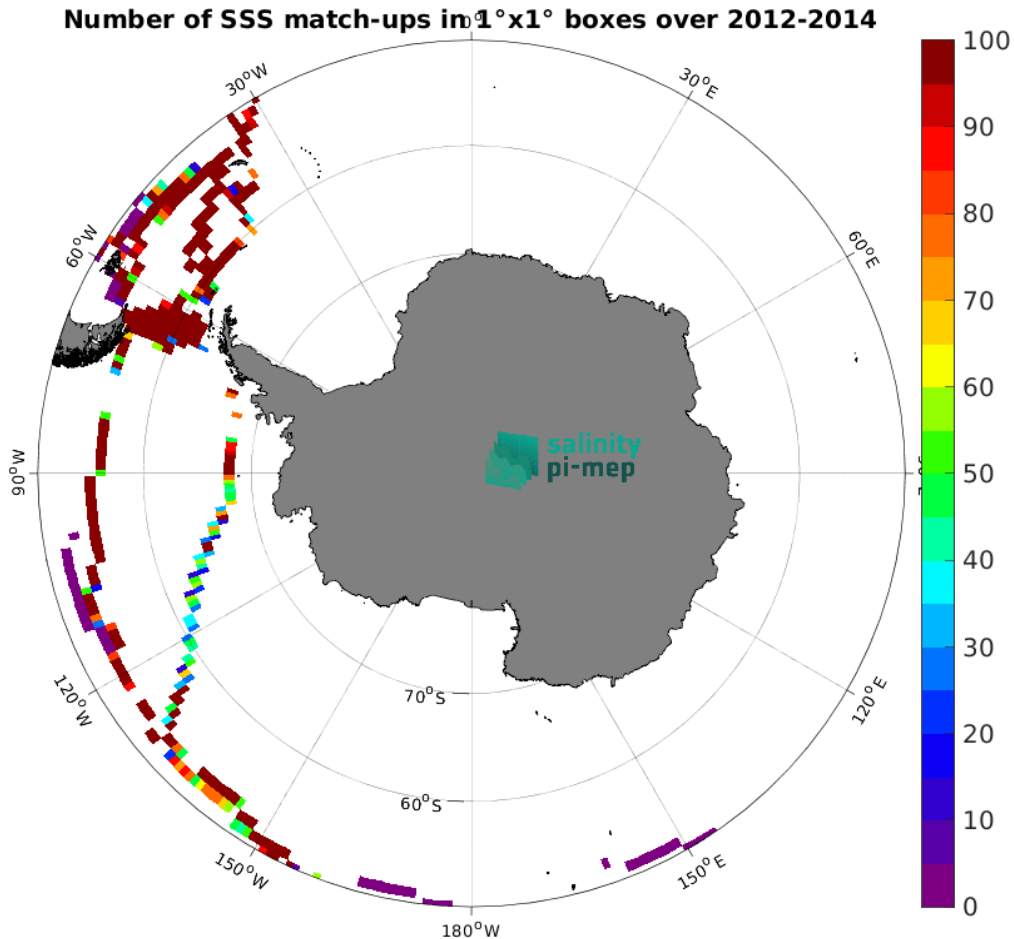
Figure 5: Number of SSS match-ups between TSG (GOSUD-Sailing-ship) SSS and the Aquarius SSS L3 OR v5 - 7-Day running - Rain mask (NASA-GSFC) SSS product for the Southern Ocean Pi-MEP region over 1^\circ \times 1^\circ boxes and for the full satellite product period.
