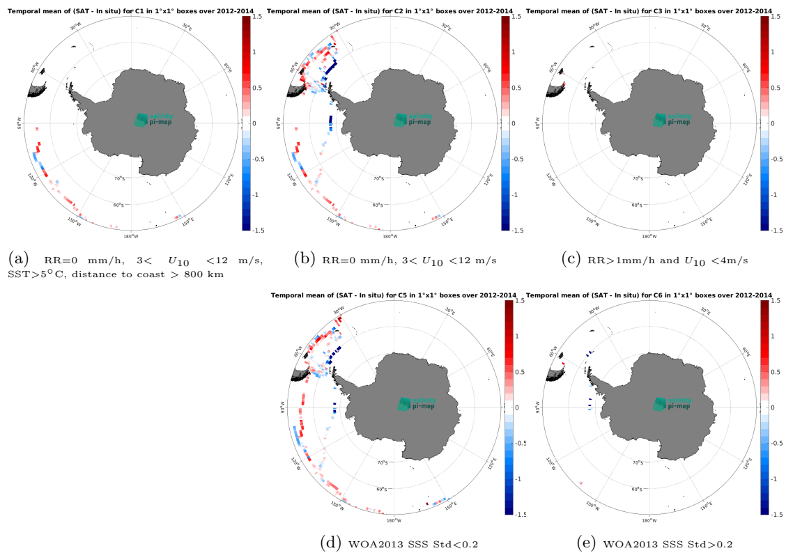
Figure 14: Temporal mean gridded over spatial boxes of size 1^\circ \times 1^\circ of \Delta SSS (Aquarius SSS L3 OR v5 - 7-Day running - Rain mask (NASA-GSFC) - TSG (GOSUD-Sailing-ship)) for 5 different subdatasets corresponding to:RR=0 mm/h, 3 < U_{10} < 12 m/s, SST >5^\circ\text{C} , distance to coast > 800 km (a), RR=0 mm/h, 3 < U_{10} < 12 m/s (b), RR >1 mm/h and U_{10} < 4 m/s (c), WOA2013 SSS Std <0.2 (d), WOA2013 SSS Std >0.2 (e).
