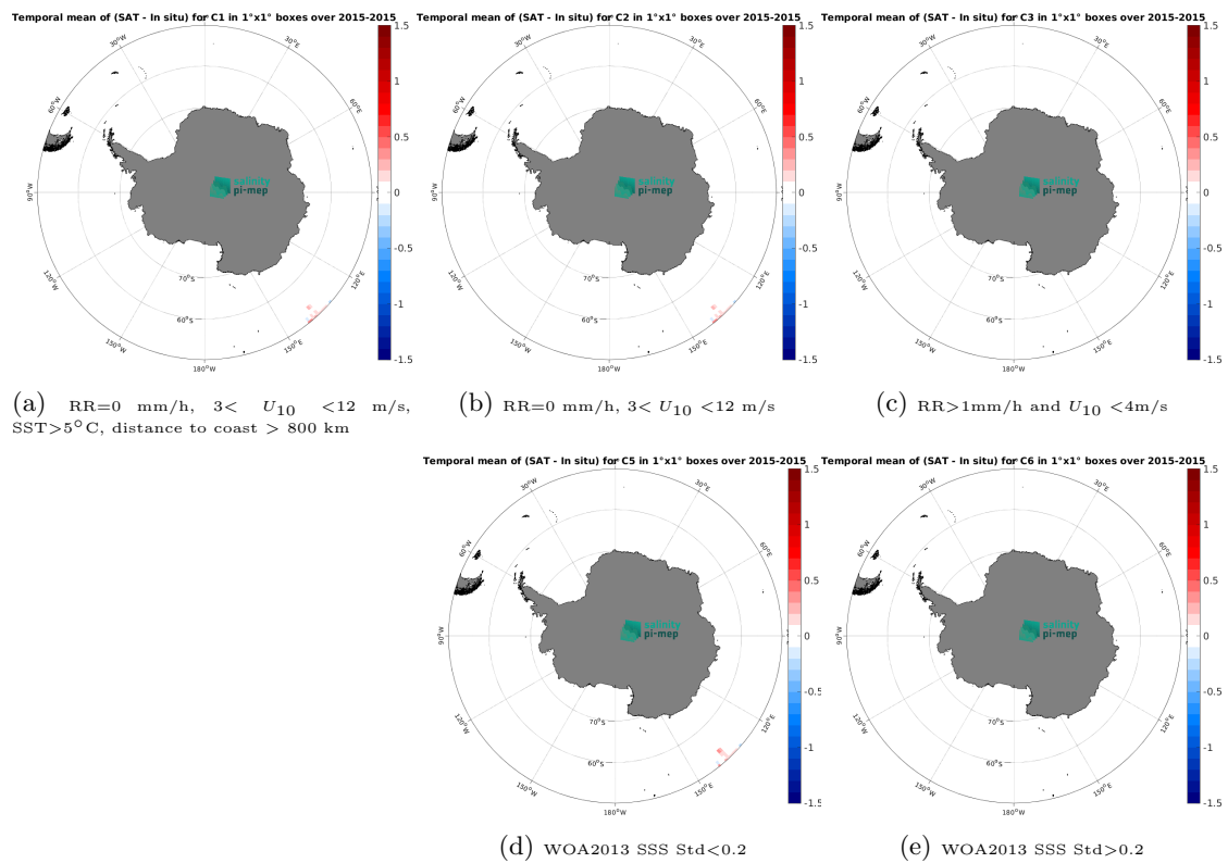
Figure 14: Temporal mean gridded over spatial boxes of size 1^\circ \times 1^\circ of \Delta\text{SSS} (Aquarius SSS L3 OR v5 - 7-Day running - Rain mask (NASA-GSFC) - TSG (GOSUD-Research-vessel)) for 5 different subdatasets corresponding to:RR=0 mm/h, 3 < U_{10} < 12 m/s, SST >5^\circ\text{C} , distance to coast > 800 km (a), RR=0 mm/h, 3 < U_{10} < 12 m/s (b), RR >1 mm/h and U_{10} < 4 m/s (c), WOA2013 SSS Std <0.2 (d), WOA2013 SSS Std >0.2 (e).
