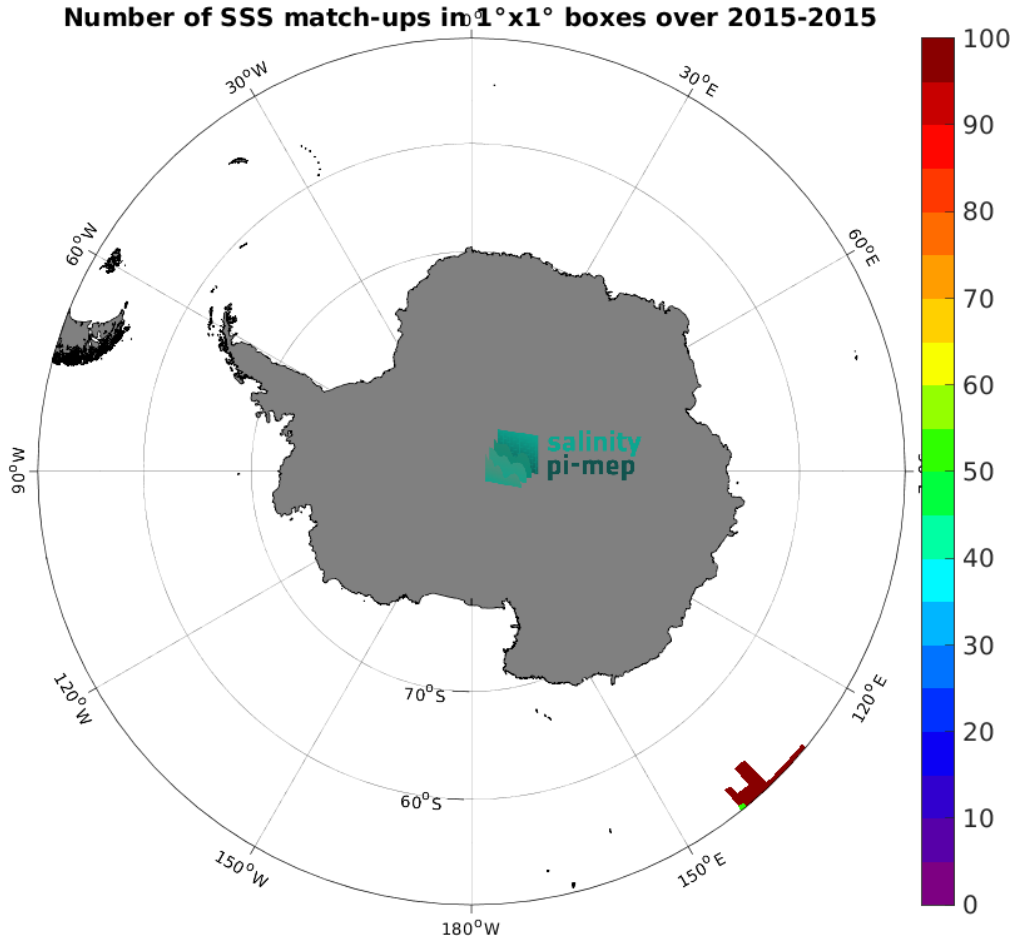
Figure 5: Number of SSS match-ups between TSG (GOSUD-Research-vessel) SSS and the Aquarius SSS L3 OR v5 - 7-Day running - Rain mask (NASA-GSFC) SSS product for the Southern Ocean Pi-MEP region over 1^\circ \times 1^\circ boxes and for the full satellite product period.
