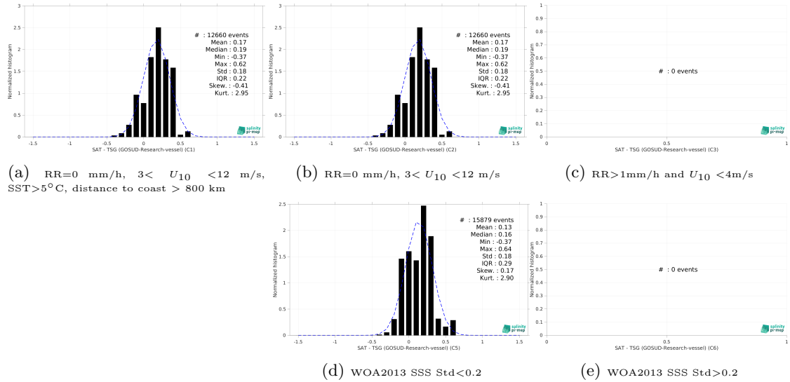
Figure 15: Normalized histogram of \Delta\text{SSS} (Aquarius SSS L3 OR v5 - 7-Day running - Rain mask (NASA-GSFC) - TSG (GOSUD-Research-vessel)) for 5 different subdatasets corresponding to: RR=0 mm/h, 3 < U_{10} < 12 m/s, SST > 5^\circ\text{C} , distance to coast > 800 km (a), RR=0 mm/h, 3 < U_{10} < 12 m/s (b), RR > 1\text{mm/h} and U_{10} < 4\text{m/s} (c), WOA2013 SSS Std < 0.2 (d), WOA2013 SSS Std > 0.2 (e).
