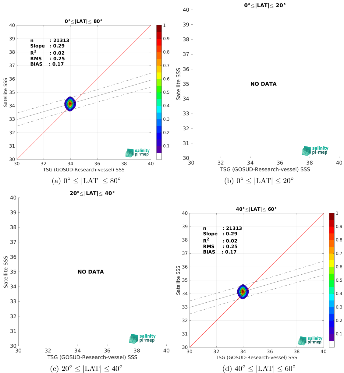
Figure 10: Contour maps of the concentration of Aquarius SSS L3 OR v5 - 7-Day running - Rain mask (NASA-GSFC) SSS (y-axis) versus TSG (GOSUD-Research-vessel) SSS (x-axis) at match-up pairs for different latitude bands. For each plot, the red line shows x=y . The black thin and dashed lines indicate a linear fit through the data cloud and the \pm 95\% confidence levels, respectively. The number match-up pairs n , the slope and R^2 coefficient of the linear fit, the root mean square (RMS) and the mean bias between satellite and in situ data are indicated for each latitude band in each plots.
