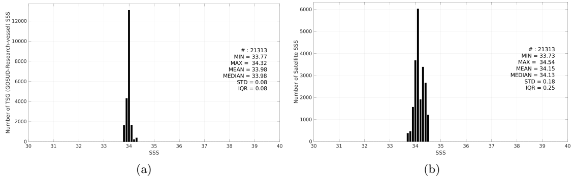
Figure 3: Histograms of SSS from TSG (GOSUD-Research-vessel) (a) and Aquarius SSS L3 OR v5 - 7-Day running - Rain mask (NASA-GSFC) (b) considering all match-up pairs per bins of 0.1 over the Southern Ocean Pi-MEP region and for the full satellite product period.
