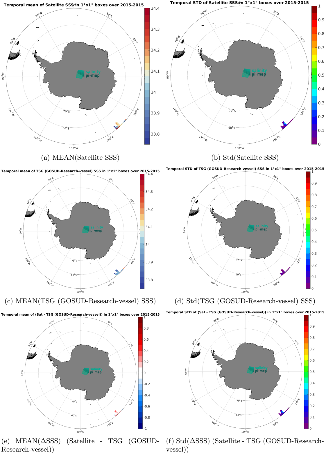
Figure 7: Temporal mean (left) and Std (right) of SSS from Aquarius SSS L3 OR v5 - 7-Day running - Rain mask (NASA-GSFC) (top), TSG (GOSUD-Research-vessel) (middle), and of \Delta SSS (Satellite - TSG (GOSUD-Research-vessel)) (bottom). Only match-up pairs are used to generate these maps.
